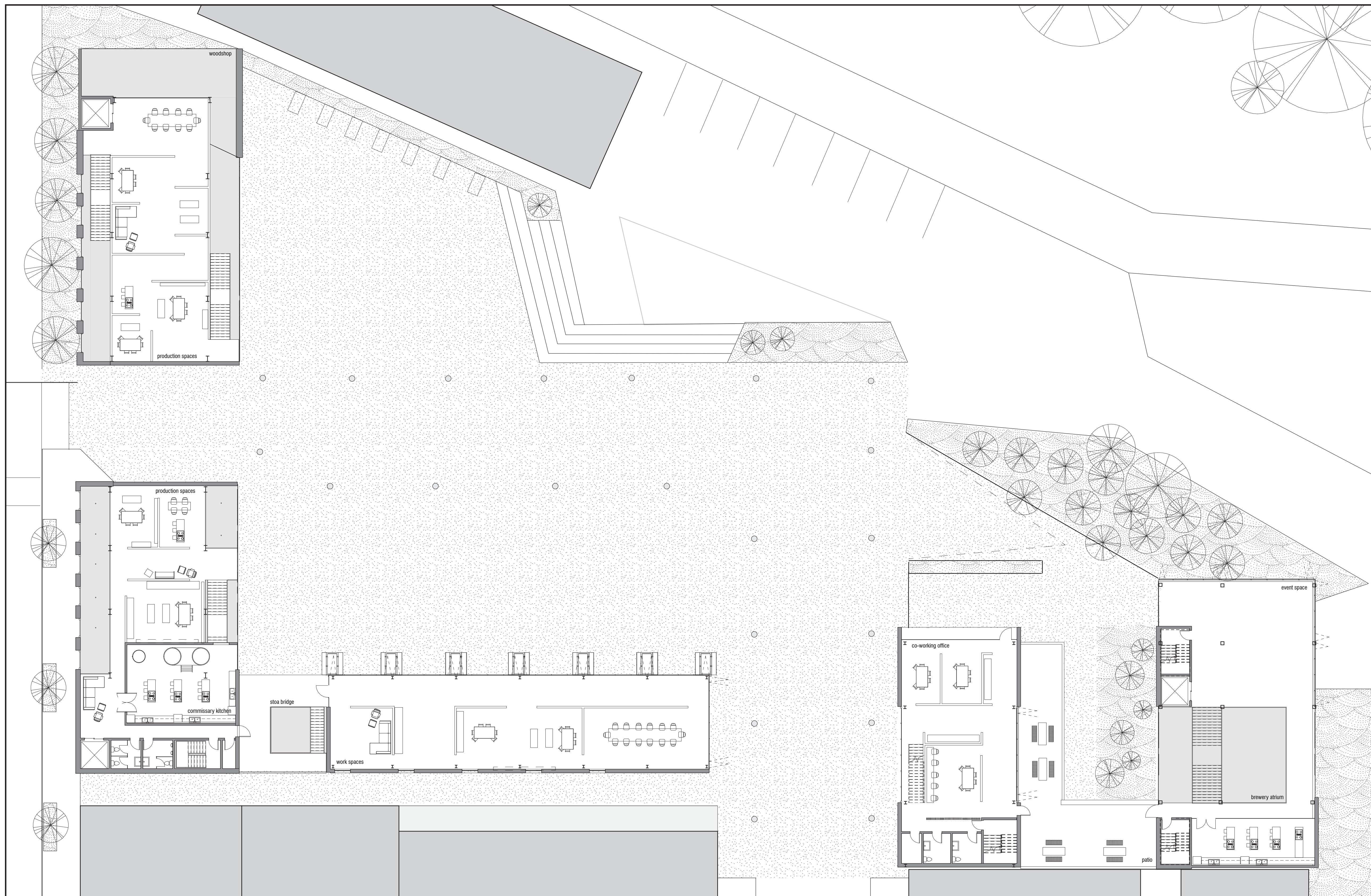
2 1/16 SECOND FLOOR // PLAN
