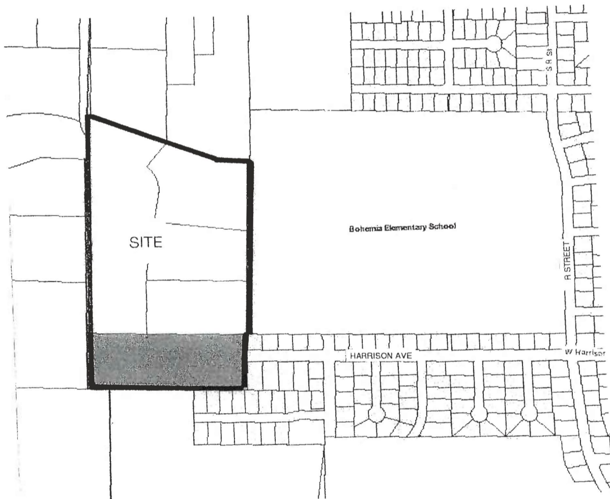
MAP 20 03 32 20 TAX LOTS 100, 200, 800, 900, & 1000
