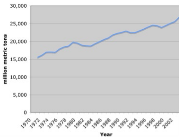
Figure 1-2. Global Carbon Dioxide Emissions, 1970-2003
