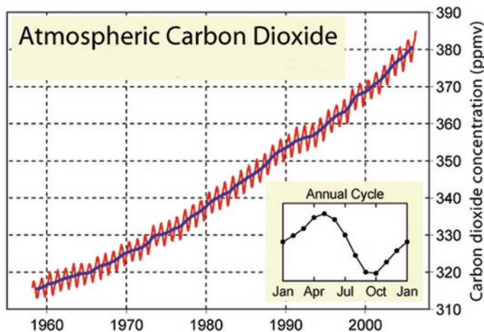
Figure 1-1. The Keeling Curve: Carbon Dioxide Concentrations Measured at Mauna Loa, 1958-2005
