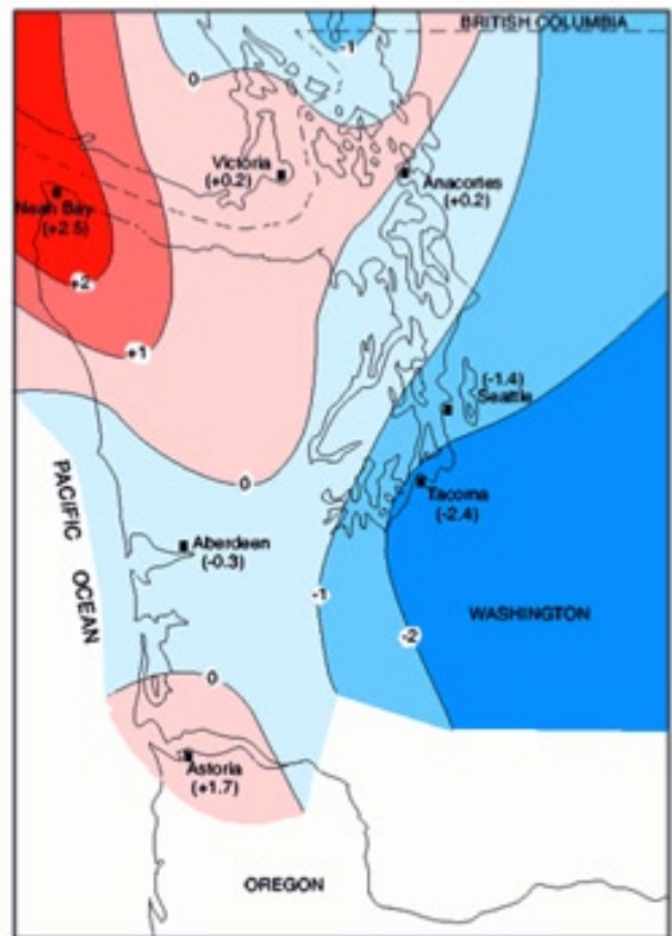
Figure 2-9. Broad Zones of Tectonic Uplift and Subsidence in Western Washington
