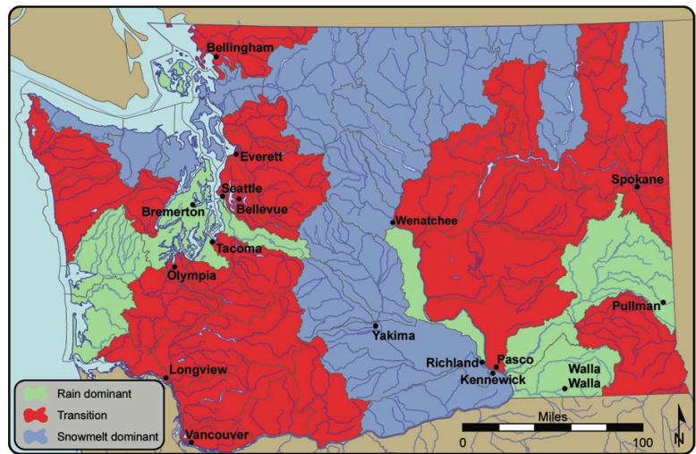
Figure 1-6. Susceptibility of Washington Drainage Basins to Climate Change Impacts on Snowpack
