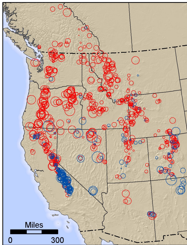
Figure 1-5. Mountain Snowpack Across the West 1950-2000
