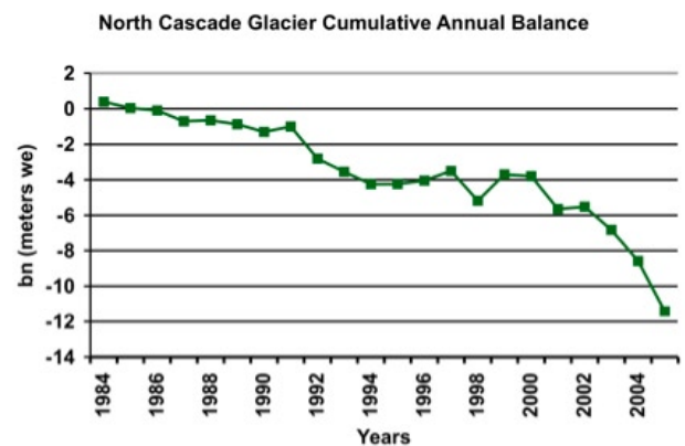
Figure 1-4. Decline of North Cascade Glaciers, 1984-2005
