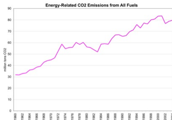
Figure 1-3. Carbon Dioxide Emissions in Washington State, 1960-2004
