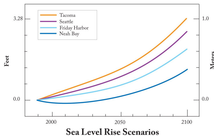
Figure 2-10. Sea Level Rise Anticipated In Several Washington Locations Between the Years 1990 and 2100 Source: Climate Impacts Group.
