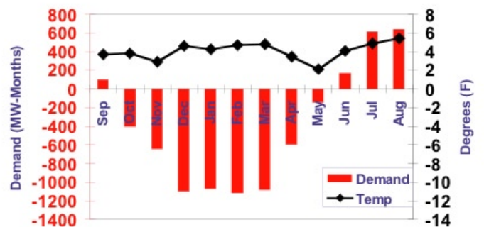
Figure 2-2. Monthly Electricity Demand and Temperature Changes, 2040 Forecast Compared with Historic Baseline
