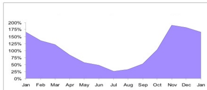
Figure 2-3. Monthly Rainfall in Seattle shows monthly rainfall as a percentage of the annual average
