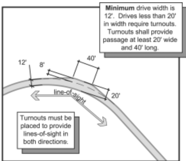
Figure 6 - Minimum construction standards for access: turnout specifications (LCC 935.200).
