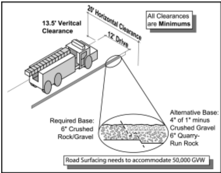
Figure 7 - Minimum construction standards for access: road construction specifications (LCC 935.200).
