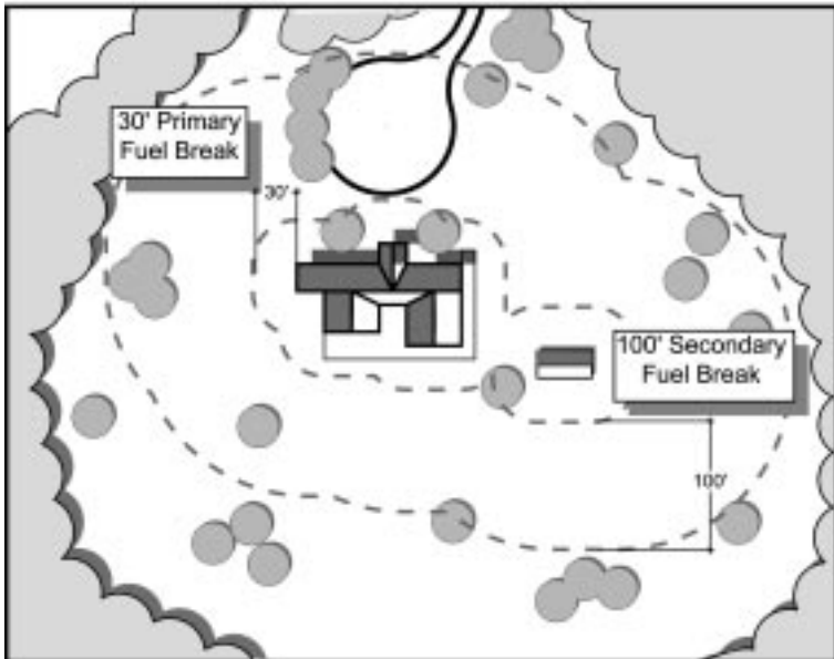
Figure 8 - Primary 30' and secondary 100' fuel-free fire breaks around dwellings in F/F and FCM zoning districts (LCC 934.590).
