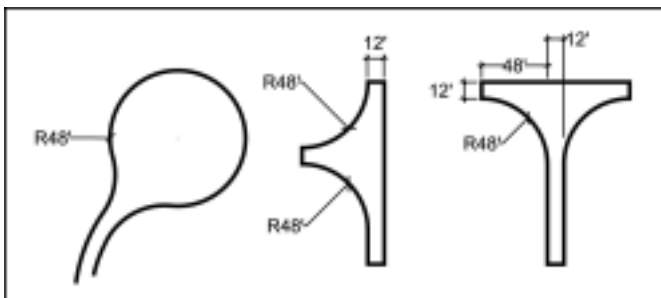
Figure 9 - Acceptable fire apparatus turnaround templates.
