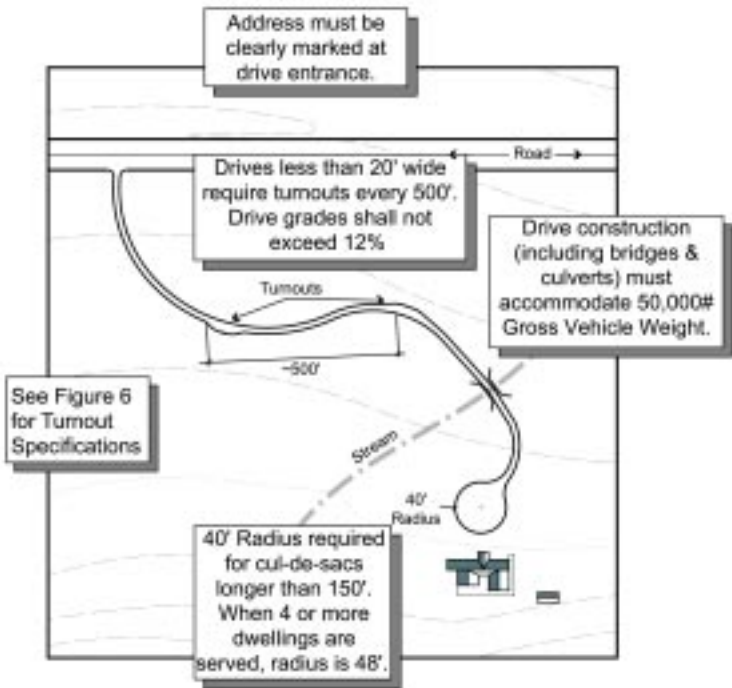
Figure 5 - Minimum construction standards for access (LCC 935.200).
