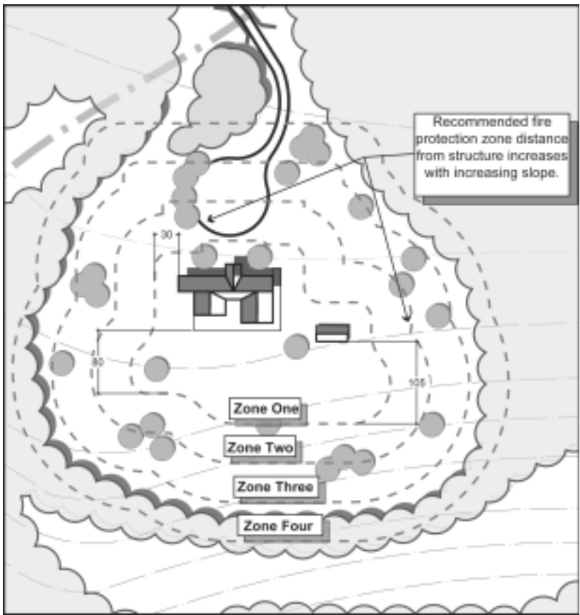
Figure 10 - Fire-wise recommendations for fuel management zones surrounding dwellings (LCC 935.200).
