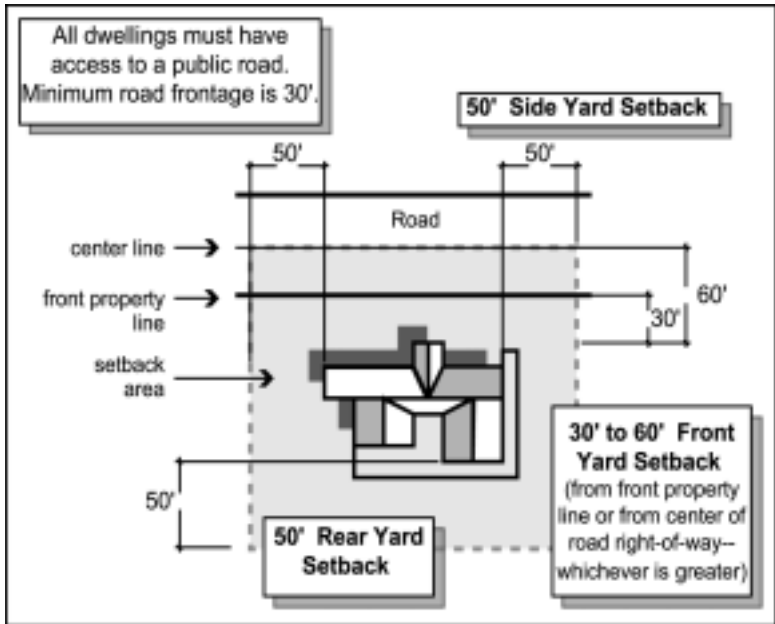
Figure 2 - F/F Structural Setback for front, side, and rear yards (LCC 934.530).
