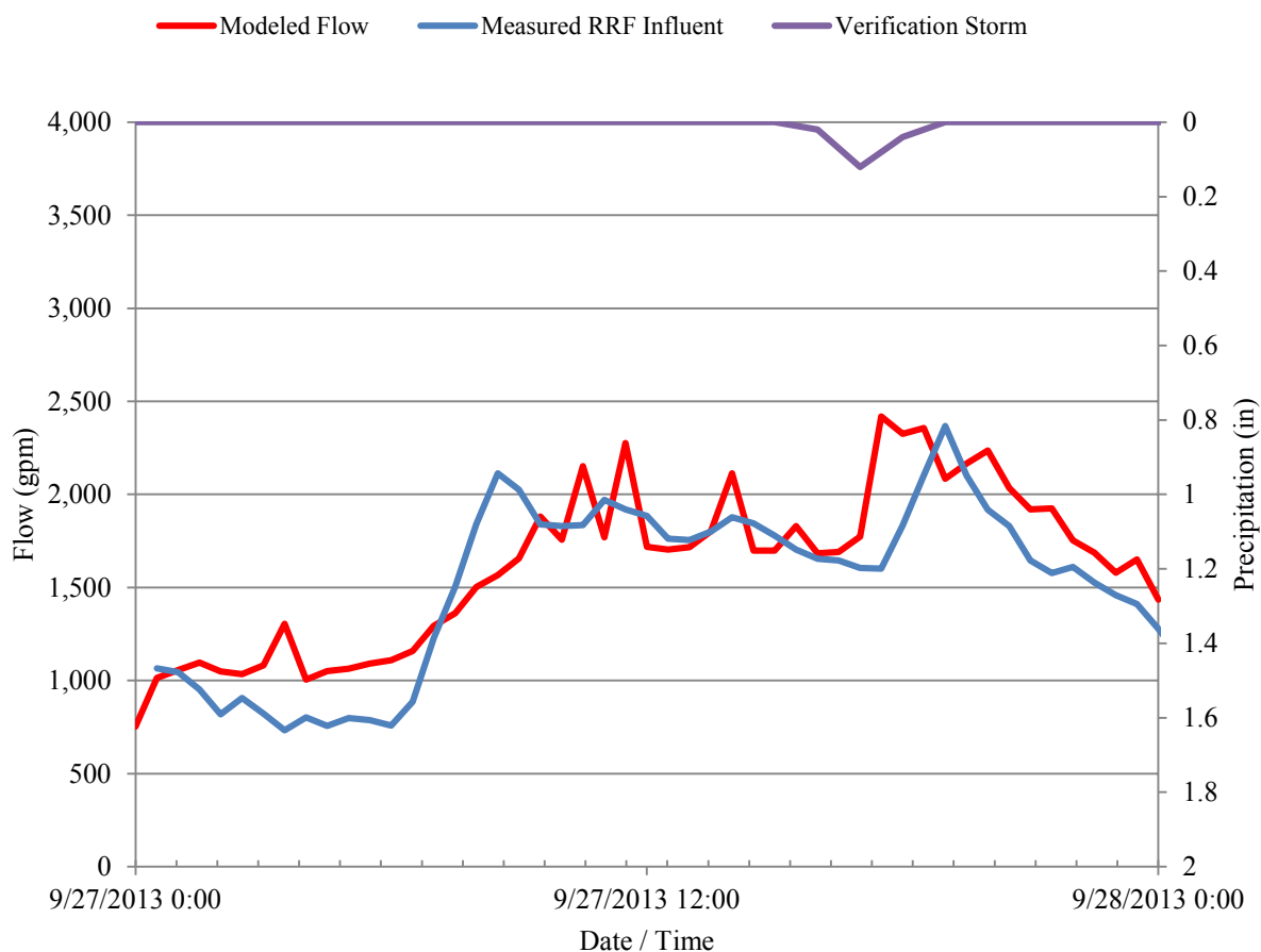
Figure 4-8 Wet Weather Verification Results at the RRF
