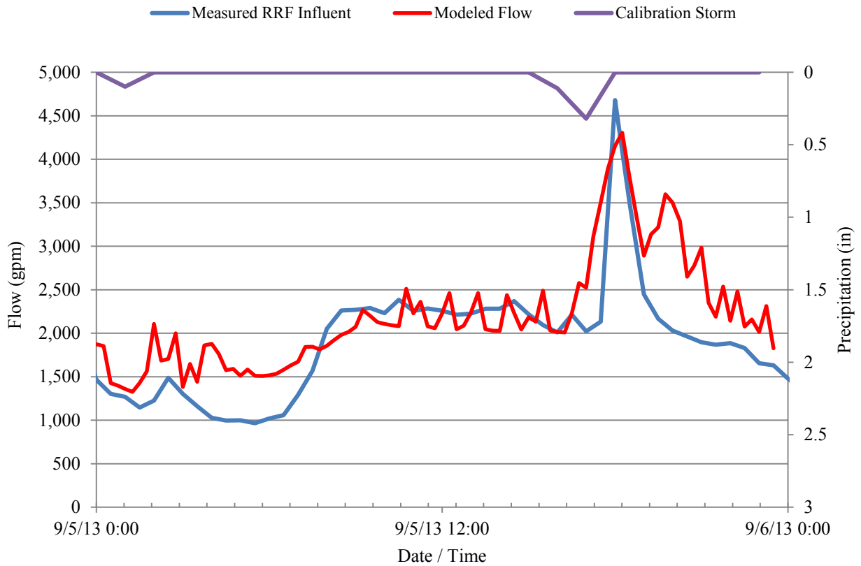
Figure 4-7 Wet Weather Calibration Results at the RRF
