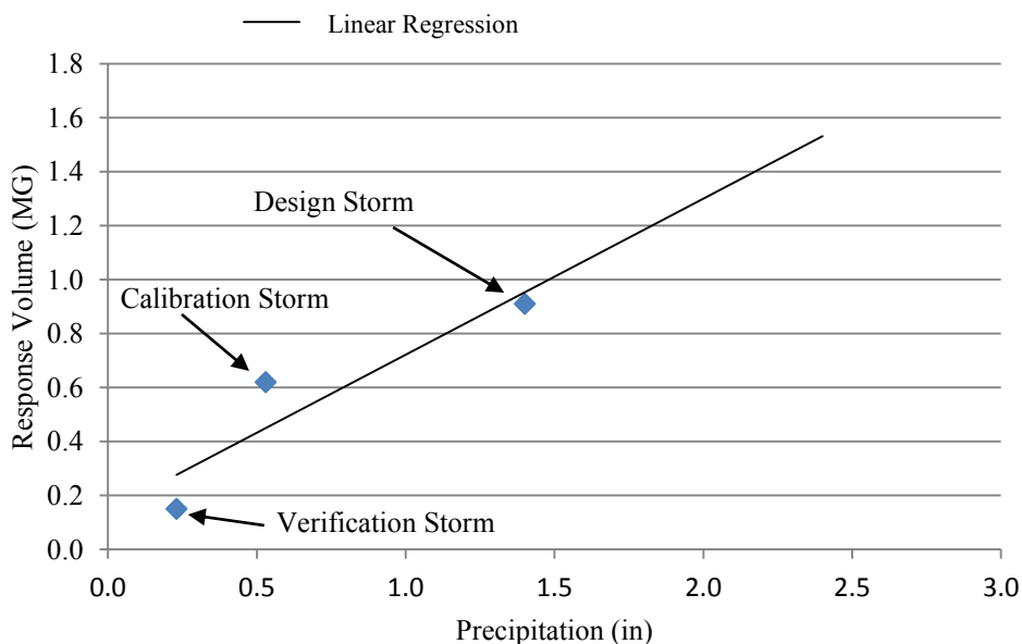
Figure 4-6 RDII Volume and Storm Depth
