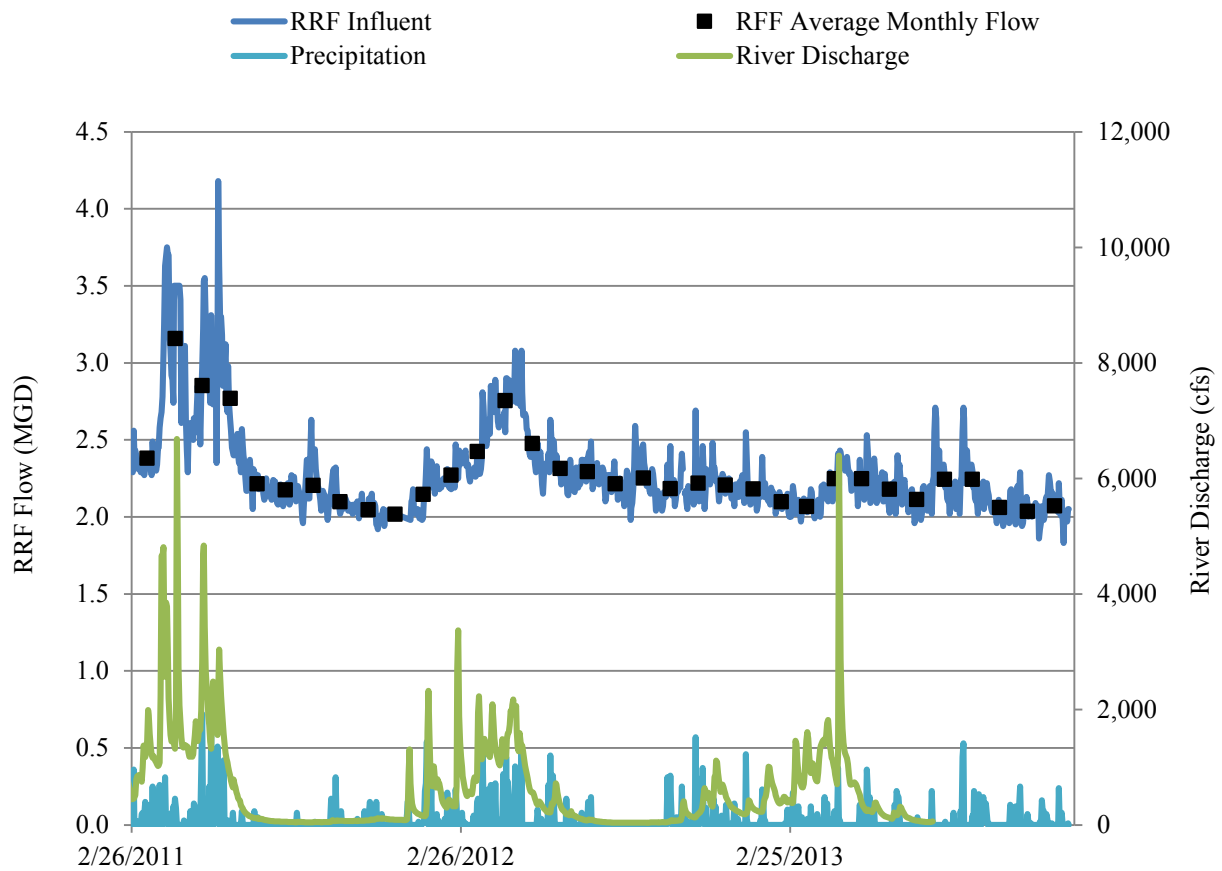
Figure A-1 Sewer Flow Measured at the RRF and Umatilla River Discharge
