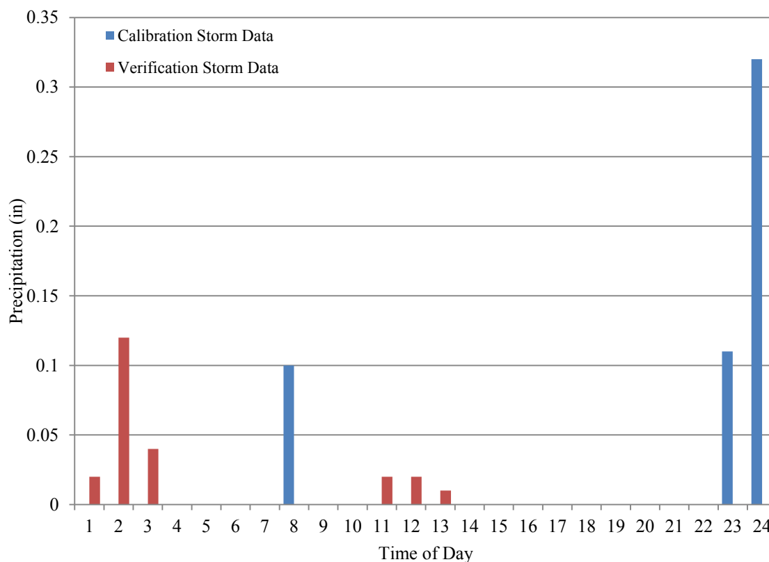
Figure 4-4 Calibration and Verification Storms - Rainfall Distribution
