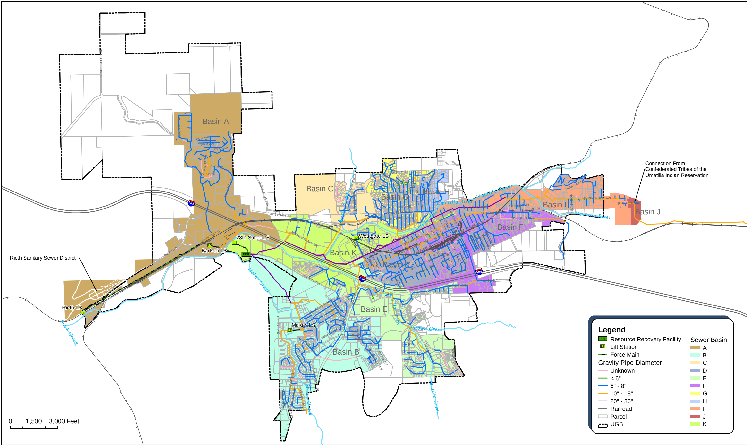
Figure 2-3 Existing Collection System
