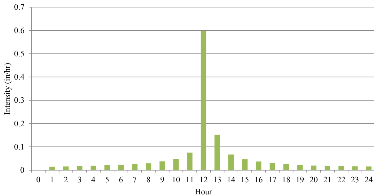
Figure 3-4 City of Pendleton Collection System Design Storm
