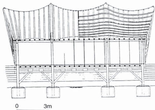
Figure 2—Prototype house, Hooke Park, UK: longitudinal section.
