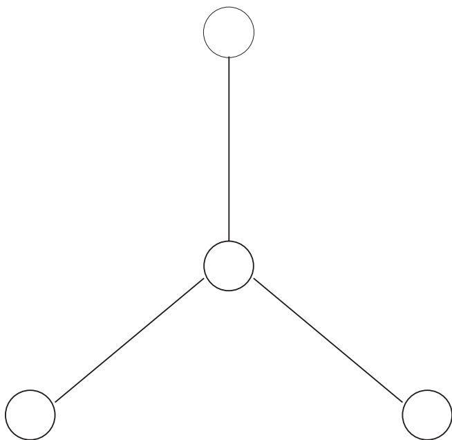
Figure 1 —Aerial view of a pitfall array used to sample sagebrush lizard abundance at Grand Canyon-Parashant National Monument in June 1999, assembled in a peace-sign configuration with drift fence delineated by lines radiating out from the center bucket at 0°, 120°, and 240°, respectively.
