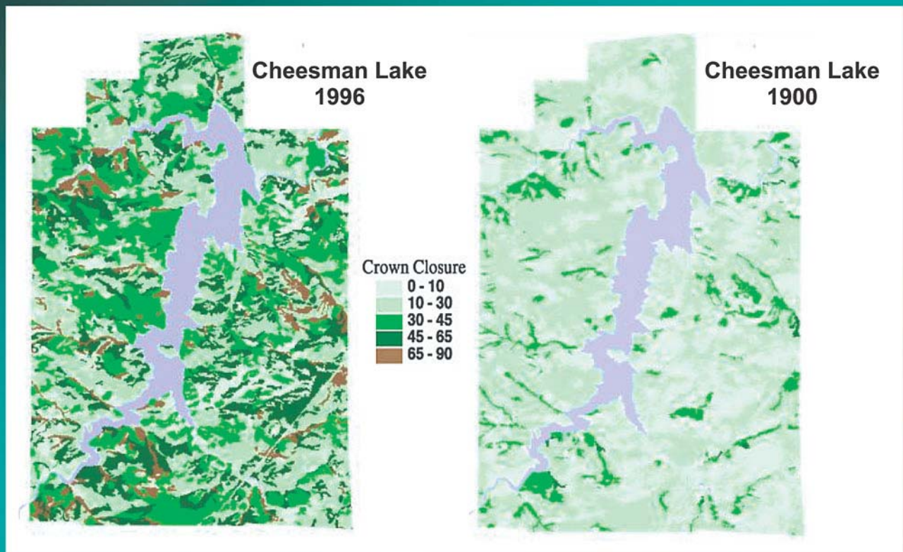
Figure 3 —Crown closure percent for the Cheesman Lake landscape. The 1996 map was developed from 1:6000 color infrared photographs and a patch classification template based on plot data. The 1900 map was developed using the Forest Vegetation Simulator to estimate conditions that, projected forward, yielded conditions observed in 1996.
