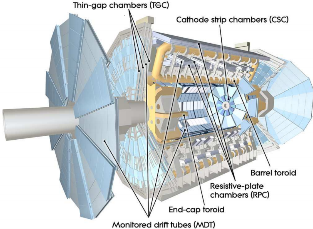
FIGURE 3.17. Schematic of the ATLAS muon detector[38].
