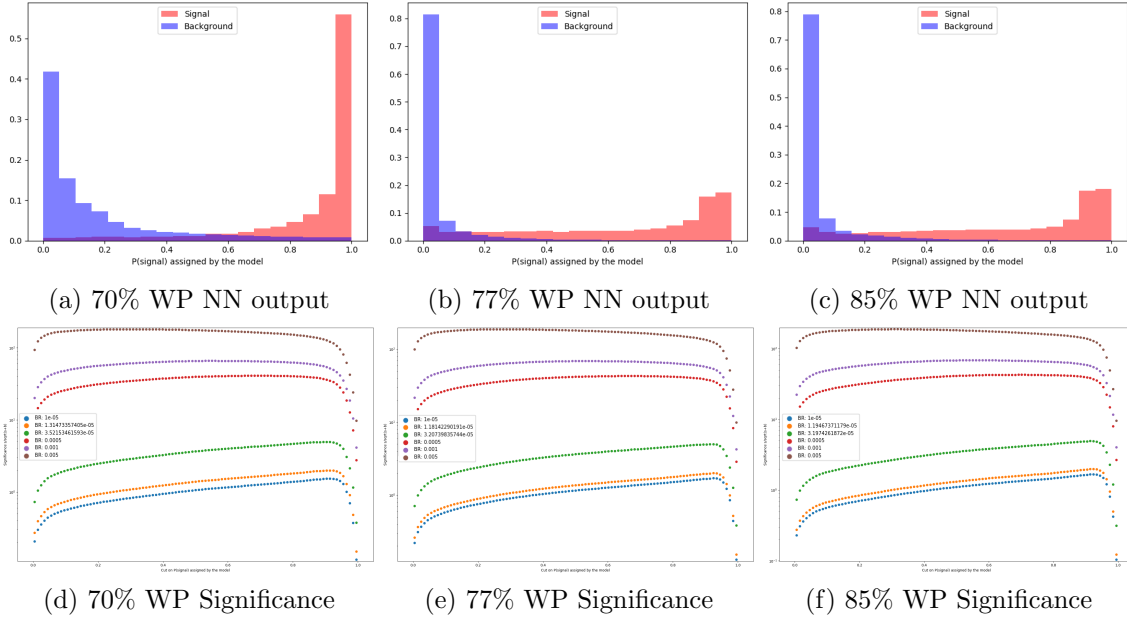
FIGURE 5.13. Neural network output and significance plots for the \mu +jets channel at 70%, 77%, and 85% b-tagging working points.
