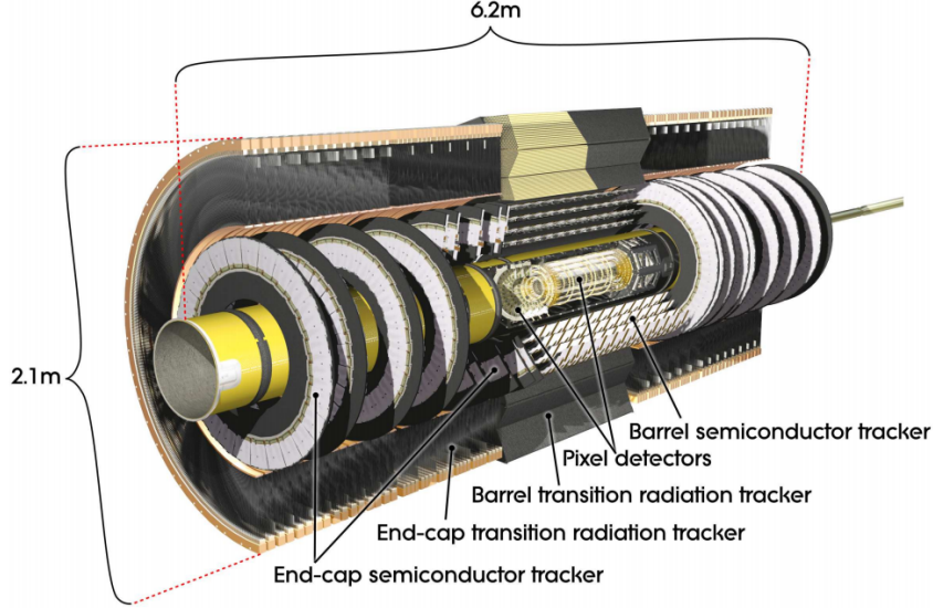
FIGURE 3.10. Schematic of the ATLAS inner detector[38].
