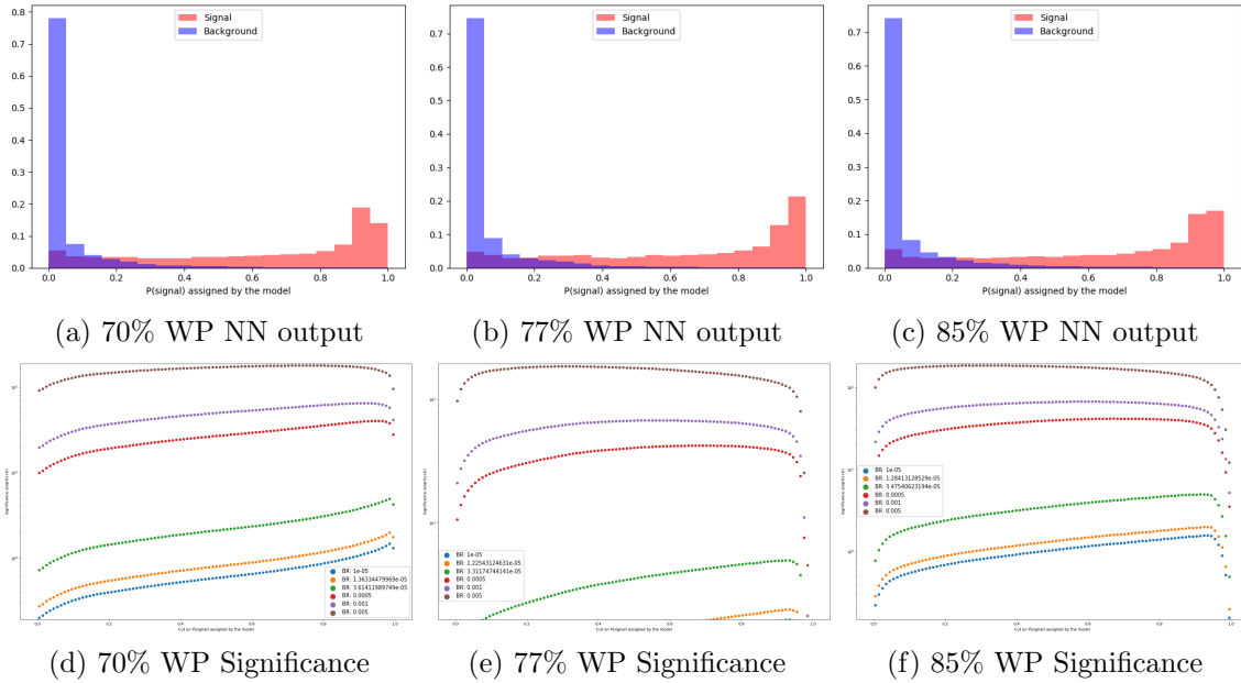
FIGURE 5.12. Neural network output and significance plots for the e +jets channel at 70%, 77%, and 85% b-tagging working points.
