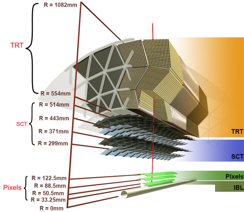
FIGURE 3.12. Blown up schematic of the ATLAS inner detector with more detail[42].
