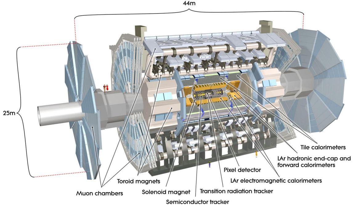
FIGURE 3.7. Schematic of the ATLAS detector[38].
