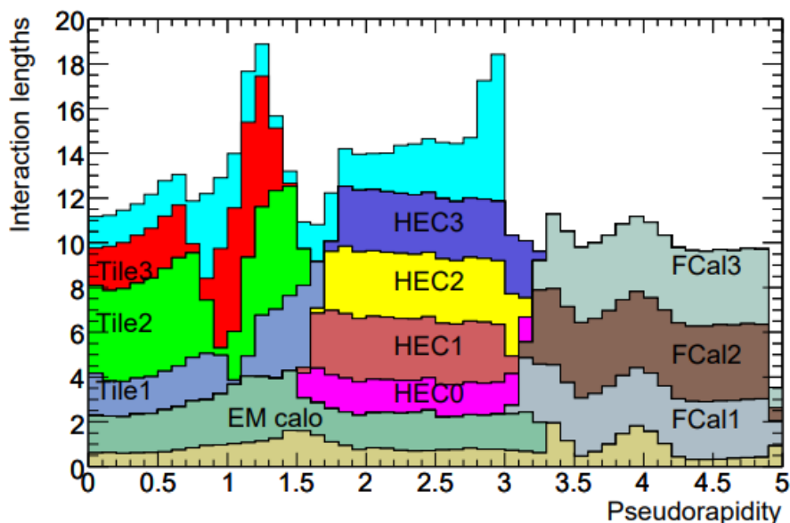
FIGURE 3.16. Number of interaction lengths throughout the LAr calorimeter as a function of |\eta| .
