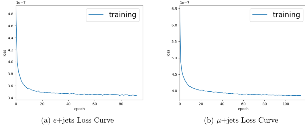
FIGURE 5.7. Loss plots for both channels for the 2 hidden layer neural network.
