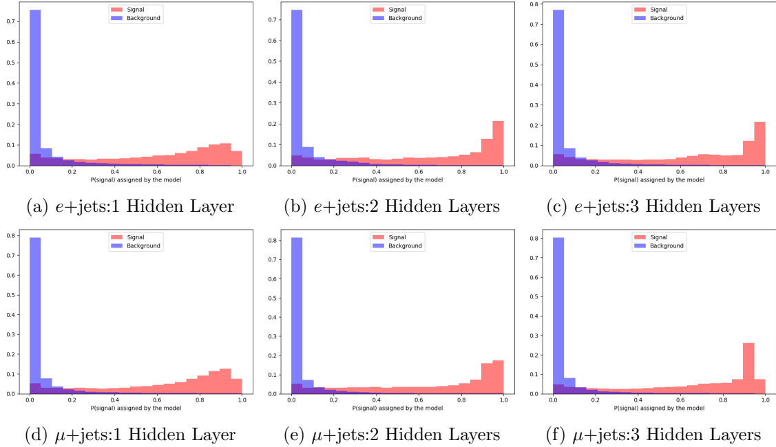
FIGURE 5.8. Normalized neural network output signal and background distribution plots are shown for both search channels for a varying number of hidden layers.
