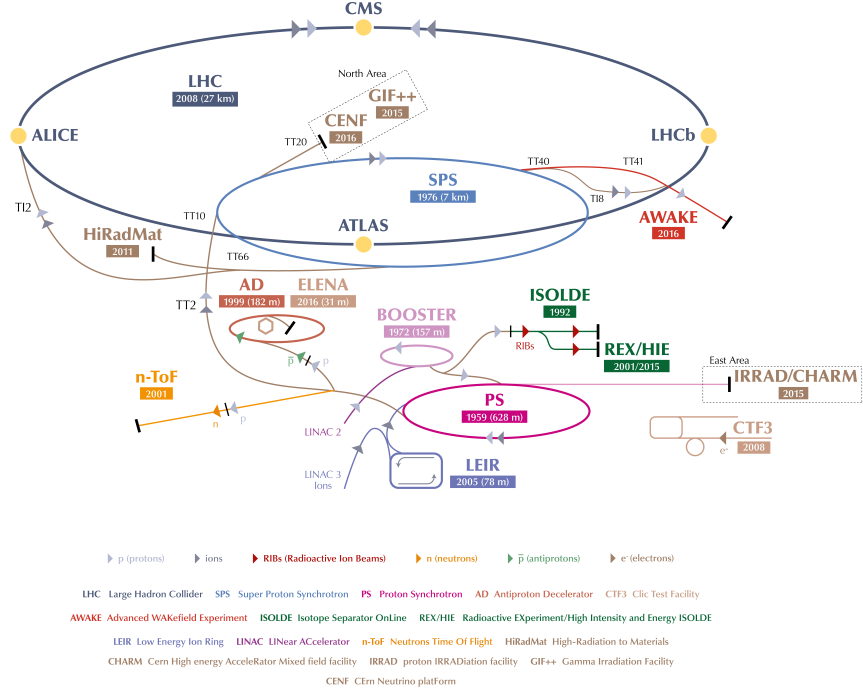
FIGURE 3.2. Schematic of the CERN accelerator complex[36].
