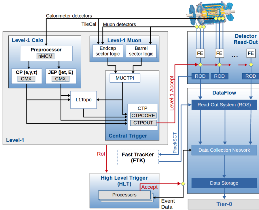
FIGURE 3.18. Flow diagram of the ATLAS trigger and data acquisition system used in Run-2[47].
