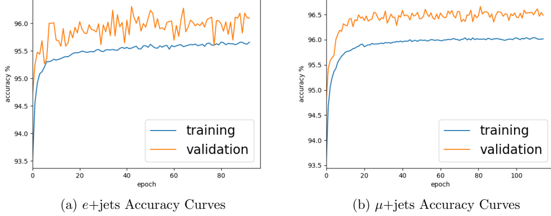
FIGURE 5.6. Accuracy plots for both channels for the 2 hidden layer neural network.
