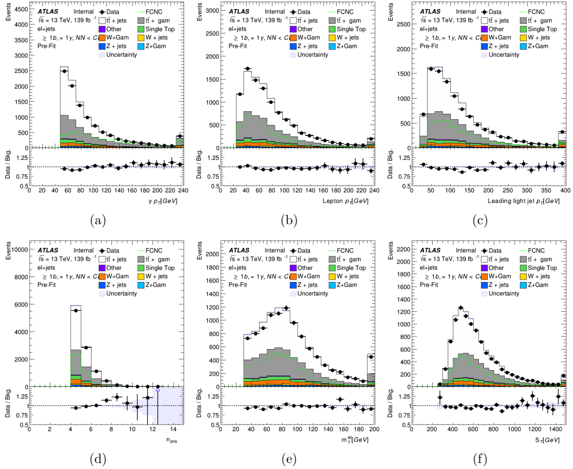
FIGURE 5.30. t\bar{t} + \text{jets} + \gamma validation region plots for the electron channel after all scale factors are applied. The FCNC signal sample is scaled to 1%.
