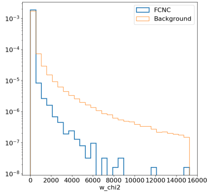
(e) \chi_W^2
