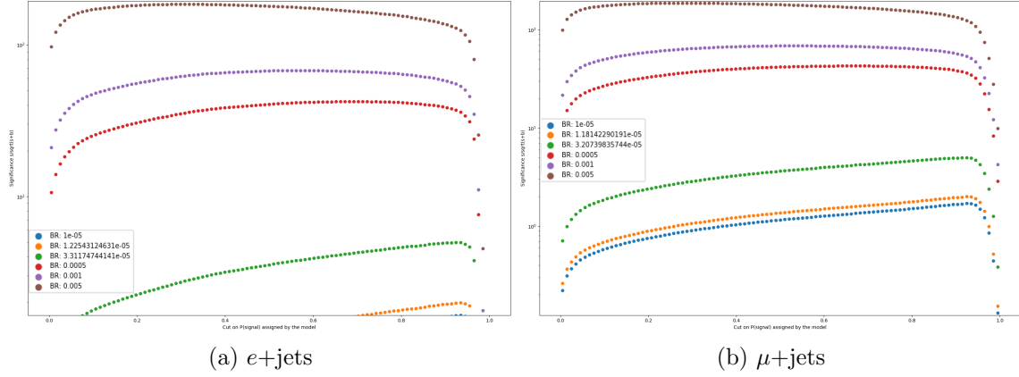
FIGURE 5.9. Significance plots for both channels for the two hidden layer neural network. The green points correspond to a branching ratio with a maximum significance of 5, and the orange to a maximum significance of 2. The e +jets ( \mu +jets) branching ratio with max significance of 2 is 1.22 \times 10^{-5} ( 1.18 \times 10^{-5} ). The blue, red, purple, and brown points correspond to branching ratios of 1 \times 10^{-5} , 5 \times 10^{-4} , 1 \times 10^{-3} , and 5 \times 10^{-3} , respectively.
