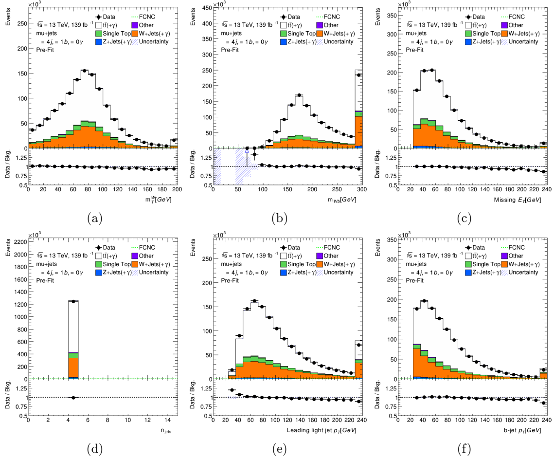
FIGURE 5.22. Event-level plots for the =4 jet validation region after scale factors have been applied in the muon channel. FCNC signal branching ratio is scaled to 0.1%.
