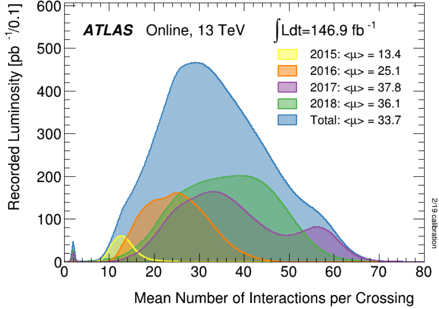
FIGURE 3.4. Luminosity-weighted distribution of the mean number of interactions per bunch crossing for the entirety of Run-2 shown by individual years, 2015 (yellow), 2016 (orange), 2017 (purple), 2018 (green), as well as an integrated total (blue)[37].
