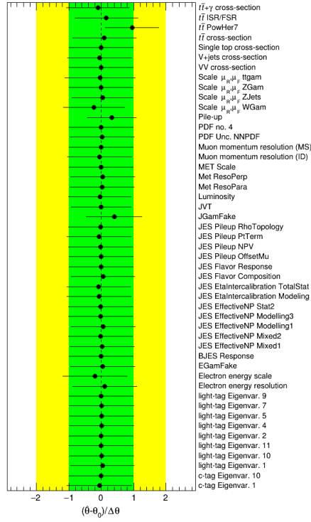
FIGURE 6.7. Pull values for the various nuisance parameters considered in the fit for the \mu +jets channel.
