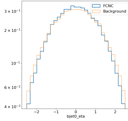
(b) \eta_b
