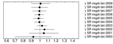
FIGURE 6.3. Bin by bin normalization \gamma factors used in each region for the e +jets channel.
