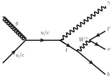
FIGURE 2.14. FCNC diagram for the search in single top production with the ATLAS detector[34].
