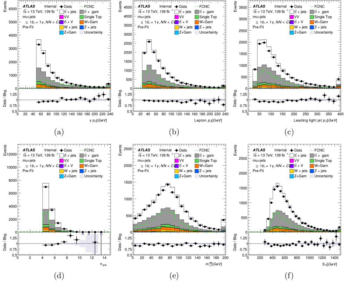
FIGURE 5.31. t\bar{t} +jets+ \gamma validation region plots for the muon channel after all scale factors are applied. The FCNC signal sample is scaled to 1%.
