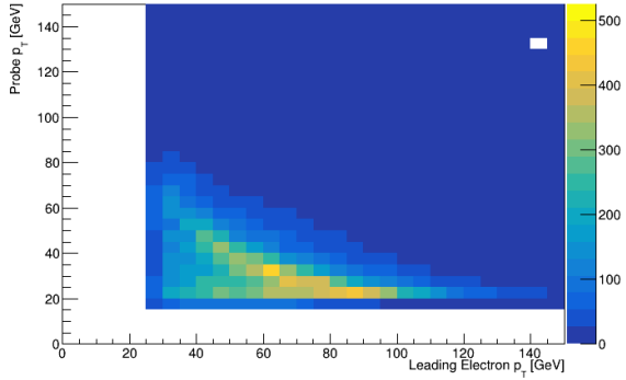
(c) Probe: Unconverted Photons
