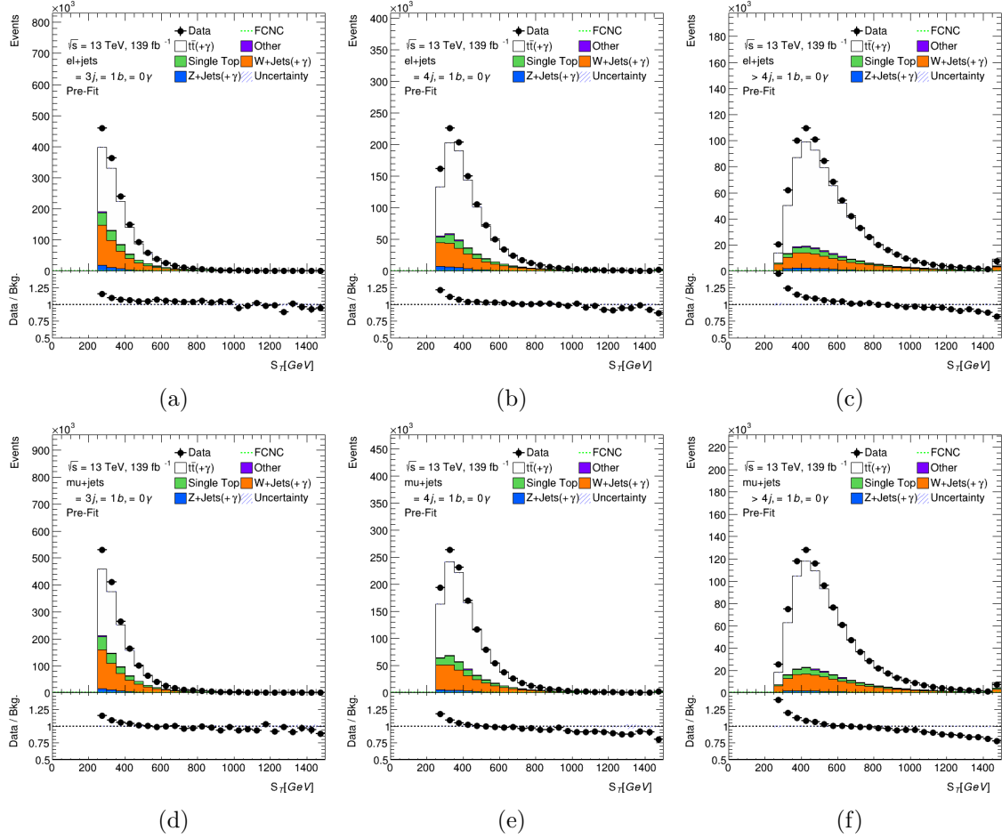
FIGURE 5.20. S_T distributions in the 3 (a, d), 4 (b, e), and 5+ (c, f) jets control and validation regions. The electron channel is shown on the top and the muon channel on the bottom, before scale factors are determined.
