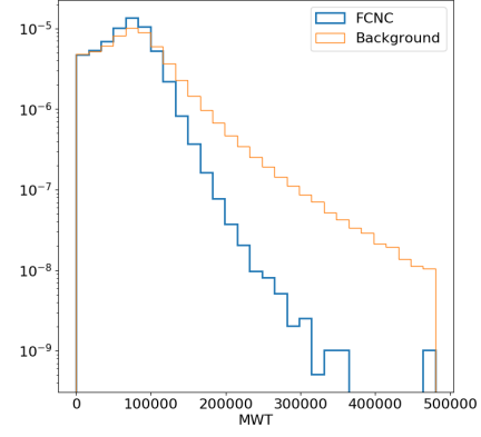
(b) m_T^W
