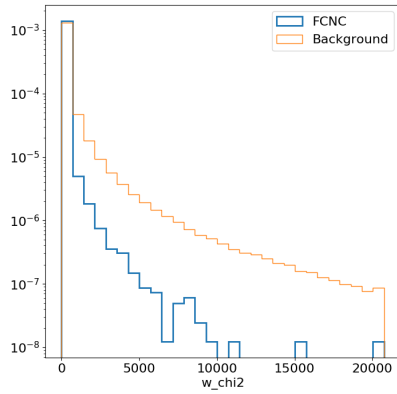
(e) \chi_W^2
