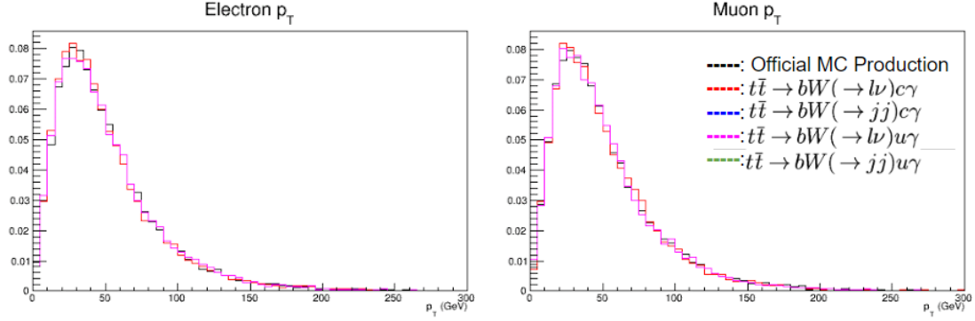
FIGURE 4.5. Normalized p_T of the electron and muons produced by the model for each FCNC final state search and an official t\bar{t} sample.
