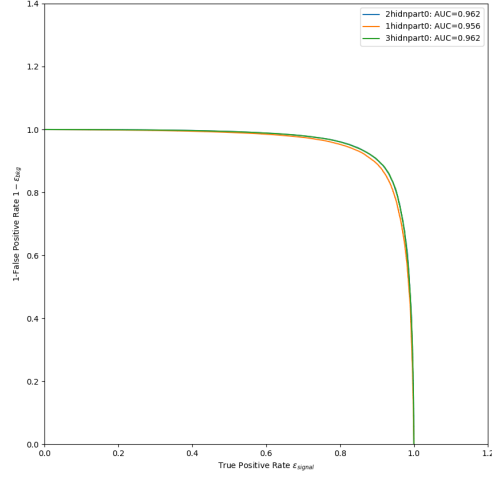
(b) \mu +jets ROC Curves
