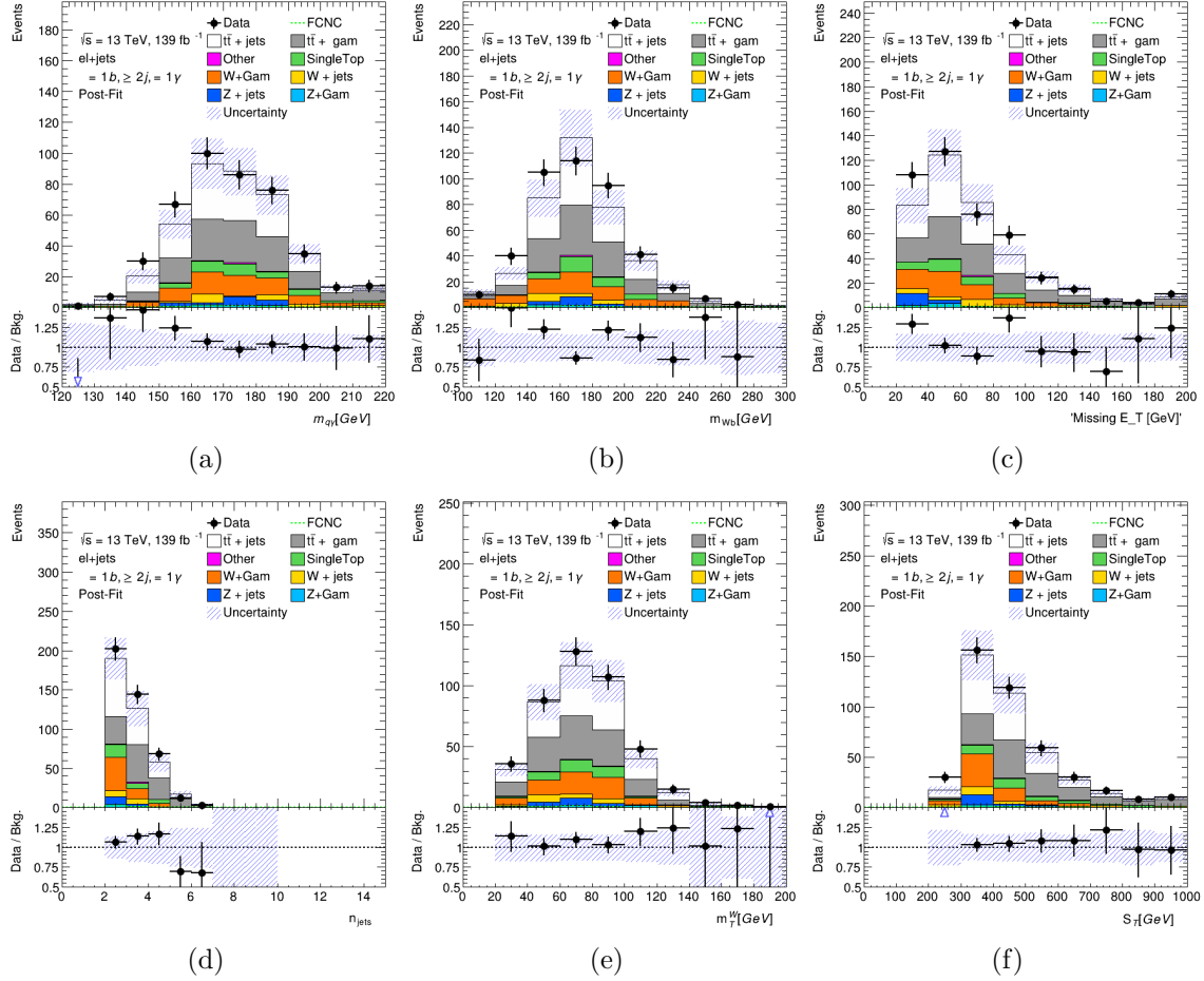
FIGURE G.7. Post-fit distributions for FCNC top candidate mass (a), Standard Model top candidate mass (b), \cancel{E}_T (c), N_{\text{jets}} (d), m_T^W (e), and S_T (f) in the final signal region for the electron channel fitting on \gamma p_T .
