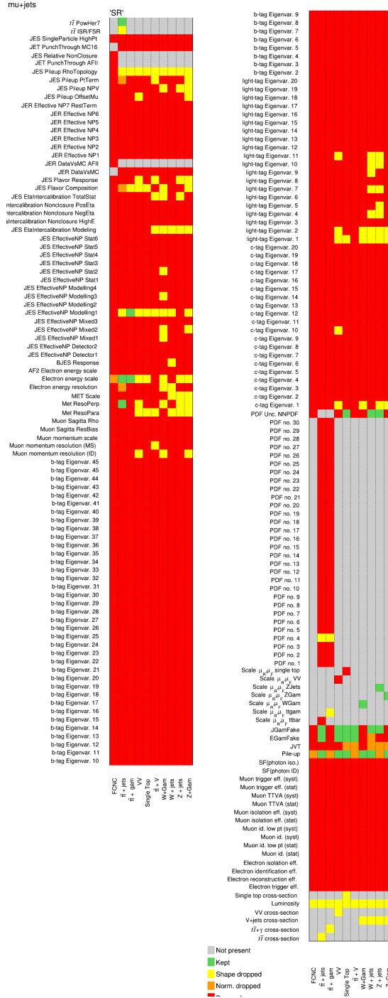
FIGURE 6.6. Overview of nuisance parameters after pruning for the \mu +jets channel. If shape or normalization impacts are smaller than 1% that part of the nuisance parameter will be dropped in the final fit.
