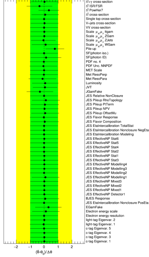
FIGURE 6.2. Pull values for the various nuisance parameters considered in the fit for the e +jets channel.
