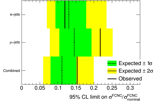
FIGURE G.3. Limits on the signal strength \mu for the alternative fit using m_{q\gamma} in both regions.
