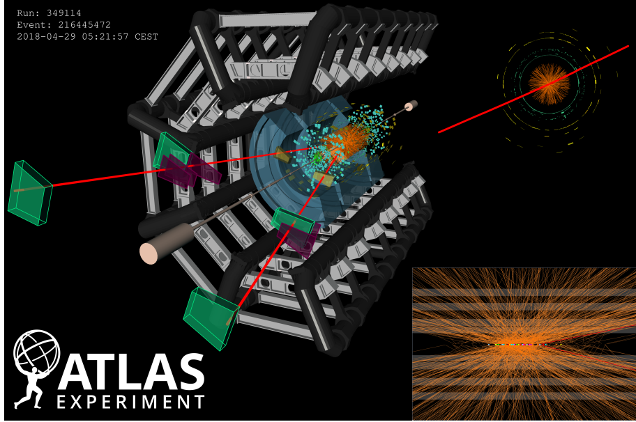
FIGURE 3.5. A candidate dimuon event ( Z \rightarrow \mu^+ \mu^- ) with 28 reconstructed vertices collected in 2018 with the ATLAS detector[37].
