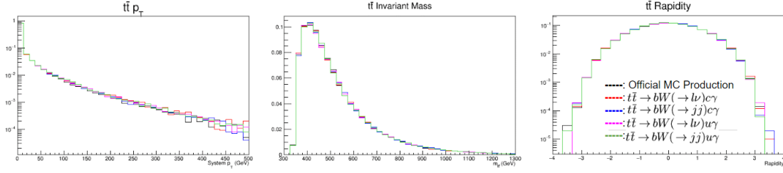
FIGURE 4.4. Normalized kinematics ( p_T , m_{t\bar{t}} , and y_{t\bar{t}} ) of the t\bar{t} system produced by the model for each FCNC final state search and an official t\bar{t} sample.
