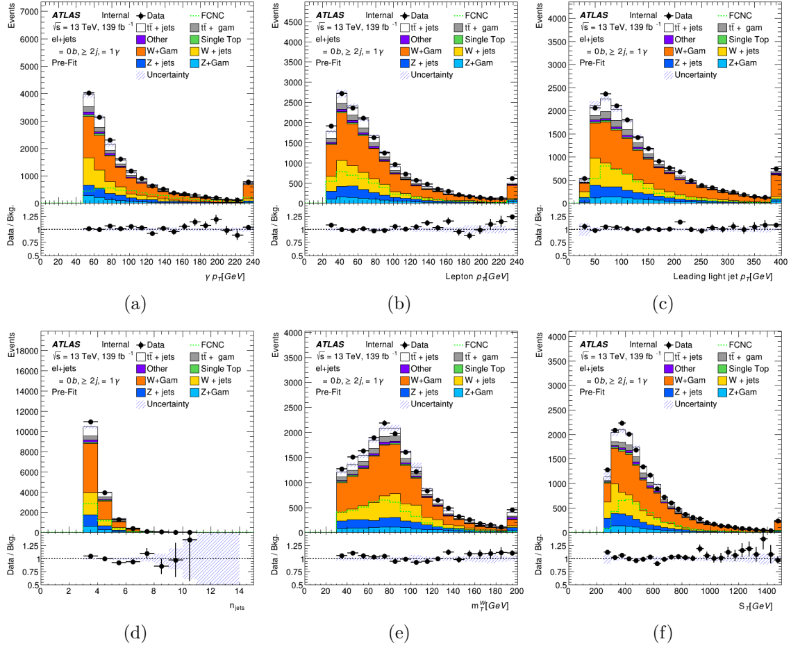
FIGURE 5.28. W+jets+ \gamma validation region plots for the electron channel after all scale factors are applied. The FCNC signal sample is scaled to 1%.
