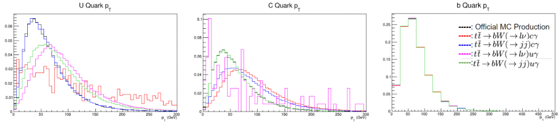
FIGURE 4.6. Normalized p_T of the up, charm, and bottom quarks produced by the model for each FCNC final state search and an official t\bar{t} sample.
