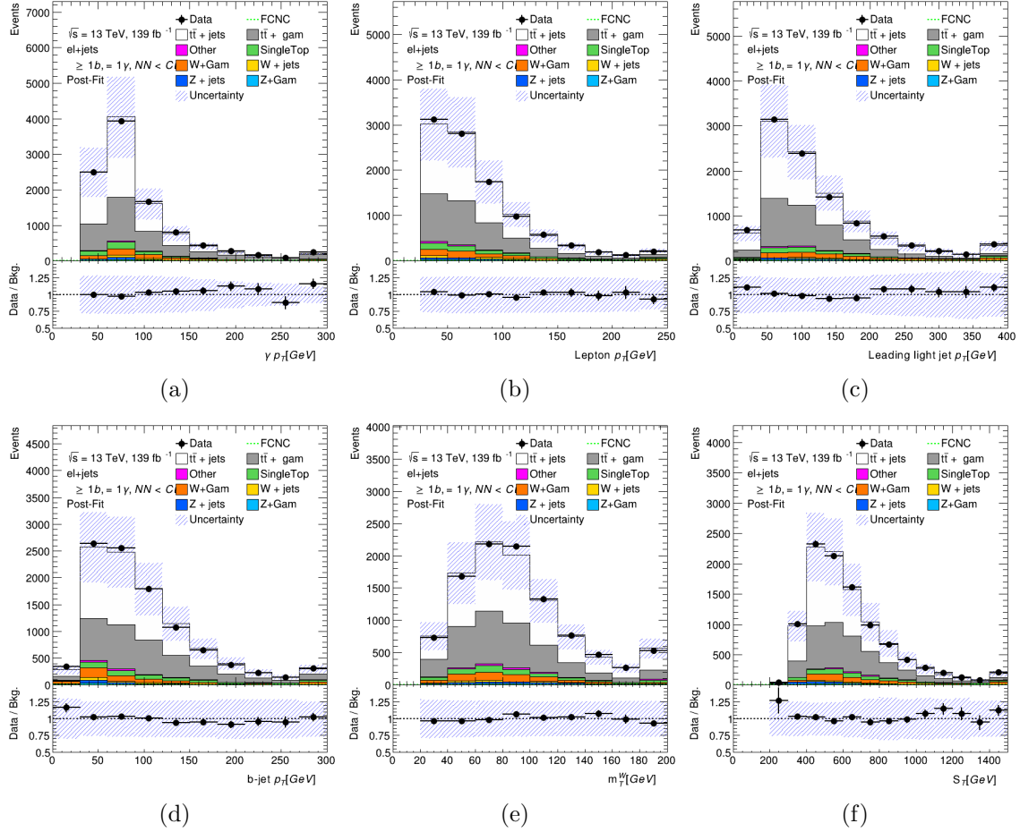
FIGURE G.10. Post-fit distributions for Photon p_T (a), lepton p_T (b), leading light jet p_T (c), leading b-jet p_T (d), m_T^W (e), and S_T (f) in the t\bar{t} + \text{jets} + \gamma validation region for the e + \text{jets} channel for alternative fit using \gamma p_T in both regions.
