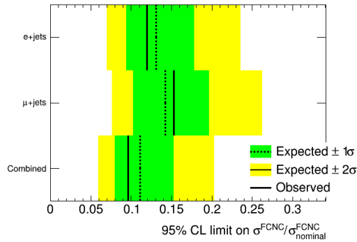
FIGURE 6.15. 95% confidence level upper limits on the signal strength \mu .
