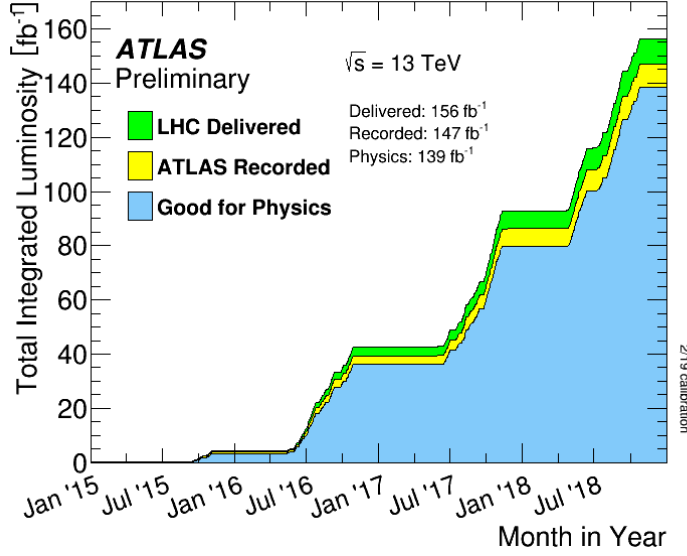
FIGURE 3.3. Total integrated luminosity as a function of time delivered by the LHC (green), recorded (yellow) and declared good for physics analysis (blue) by the ATLAS detector throughout Run-2 consisting entirely of 13 TeV pp collisions[37].
