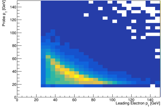
(b) Probe: Converted Photons
