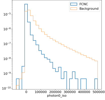
(a) \gamma_{iso} topo E_{T\text{cone}40}
