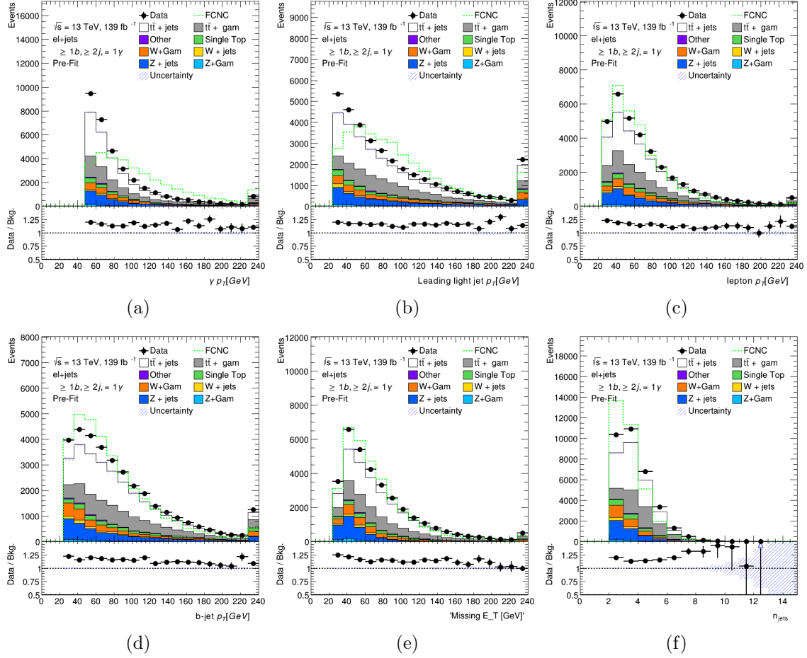
FIGURE 5.17. Photon p_T (a), leading light jet p_T (b), lepton p_T (c), b-jet p_T (d), \cancel{E}_T (e), and n_{\text{jets}} (f) plots in the signal region preselection for the electron+jets channel. FCNC signal branching ratio is scaled to 1.5%.
