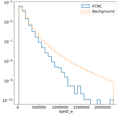
(a) E(b_{\text{jet}})
