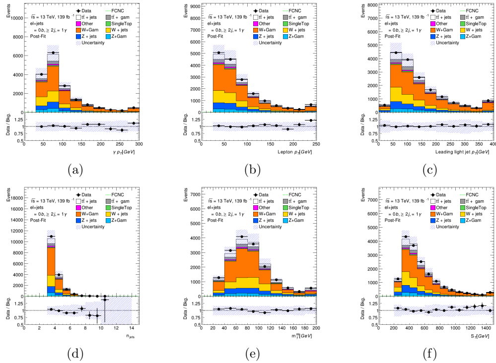
FIGURE F.1. Post-fit distributions for Photon p_T (a), lepton p_T (b), leading light jet p_T (c), n_{\text{jet}} (d), m_T^W (e), and S_T (f) in the W+\gamma validation region for the electron channel.
