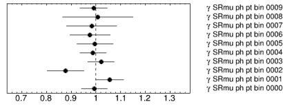
FIGURE 6.8. Bin by bin normalization \gamma factors used in each region for the \mu +jets channel.
