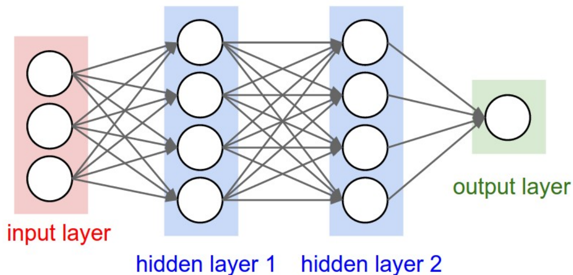
FIGURE 5.4. Pictorial representation of neural network architecture with three input variables, two hidden layers with four nodes each, and one output layer[83].
