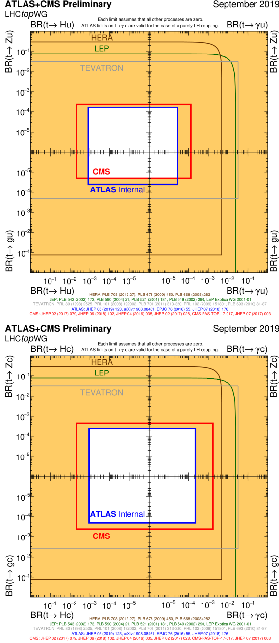
FIGURE 2.11. Flavor-changing neutral current limits from a variety of experiments in every channel t \rightarrow uX (top) and t \rightarrow cX (bottom)[23]. The blue box shows the current ATLAS limits on the FCNC processes, the vertical lines show the Higgs and \gamma limits while the horizontal lines show the Z and g limits.
