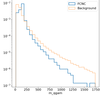
(c) m_{q\gamma}
