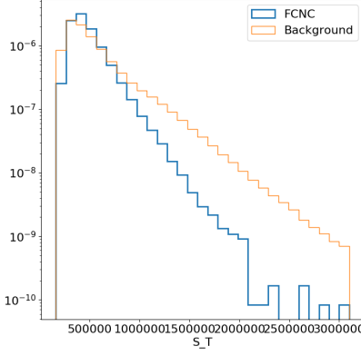
(c) S_T
