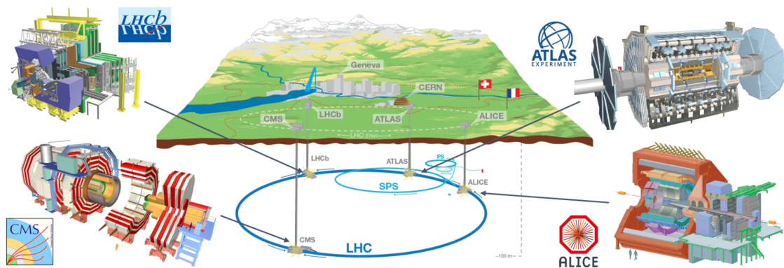
FIGURE 3.1. Map of LHC and the various detector experiments: ATLAS, CMS, LHCb, and ALICE located under the Franco-Swiss border near Geneva[35].
