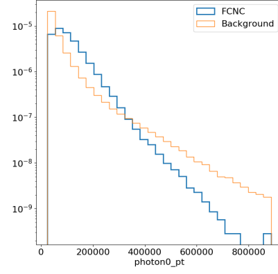
(b) \gamma_{pT}
