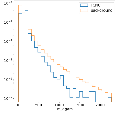
(c) m_{q\gamma}
