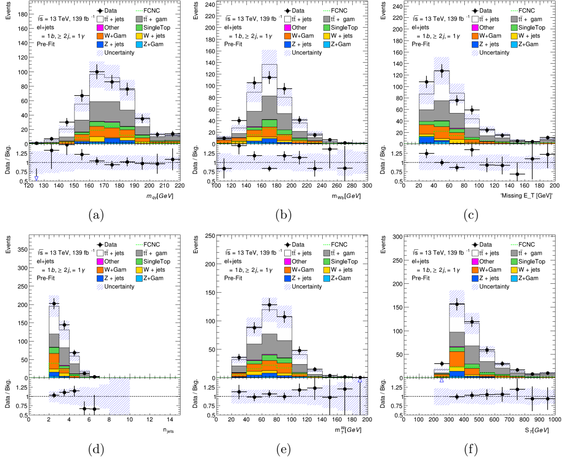
FIGURE 5.33. FCNC top candidate mass (a), Standard Model top candidate mass (b), \cancel{E}_T (c), N_{\text{jets}} (d), m_T^W (e), and S_T (f) pre-fit distributions in the final signal region with scale factors applied for the electron channel.
