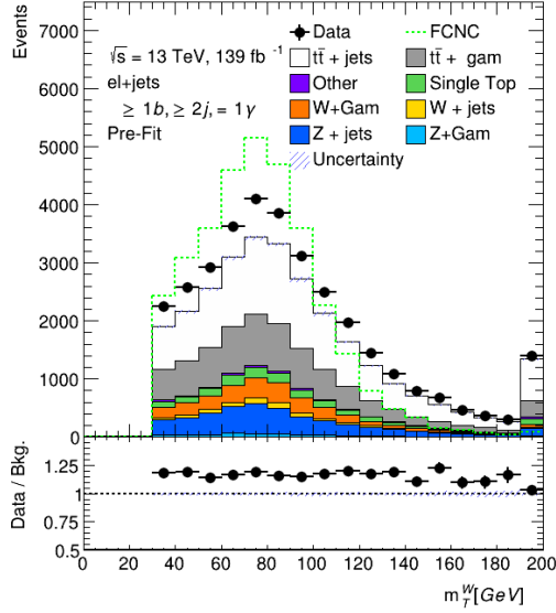
(a) electron channel
