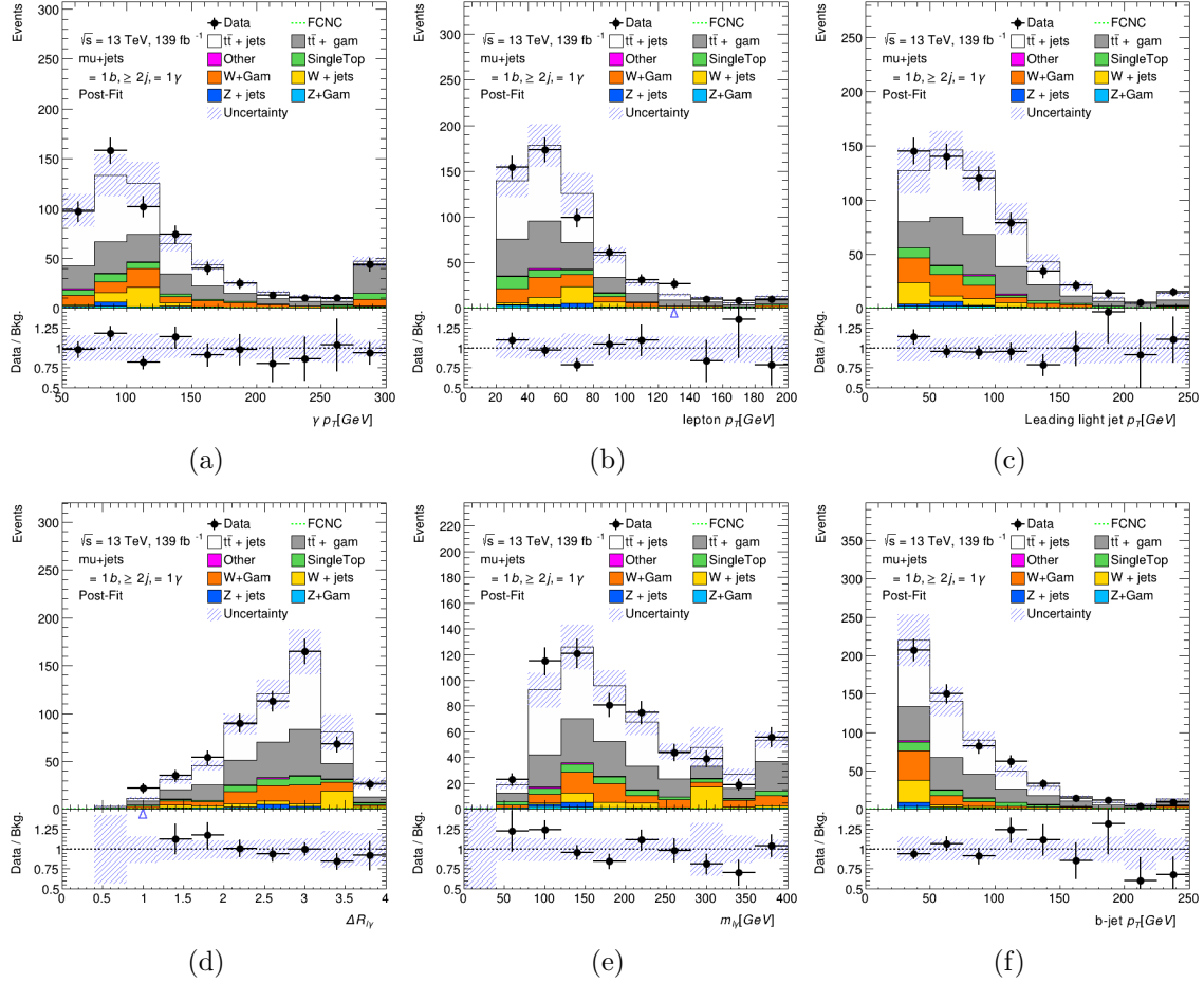
FIGURE 6.13. Post-fit distributions for Photon p_T (a), lepton p_T (b), leading light jet p_T (c), \Delta R_{l\gamma} (d), m_{l\gamma} (e), and b-jet p_T (f) in the final signal region for the muon channel.
