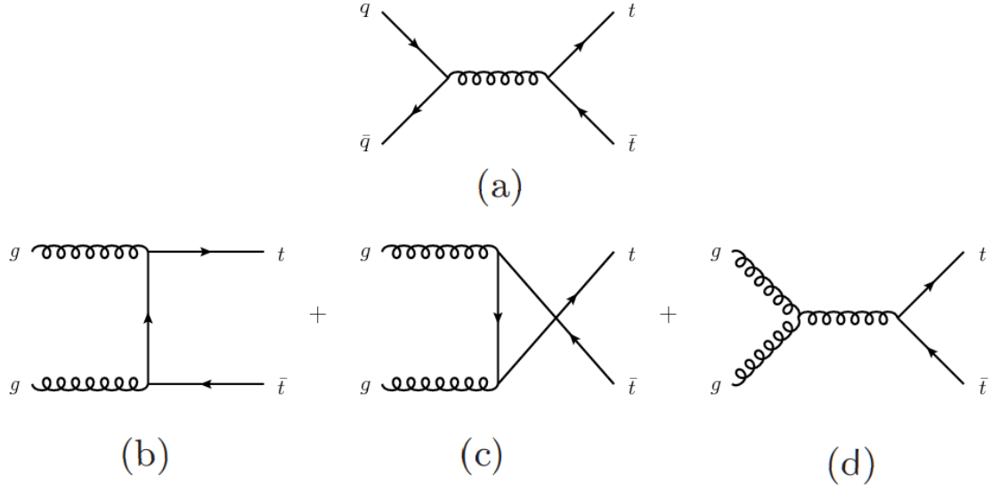
FIGURE 2.3. Leading order diagrams for the production of top/anti-top quark pairs at hadron colliders. Quark-antiquark annihilation diagram is shown in (a) while (b)-(d) show various gluon-gluon fusion diagrams.
