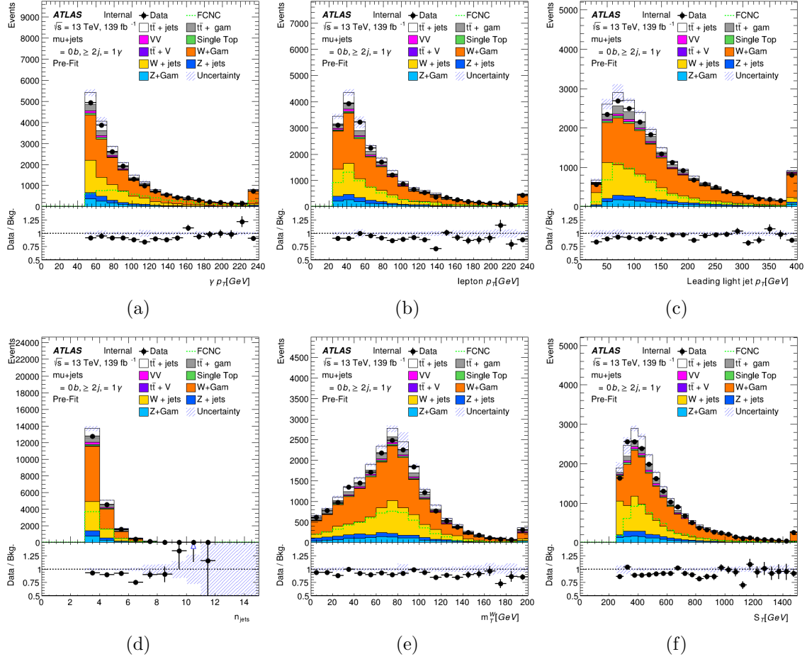
FIGURE 5.29. W +jets+ \gamma validation region plots for the muon channel after all scale factors are applied. The FCNC signal sample is scaled to 1%.
