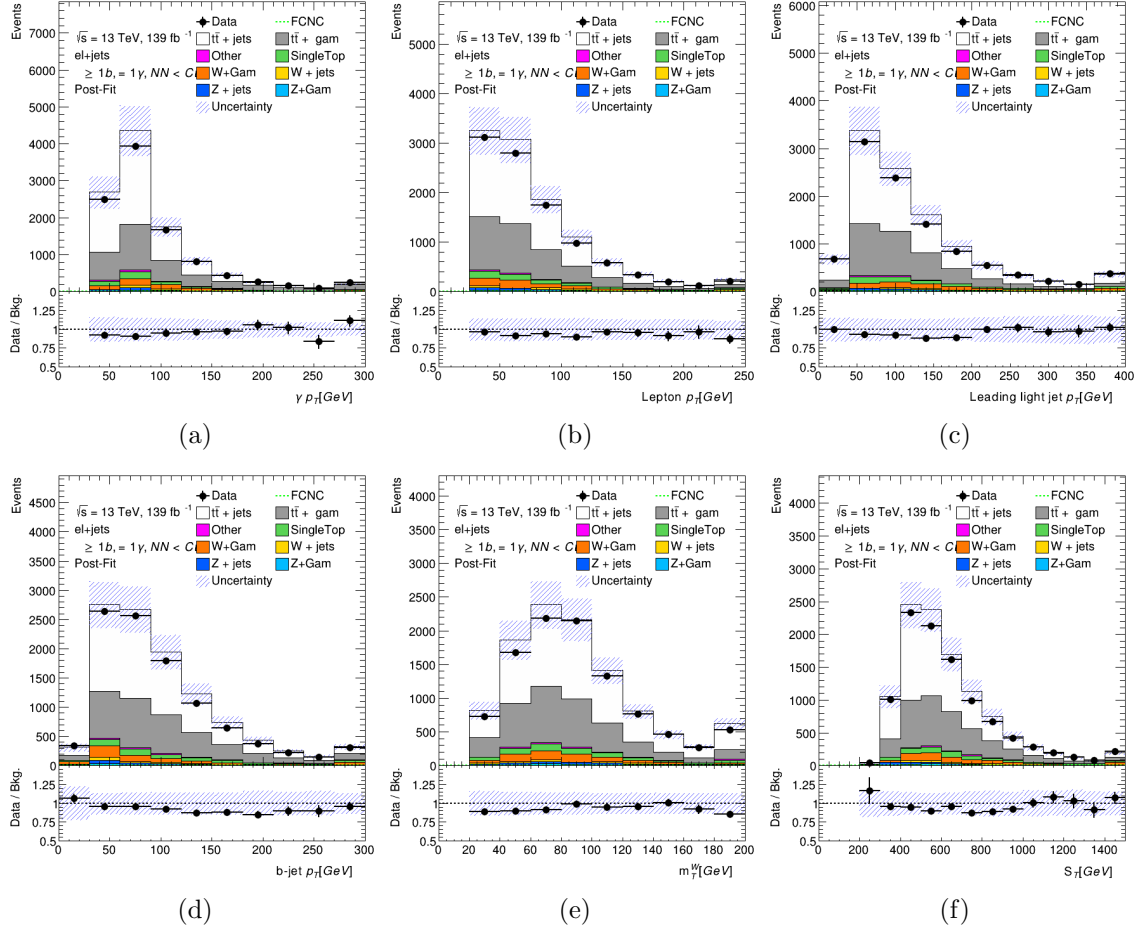
FIGURE F.2. Post-fit distributions for Photon p_T (a), lepton p_T (b), leading light jet p_T (c), leading b-jet p_T (d), m_T^W (e), and S_T (f) in the t\bar{t} + \text{jets} + \gamma validation region for the electron channel.
