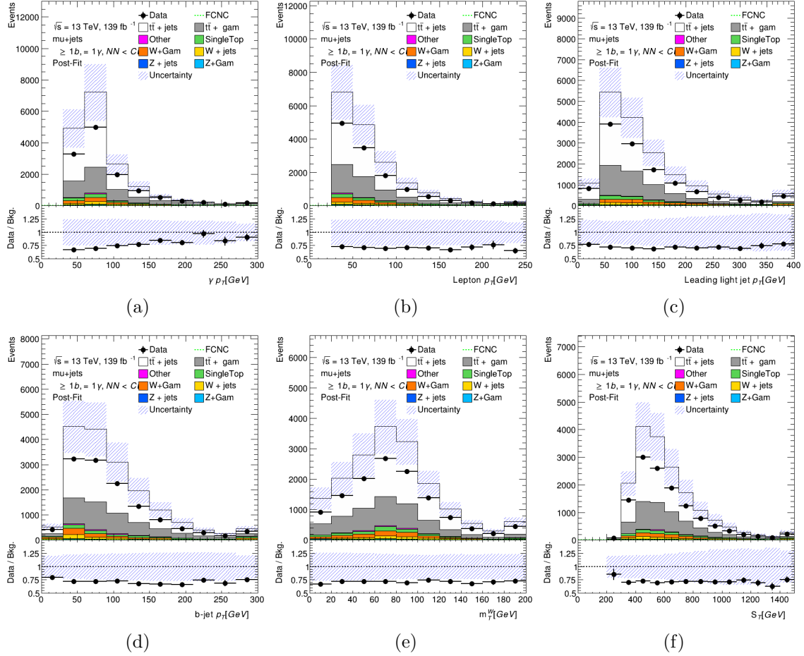
FIGURE F.4. Post-fit distributions for Photon p_T (a), lepton p_T (b), leading light jet p_T (c), leading b-jet p_T (d), m_T^W (e), and S_T (f) in the t\bar{t} + \text{jets} + \gamma validation region for the muon channel.
