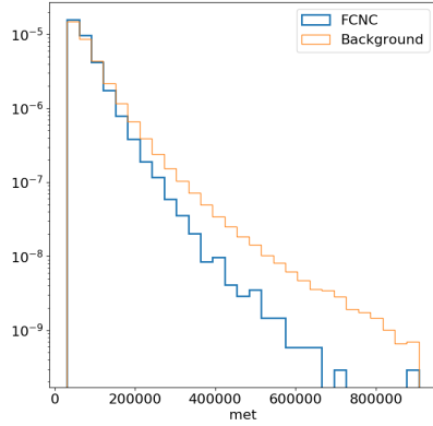
(c) \cancel{E}_T
