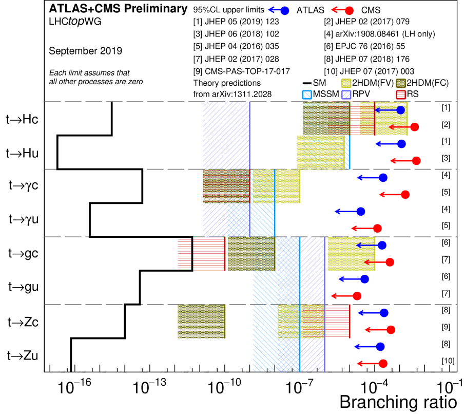
FIGURE 2.15. Flavor-changing neutral current theoretical branching ratios and experimental limits (both ATLAS and CMS) updated through 2018[23].
