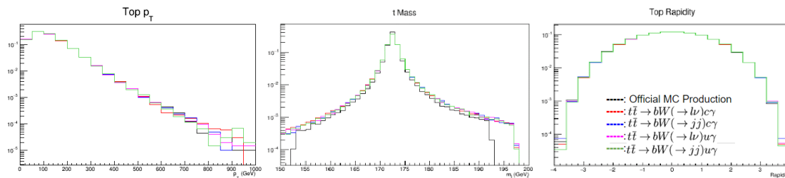
FIGURE 4.3. Normalized kinematics ( p_T , m_t , and y_t ) of individual top quarks produced by the model for each FCNC final state search and an official t\bar{t} sample.
