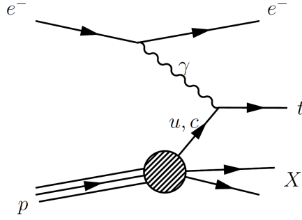
FIGURE 2.12. FCNC diagram for the search in single top production at the electron-proton collider HERA.
