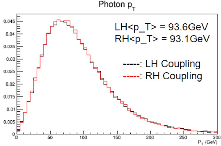
FIGURE 4.8. Normalized p_T of the photons produced by the model using the Left-handed (LH) and Right-handed (RH) couplings.
