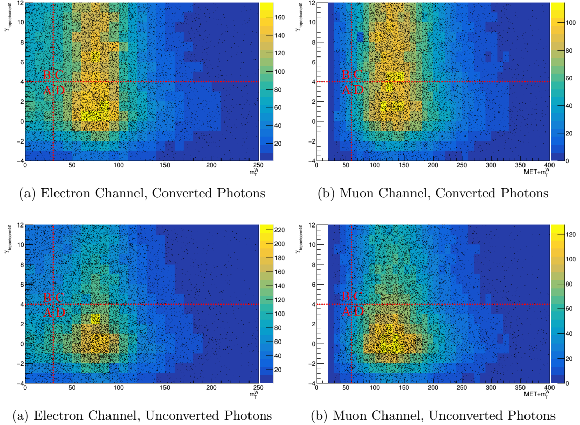
FIGURE 5.27. Regions used for the ABCD method shown for both converted and unconverted photon types. MC events are shown in the gradient histogram and data events are shown with the black points. All final signal region cuts are included except the neural network cut to give enough statistics in the regions for the ABCD method to be a reasonable estimate of the fake rate scale factor.
