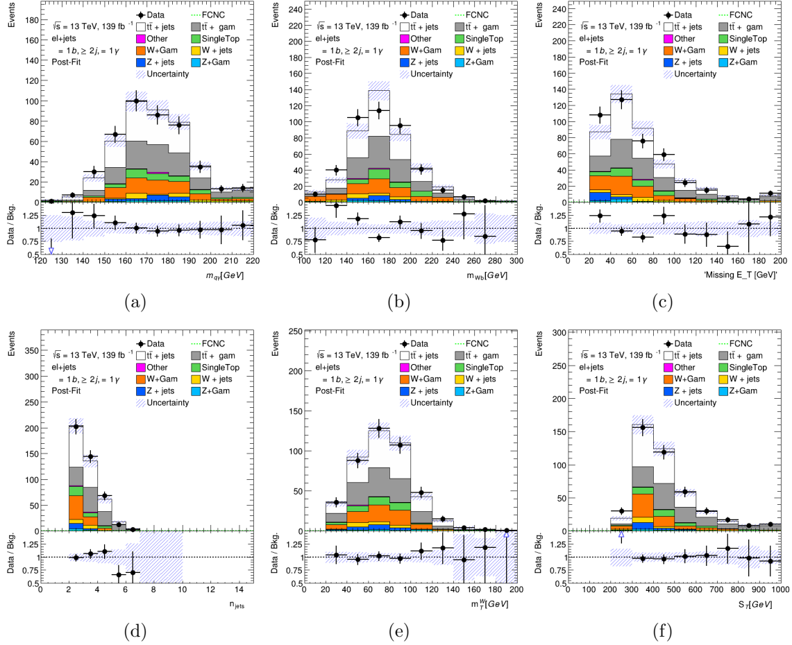
FIGURE 6.12. Post-fit distributions for FCNC top candidate mass (a), Standard Model top candidate mass (b), E_T (c), N_{\text{jets}} (d), m_T^W (e), and S_T (f) in the final signal region for the electron channel.
