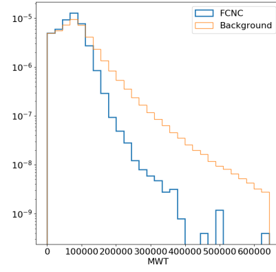
(b) m_T^W
