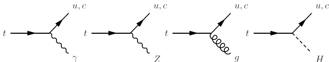
FIGURE 2.10. Flavor-changing neutral current top quark decays.
