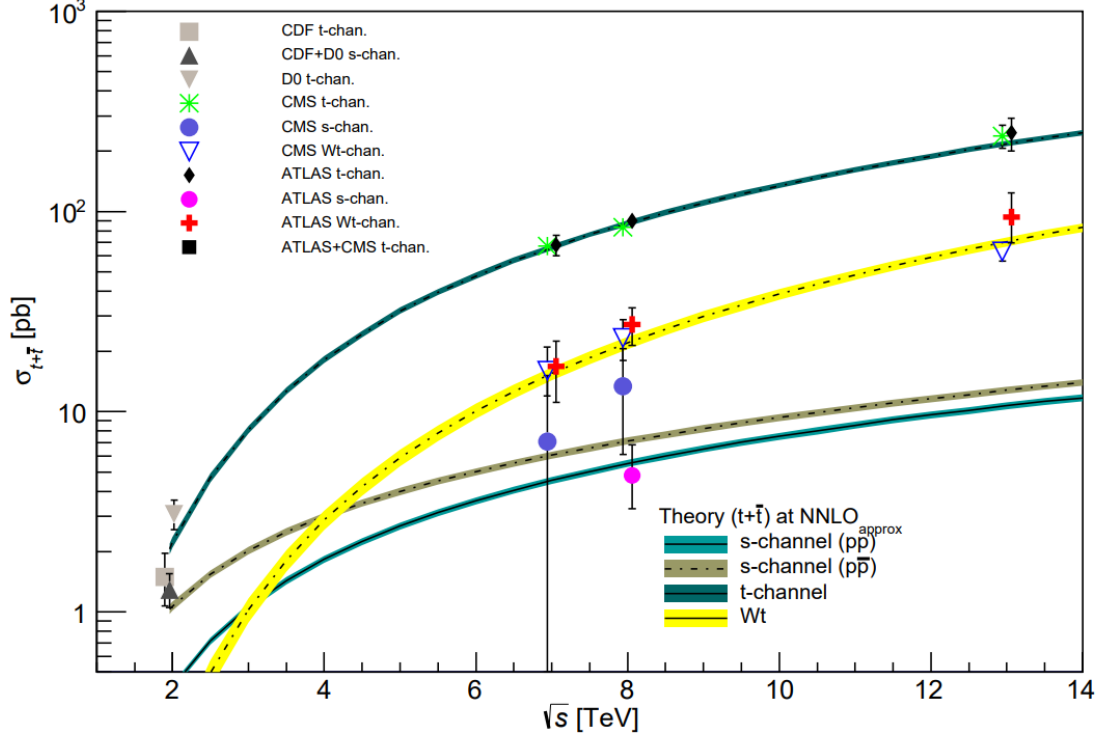
FIGURE 2.2. Summary of single-top production cross sections as a function of center-of-mass energy at Fermilab’s Tevatron and CERN’s LHC[23].
