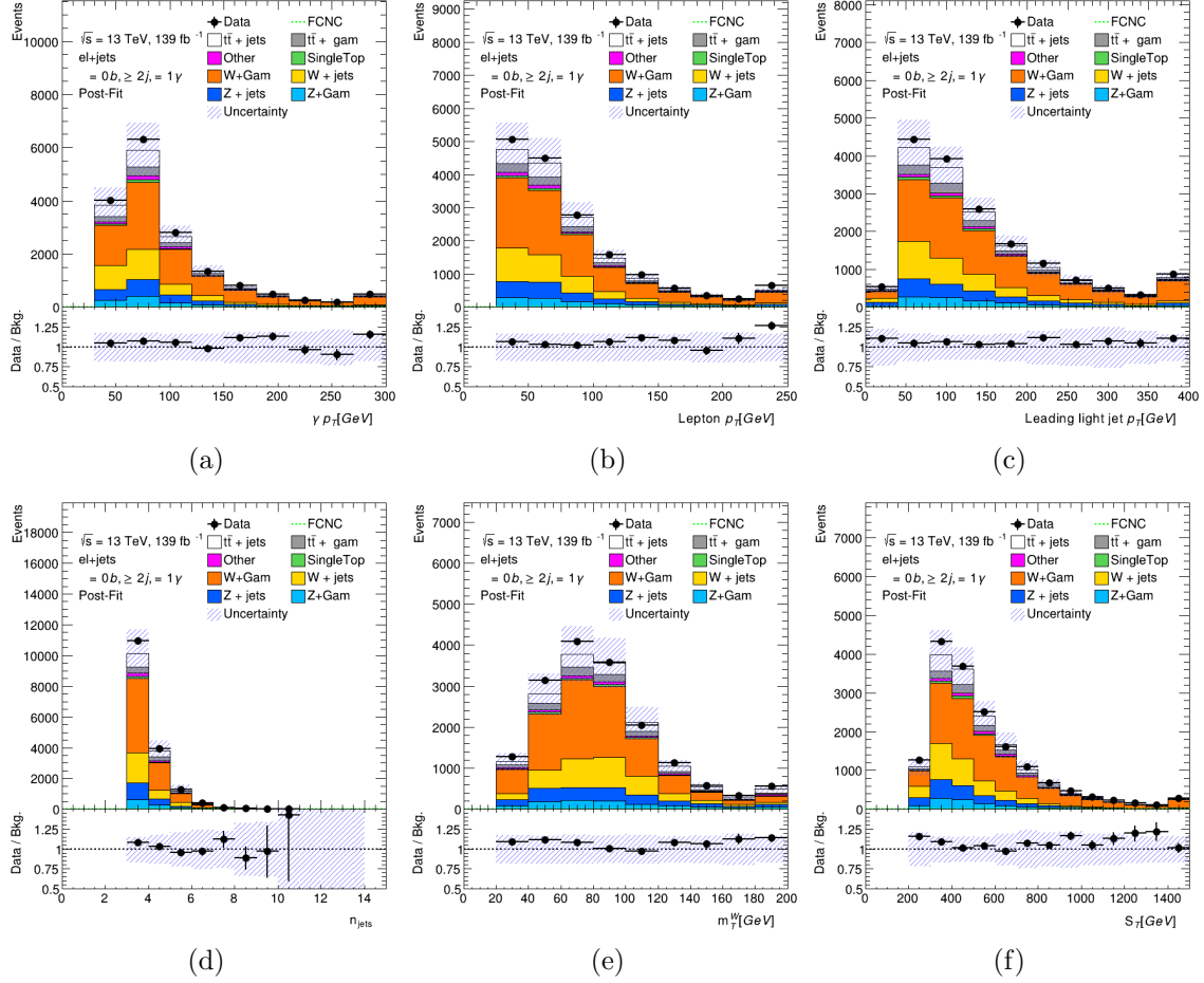
FIGURE G.9. Post-fit distributions for Photon p_T (a), lepton p_T (b), leading light jet p_T (c), n_{jet} (d), m_T^W (e), and S_T (f) in the W+ \gamma validation region for the e+jets channel for alternative fit using \gamma p_T in both regions.
