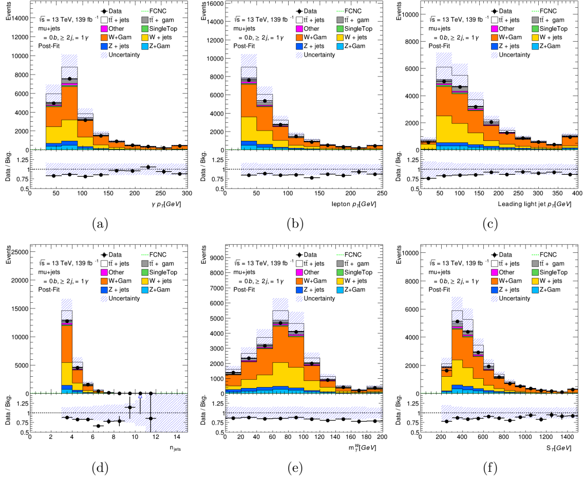
FIGURE F.3. Post-fit distributions for Photon p_T (a), lepton p_T (b), leading light jet p_T (c), n_{jet} (d), m_T^W (e), and S_T (f) in the W+ \gamma validation region for the muon channel.
