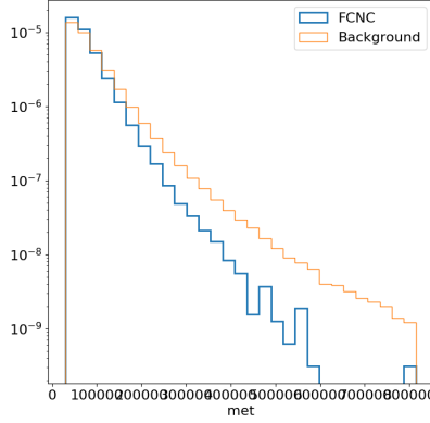
(c) \cancel{E}_T
