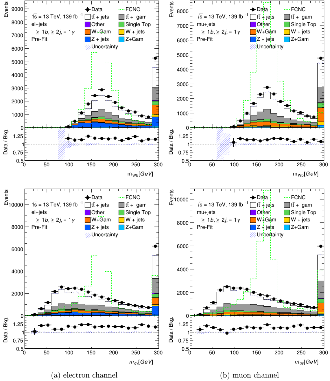
FIGURE 5.16. Top mass candidates in the signal region preselection: m_{Wb} and m_{q\gamma} . FCNC signal branching ratio is scaled to 1.5%.
