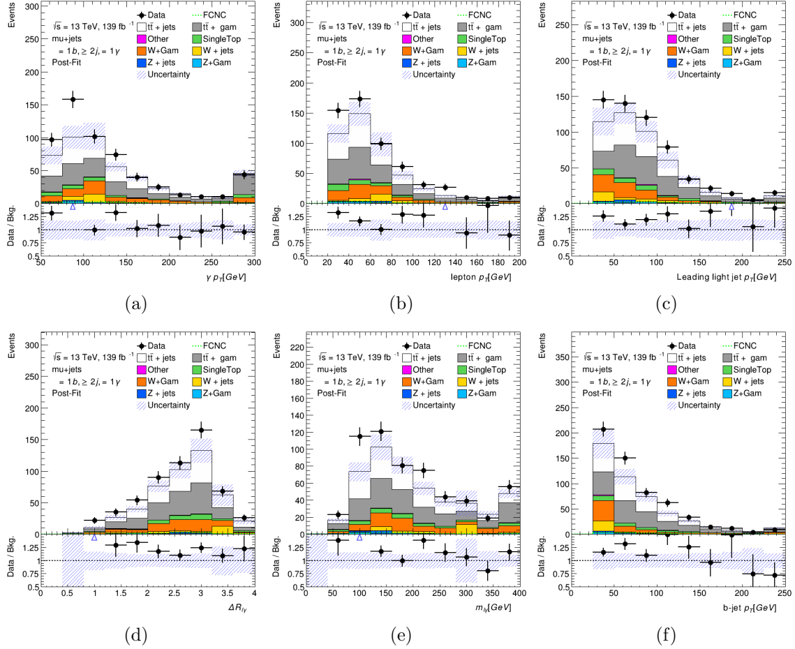
FIGURE G.1. Post-fit distributions for Photon p_T (a), lepton p_T (b), leading light jet p_T (c), \Delta R_{l\gamma} (d), m_{l\gamma} (e), and b-jet p_T (f) in the final signal region for the muon channel fitting on m_{q\gamma} .
