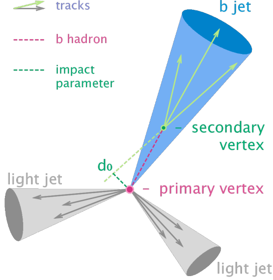
FIGURE 4.11. Pictorial representation of an event with a b-jet showing the secondary vertex and impact parameter[76].
