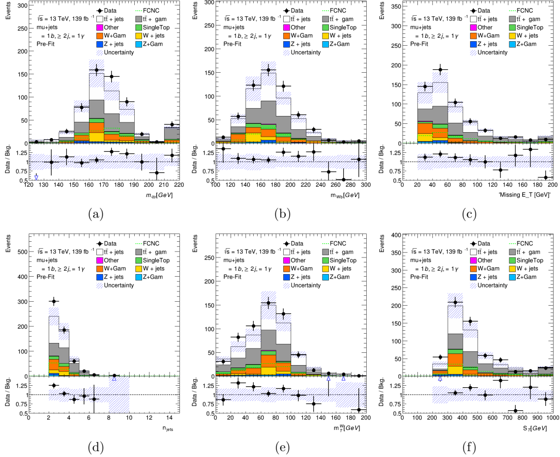
FIGURE 5.35. FCNC top candidate mass (a), Standard Model top candidate mass (b), \cancel{E}_T (c), N_{\text{jets}} (d), m_T^W (e), and S_T (f) pre-fit distributions in the final signal region with scale factors applied for the muon channel.
