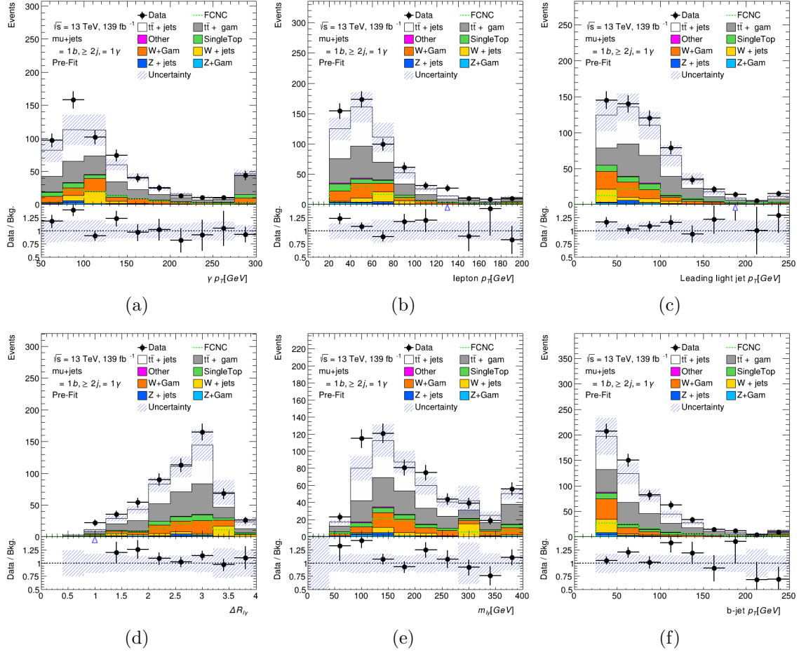
FIGURE 5.34. Photon p_T (a), lepton p_T (b), leading light jet p_T (c), \Delta R_{l\gamma} (d), m_{l\gamma} (e), and b-jet p_T (f) pre-fit distributions in the final signal region with scale factors applied for the muon channel.
