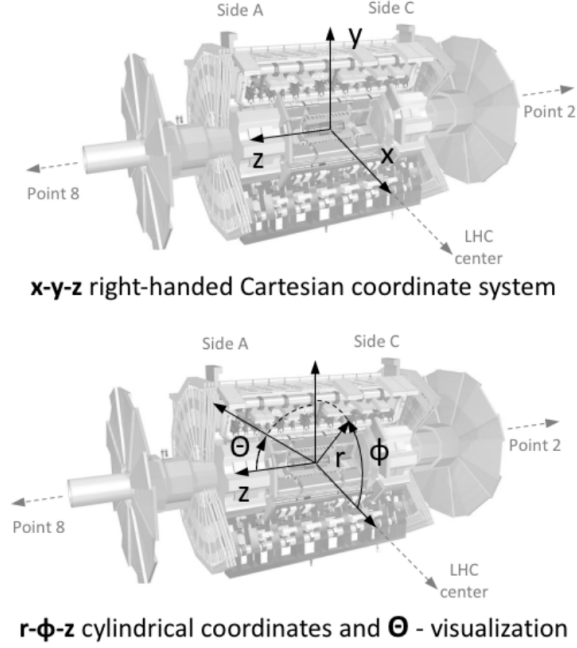
FIGURE 3.8. Coordinate system used in the ATLAS Collaboration[35].
