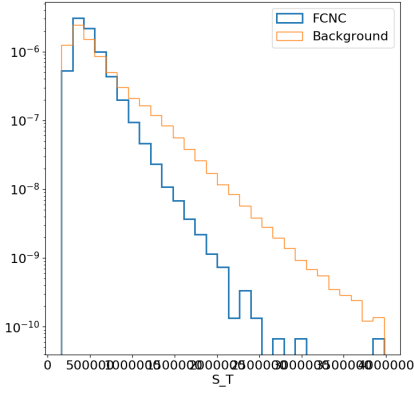
(c) S_T
