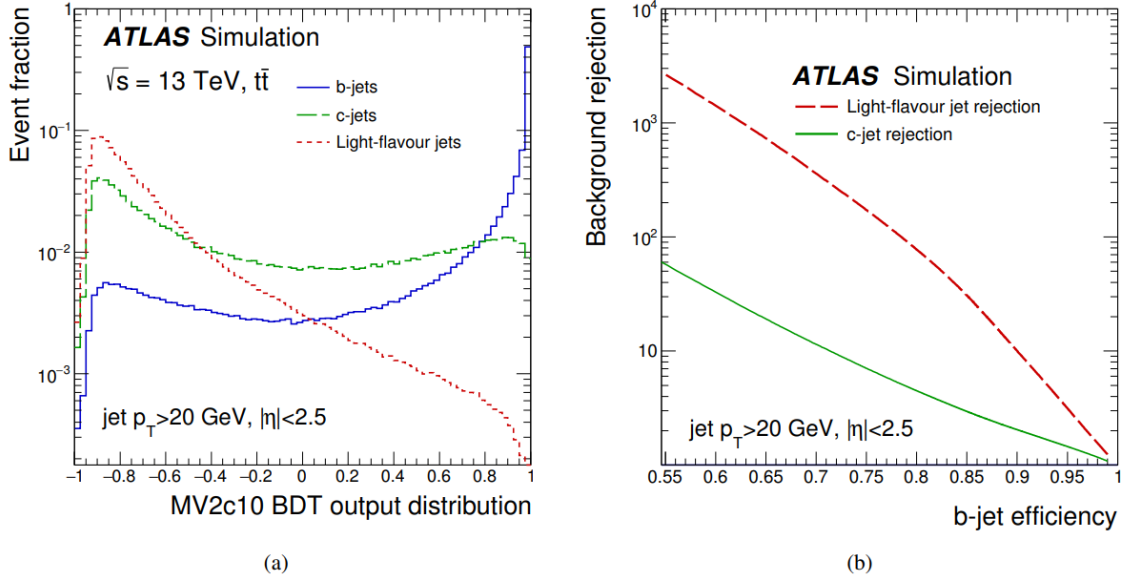
FIGURE 4.12. The MV2c10 output for b, c, and light flavored jets in simulated t\bar{t} and the background rejection as a function of the b-jet efficiency[78].
