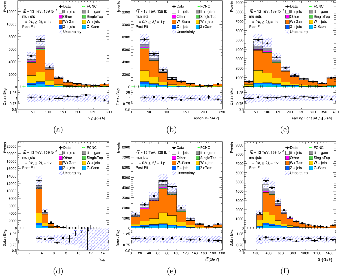
FIGURE G.4. Post-fit distributions for Photon p_T (a), lepton p_T (b), leading light jet p_T (c), n_{jet} (d), m_T^W (e), and S_T (f) in the W+\gamma validation region for the \mu +jets channel for alternative fit using m_{q\gamma} in both regions.
