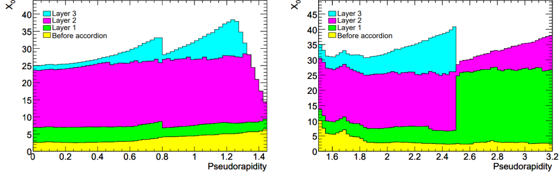
FIGURE 3.15. Number of radiation lengths throughout the LAr calorimeter as a function of |\eta| . [38]
