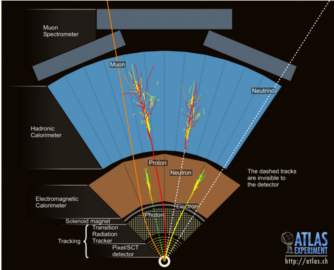
FIGURE 4.9. Cross section of a simulated ATLAS detector showing how various particles interact with ATLAS subsystems. Solid lines indicate interactions while dashed lines indicate that no interactions typically occur in that section of the detector [64].
