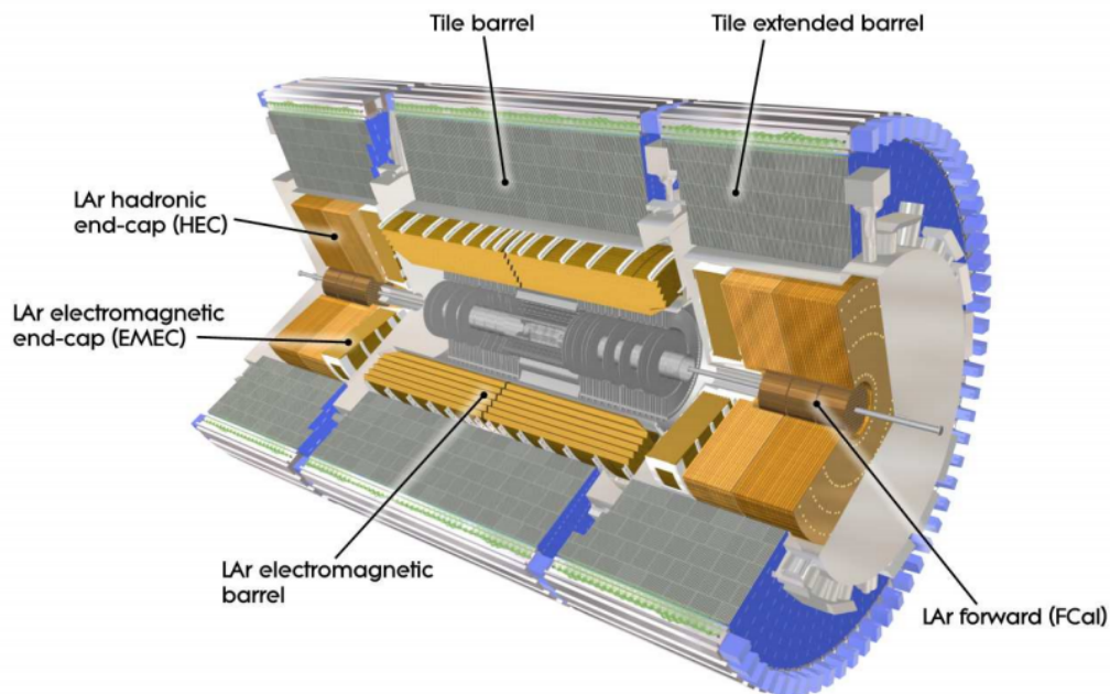
FIGURE 3.13. Schematic of the ATLAS hadronic and electromagnetic calorimeter systems[38].
