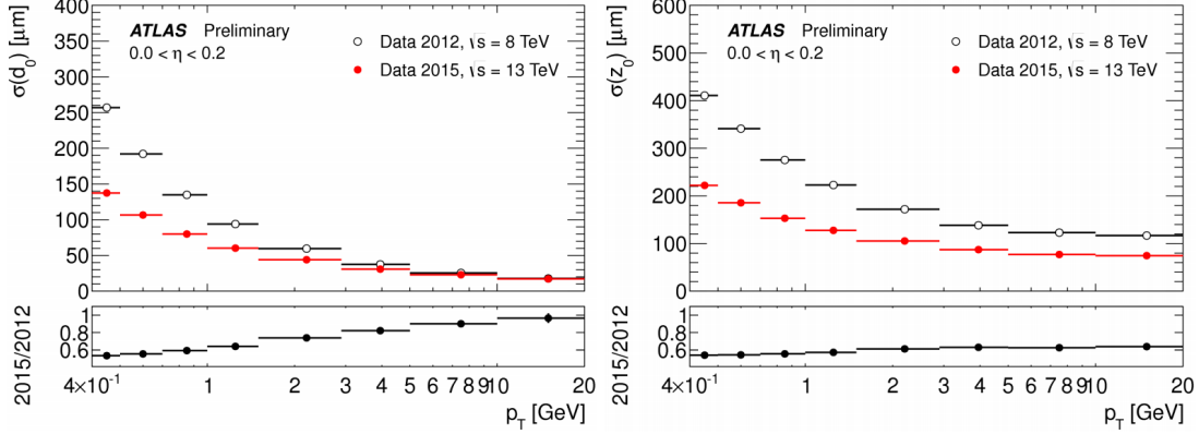
FIGURE 3.11. Unfolded transverse (left) and longitudinal (right) impact parameter resolution measured with (Run-2) and without (Run-1) the IBL as a function of p_T [41].
