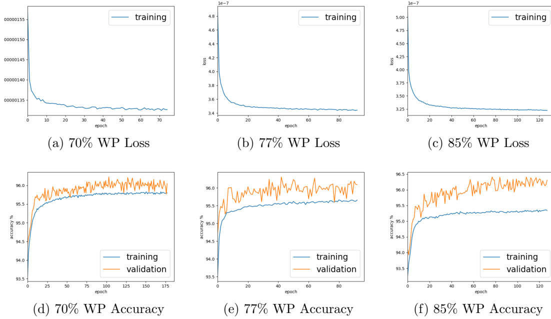
FIGURE 5.10. Accuracy and loss plots for the e +jets channel at 70%, 77%, and 85% b-tagging working points.
