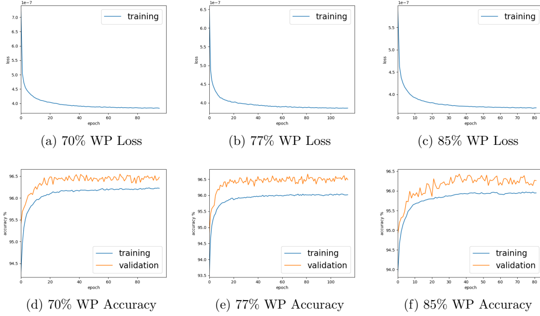
FIGURE 5.11. Accuracy and loss plots for the \mu +jets channel at 70%, 77%, and 85% b-tagging working points.
