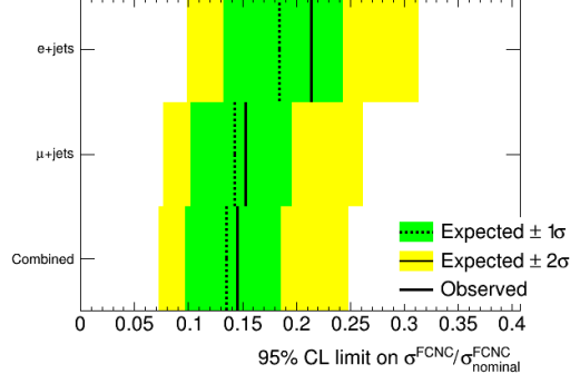
FIGURE G.8. Limits on the signal strength \mu for the alternative fit using \gamma p_T in both regions.
