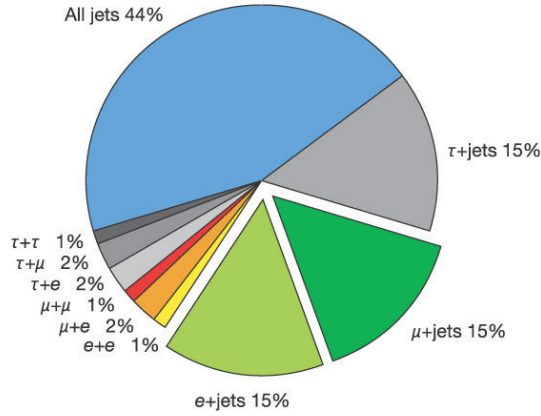
FIGURE 2.6. Categorization of top quark pair decays in the Standard Model based on the decays of the W bosons[24].
