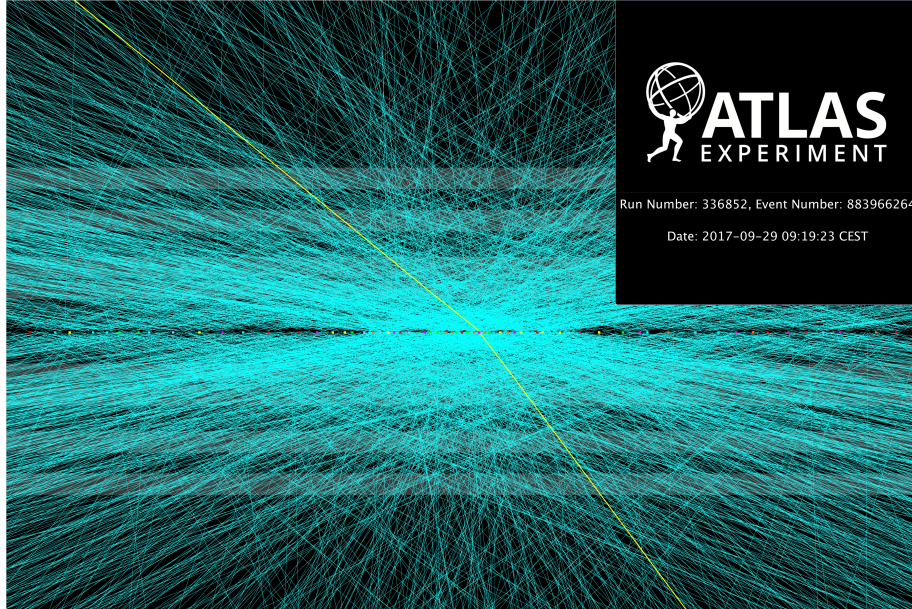
FIGURE 3.6. A candidate dimuon event ( Z \rightarrow \mu^+ \mu^- ) with 65 reconstructed vertices collected in 2017 with the ATLAS detector[37].
