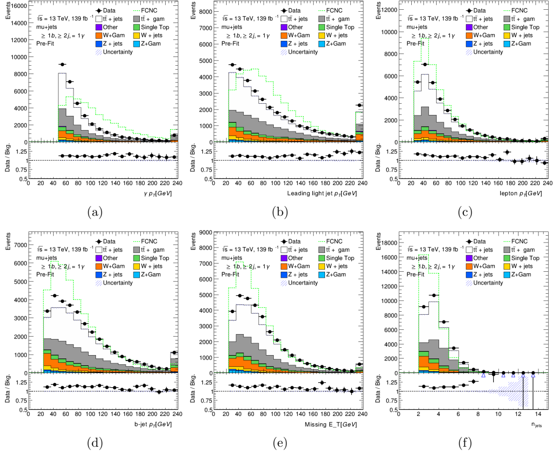
FIGURE 5.18. Photon p_T (a), leading light jet p_T (b), lepton p_T (c), b-jet p_T (d), \cancel{E}_T (e), and n_{\text{jets}} (f) plots in the signal region preselection for the muon+jets channel. FCNC signal branching ratio is scaled to 1.5%.
