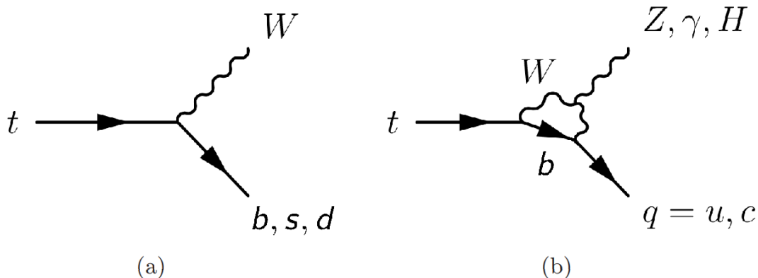
FIGURE 2.5. Top quark decays in the Standard Model.
