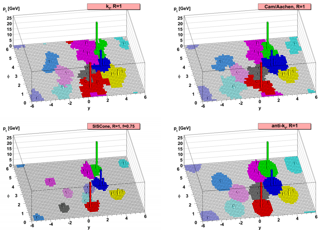
FIGURE 4.10. A sample parton-level event with many random soft jet objects, clustered with four different jets algorithms, illustrating the areas of the resulting hard jets. For kt and Cambridge/Aachen the detailed shapes are in part determined by the specific set of ghosts used, and change when the ghosts are modified[70].
