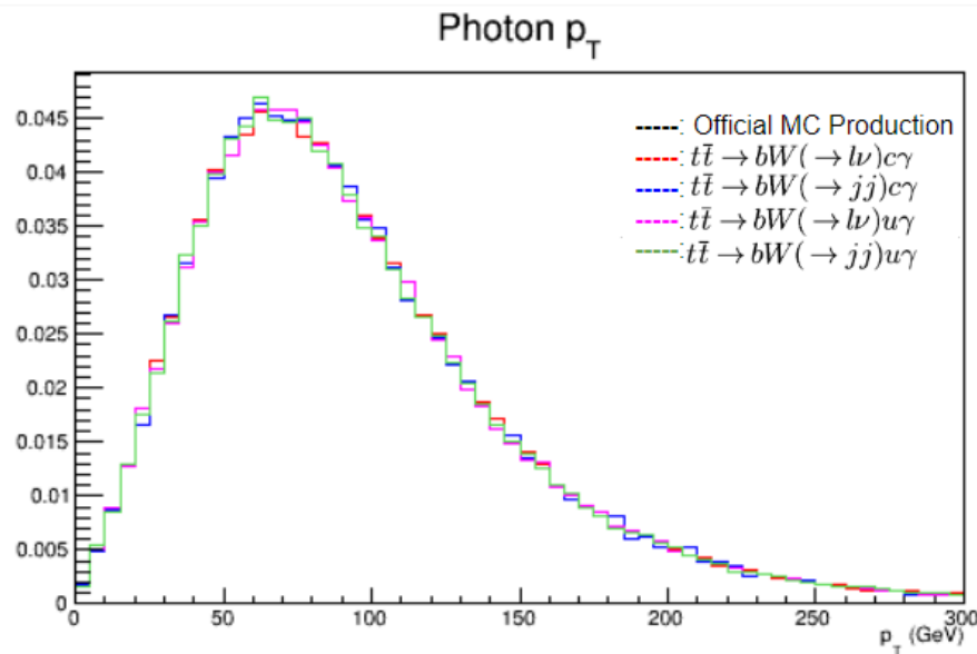
FIGURE 4.7. Normalized p_T of the photons produced by the model for each FCNC final state search and an official t\bar{t} sample. There is 0 contribution from the official t\bar{t} sample.
