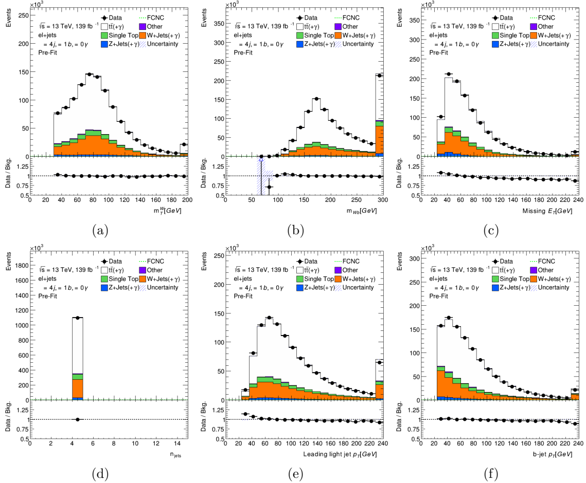
FIGURE 5.21. Event-level plots for the =4 jet validation region after scale factors have been applied in the electron channel. FCNC signal branching ratio is scaled to 0.1%.
