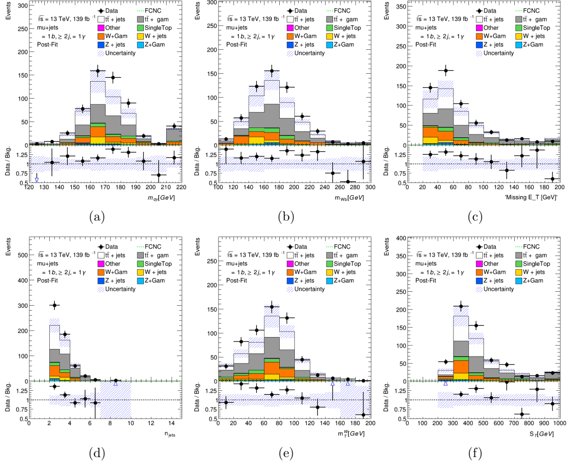
FIGURE G.2. Post-fit distributions for FCNC top candidate mass (a), Standard Model top candidate mass (b), E_T (c), N_{\text{jets}} (d), m_T^W (e), and S_T (f) in the final signal region for the muon channel fitting on m_{q\gamma} .
