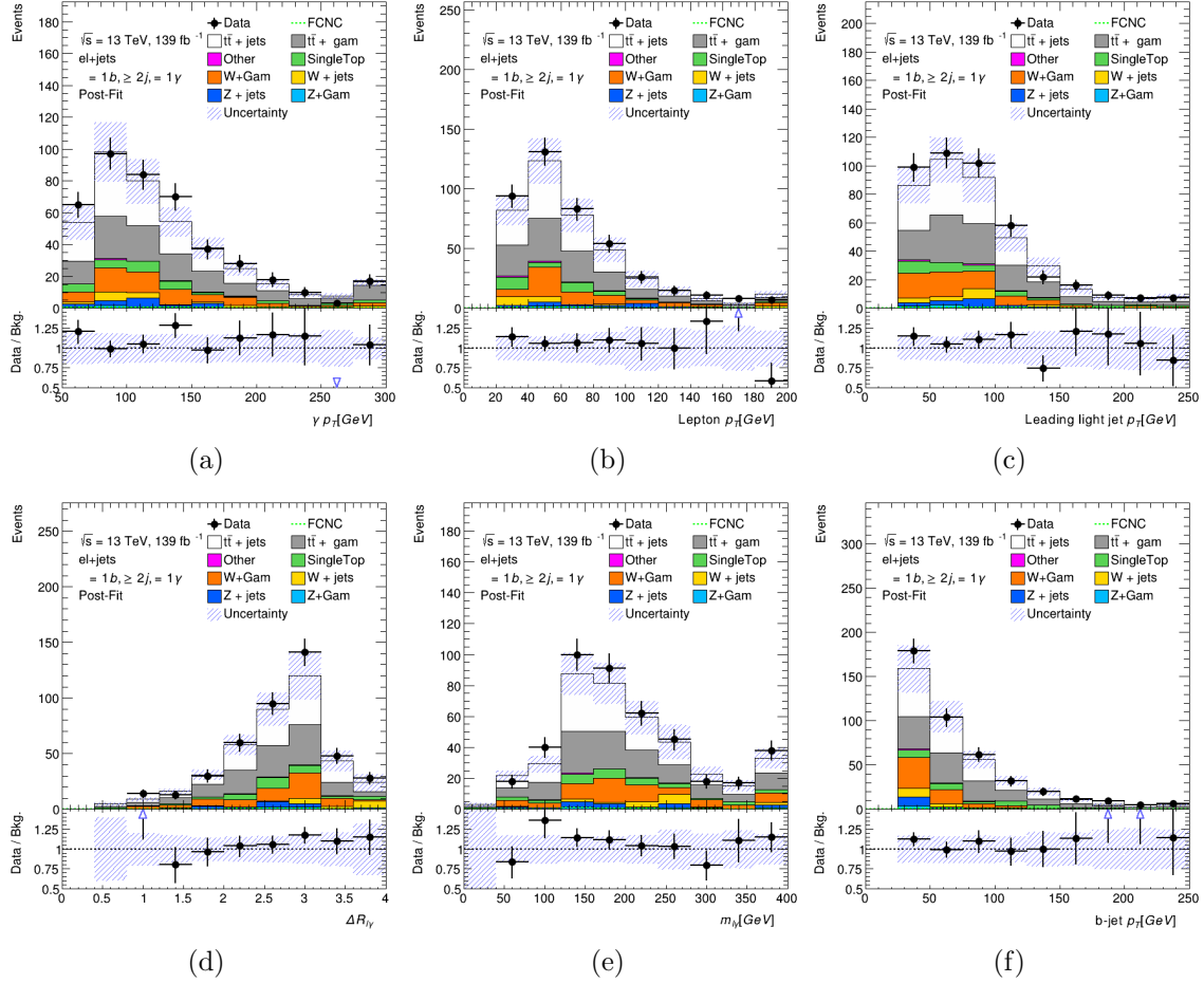
FIGURE G.6. Post-fit distributions for Photon p_T (a), lepton p_T (b), leading light jet p_T (c), \Delta R_{l\gamma} (d), m_{l\gamma} (e), and b-jet p_T (f) in the final signal region for the electron channel fitting on \gamma p_T .
