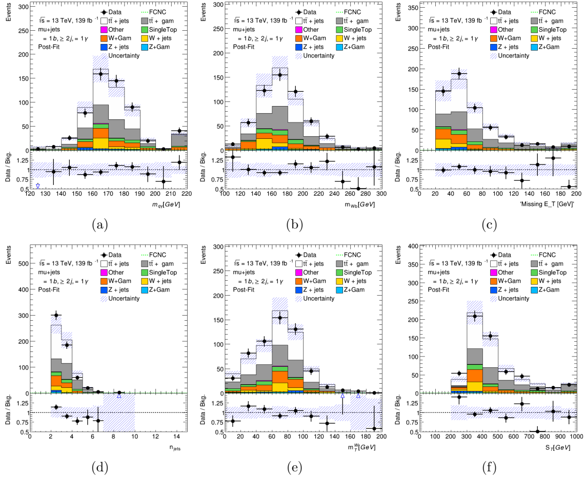
FIGURE 6.14. Post-fit distributions for FCNC top candidate mass (a), Standard Model top candidate mass (b), \cancel{E}_T (c), N_{\text{jets}} (d), m_T^W (e), and S_T (f) in the final signal region for the muon channel.
