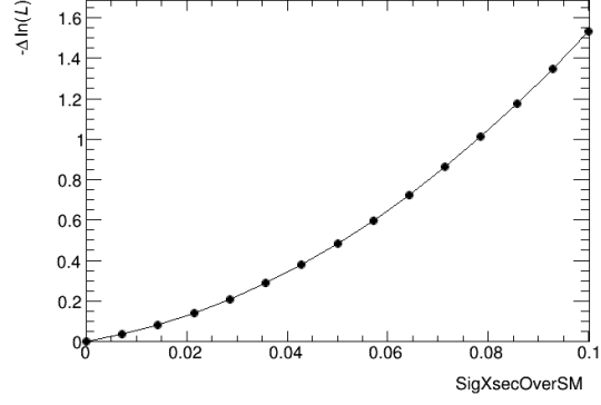
FIGURE 6.4. Negative-log likelihood (goodness of fit) as a function of signal strength using data in all regions for the e +jets channel.
