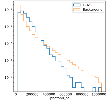
(b) \gamma_{pT}
