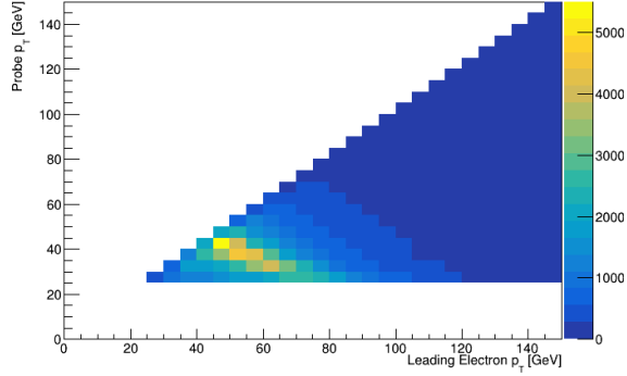
(a) Probe: Electrons
