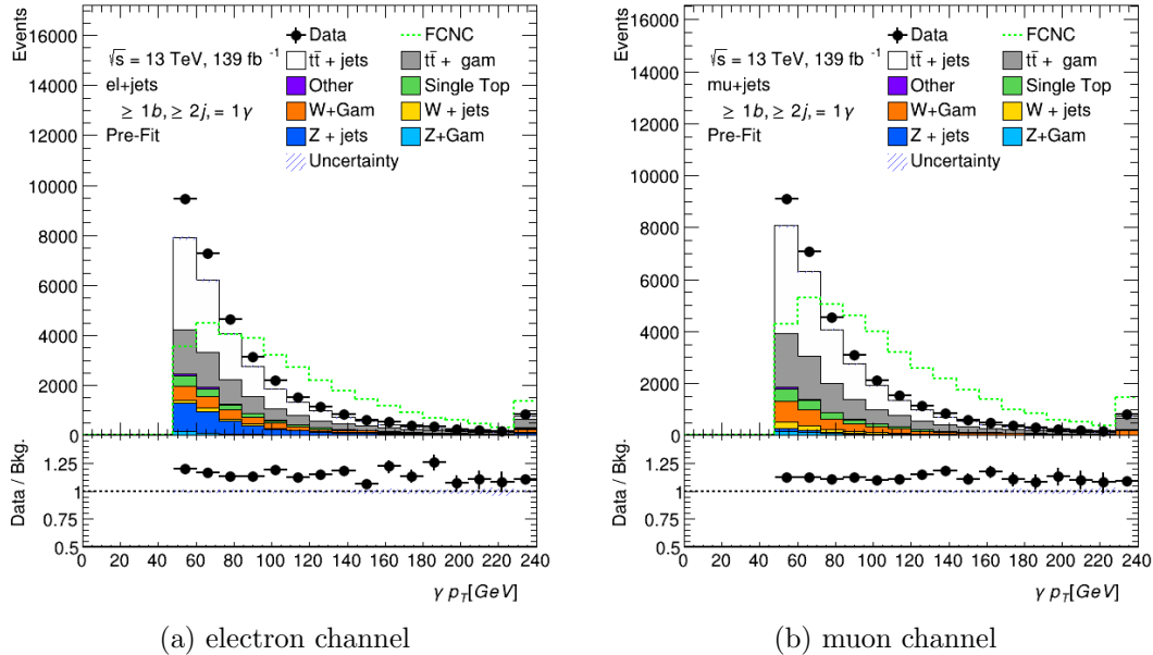
FIGURE 5.14. Photon p_T in the signal region preselection region. FCNC signal branching ratio is scaled to 1.5%.
