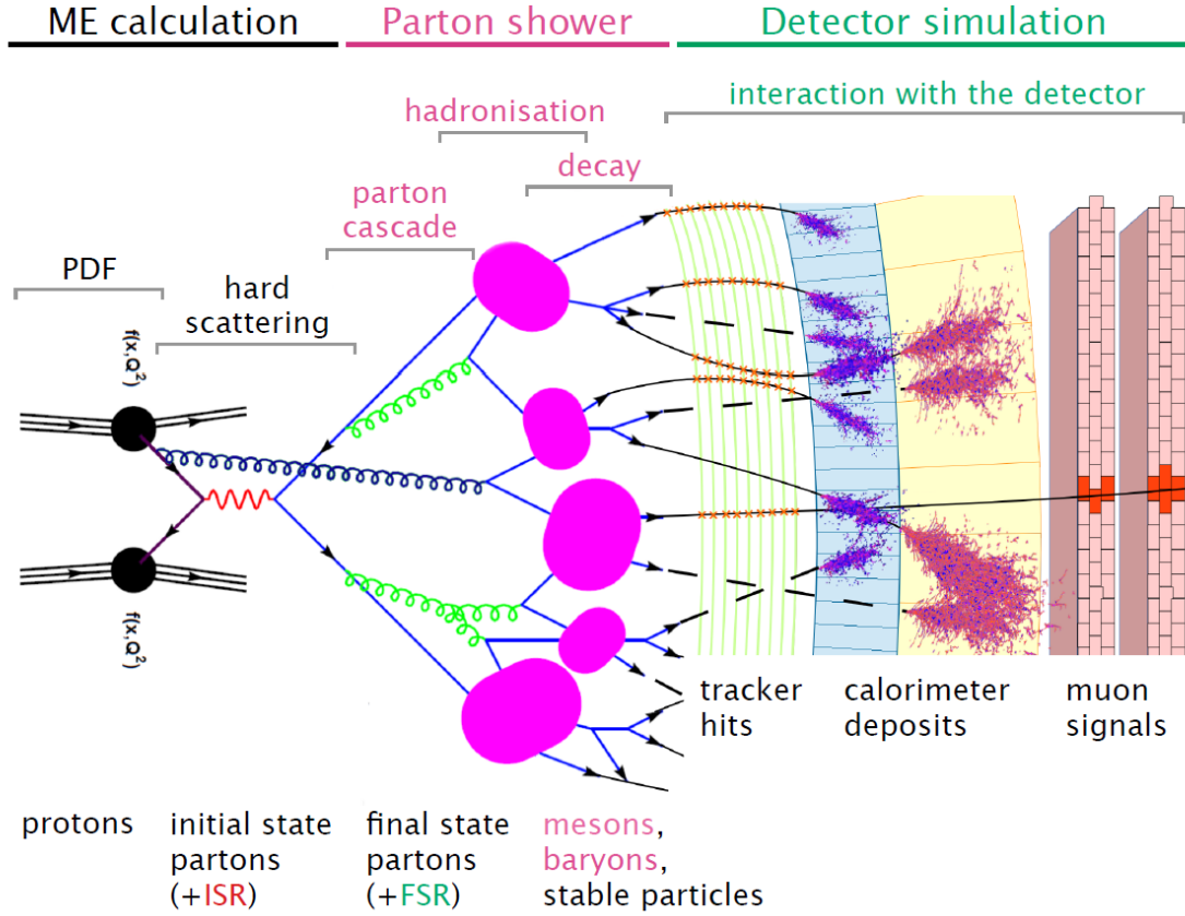
FIGURE 4.1. A pictorial view of the different steps for the creation of a MC event[48].
