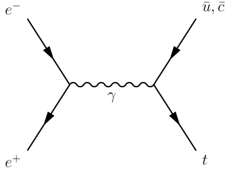
FIGURE 2.13. FCNC diagram for the search in single top production at the electron-positron collider, LEP.
