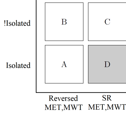
FIGURE 5.26. Pictorial representation of the regions used for the ABCD method in this search.
