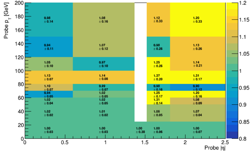
(b) Unconverted Photons
