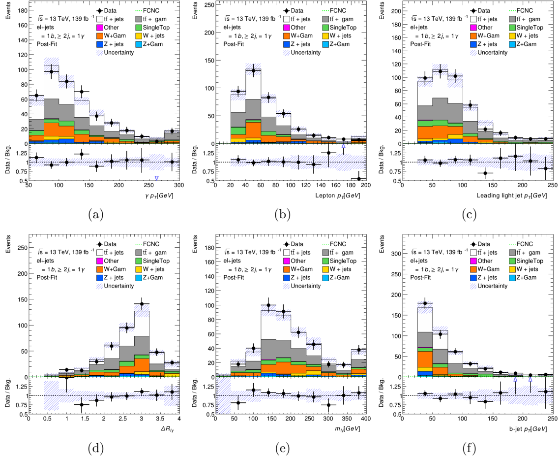
FIGURE 6.11. Post-fit distributions for Photon p_T (a), lepton p_T (b), leading light jet p_T (c), \Delta R_{l\gamma} (d), m_{l\gamma} (e), and b-jet p_T (f) in the final signal region for the electron channel.
