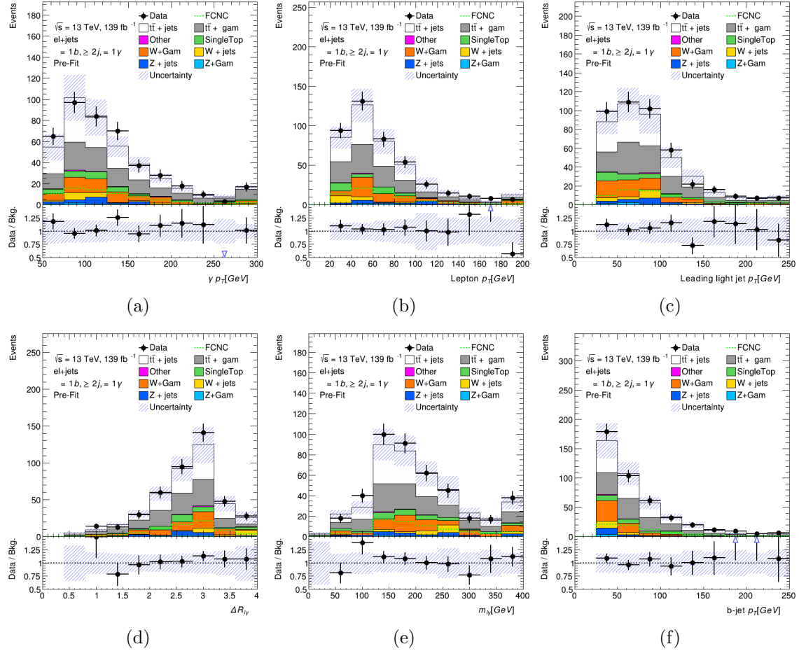
FIGURE 5.32. Photon p_T (a), lepton p_T (b), leading light jet p_T (c), \Delta R_{l\gamma} (d), m_{l\gamma} (e), and b-jet p_T (f) pre-fit distributions in the final signal region with scale factors applied for the electron channel.
