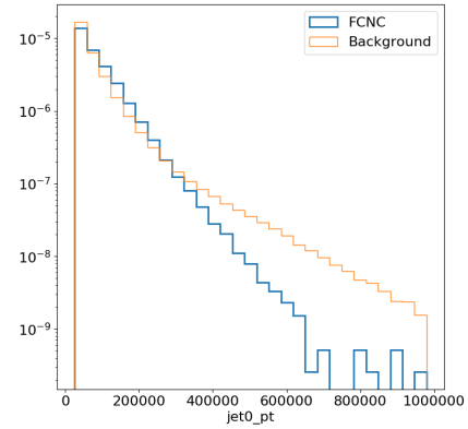
(f) p_T(q)
