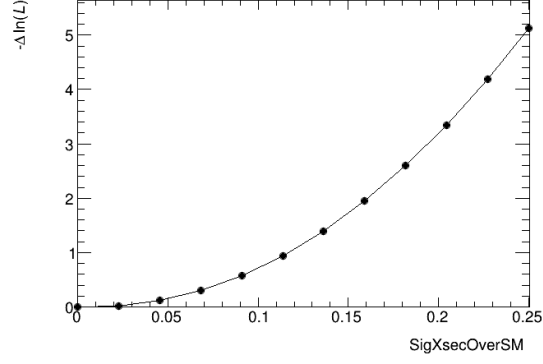
FIGURE 6.9. Negative-log likelihood (goodness of fit) as a function of signal strength using data in all regions for the \mu +jets channel.
