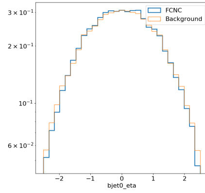
(b) \eta_b
