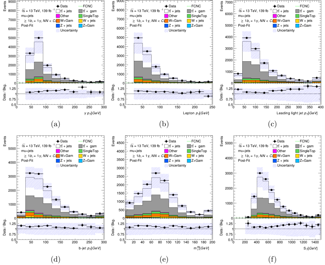
FIGURE G.5. Post-fit distributions for Photon p_T (a), lepton p_T (b), leading light jet p_T (c), leading b-jet p_T (d), m_T^W (e), and S_T (f) in the t\bar{t} + \text{jets} + \gamma validation region for the \mu + \text{jets} channel for alternative fit using m_{q\gamma} in both regions.
