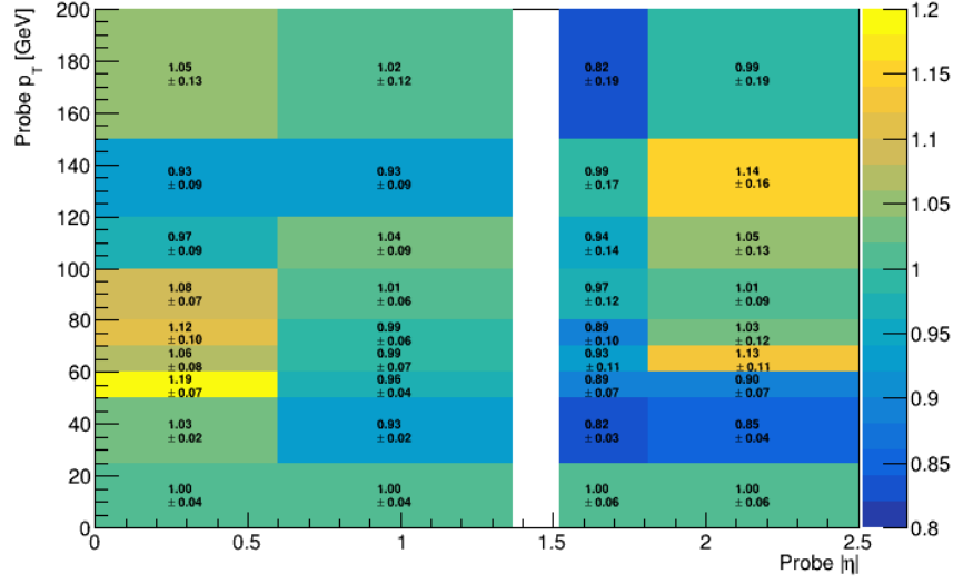
(a) Converted Photons
