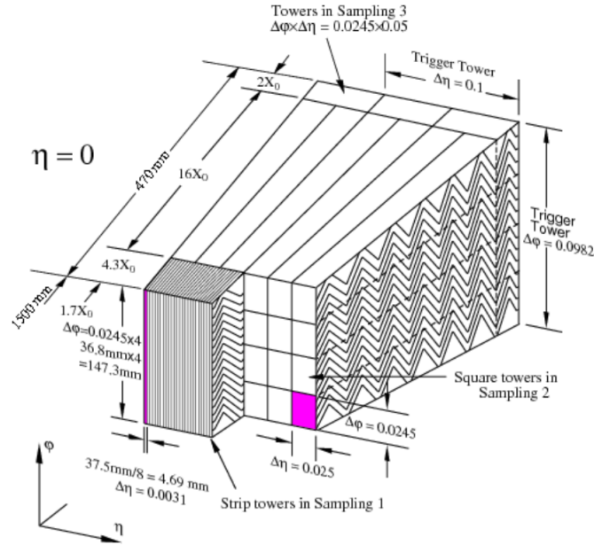
FIGURE 3.14. Sketch of the accordion structure used in the LAr Calorimeter[44].
