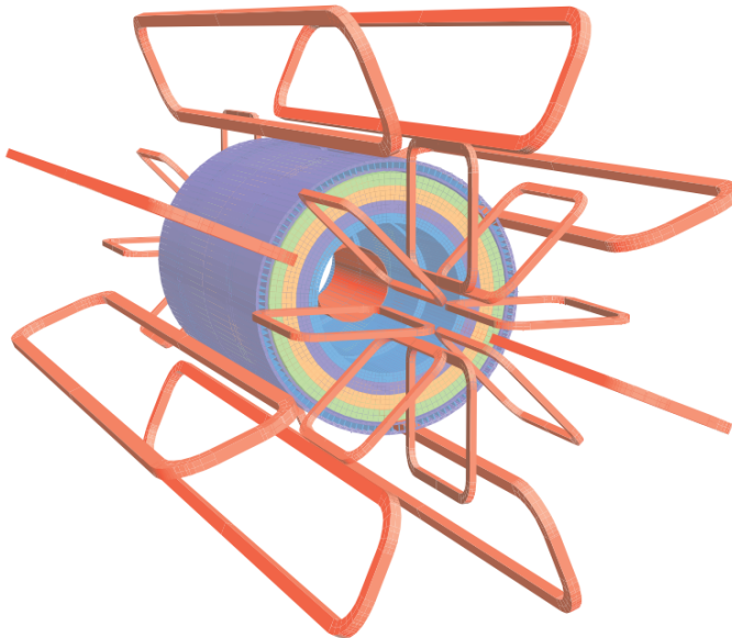
FIGURE 3.9. Schematic of the windings of the ATLAS magnet[38].
