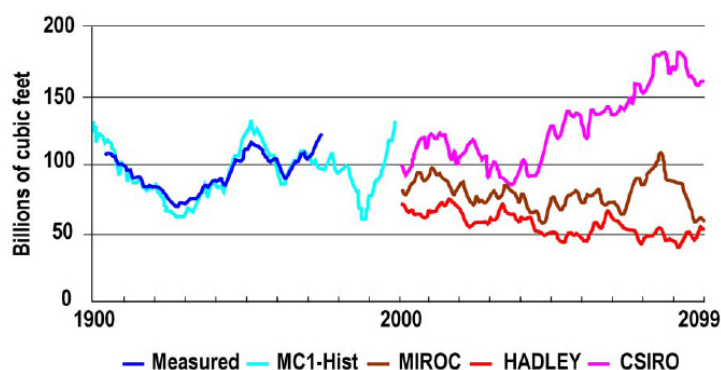
FIG 5. ANNUAL STREAM FLOW AT A SINGLE STREAM GAUGE (GOLD REY) IN THE ROGUE BASIN, WITH AN 11 YEAR FILTER. HISTORICAL STREAM FLOW IS SHOWN BASED ON HISTORICAL DATA (DARK BLUE) AND MODELED (LIGHT BLUE). PROJECTED STREAM FLOW IS GIVEN BASED ON THREE DOWNSCALED GLOBALCLIMATE MODELS.
