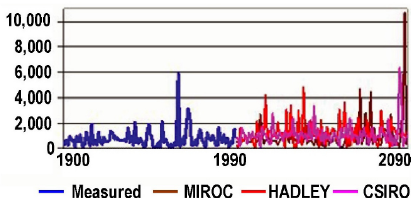
FIG 6. HISTORIC AND PROJECTED ANNUAL BIOMASS CONSUMED BY FIRE IN GIGATONS
