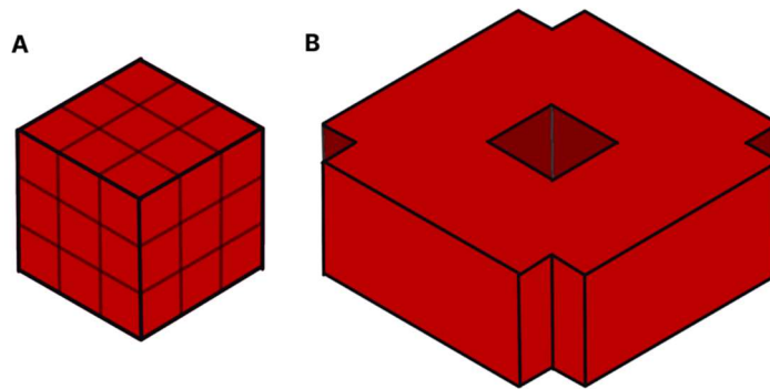
Figure 3. (A) The 3 \times 3 \times 3 test cube. (B) The 3 \times 8 \times 8 test torus.
