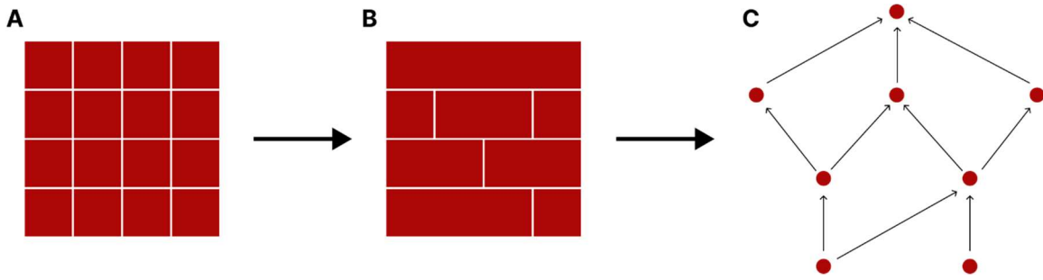
Figure 1. (A) A sample 2D square for allocation. (B) A shape configuration for the grid (layers are horizontal, connections between blocks are vertical overlaps). (C) The shape configuration represented as a directed graph with nodes representing blocks and edges representing block connections.
