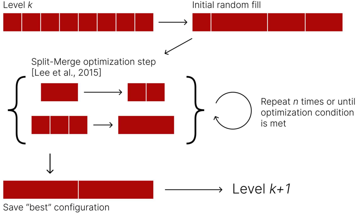
Figure 2. Steps of the evolutionary model for generating level k .
