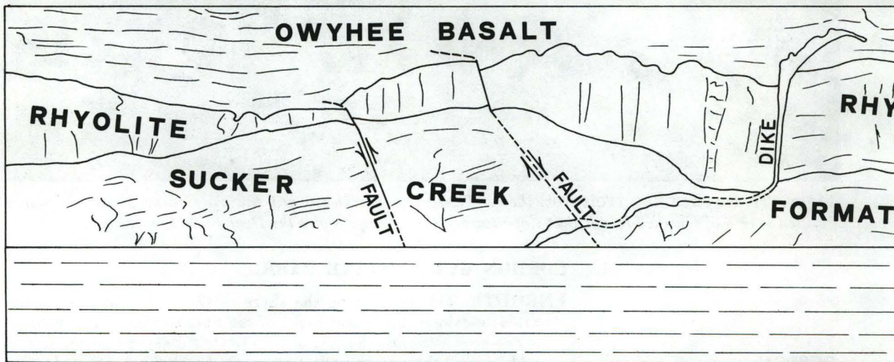
Figure 28. Ledge of rhyolite across from McCormack State Park is cut by a fault that moved it downward on the right. The structure is interpreted in the accompanying diagram.
