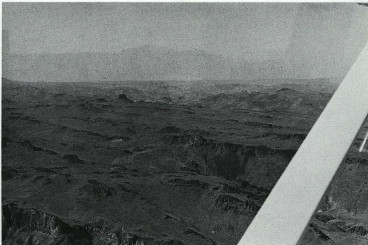
Figure 33. Three Fingers Butte, at the left of center in the middle distance, is a rhyolitic volcanic neck perched upon Owyhee Ridge. The ridge itself is Jump Creek Rhyolite, broken by faulting into many sharp ribs that run horizontally across the picture. This aerial view is southwestward from a point nearly above Stop 5.
