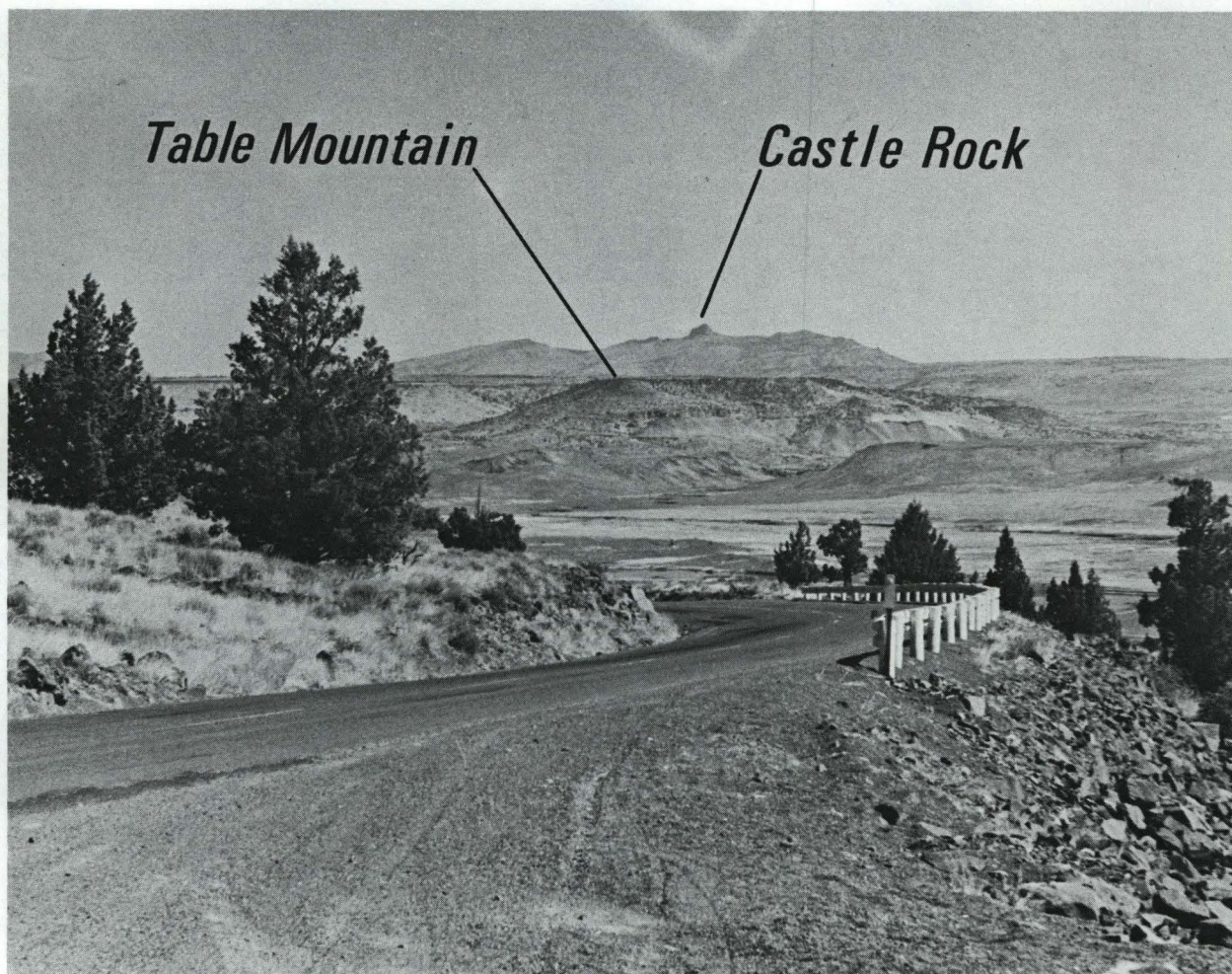
Figure 4. Western Juntura Basin seen from Stinking Water Mountain . Castle Rock is thought to have been the source of the Dinner Creek Ash-Flow Tuff .
