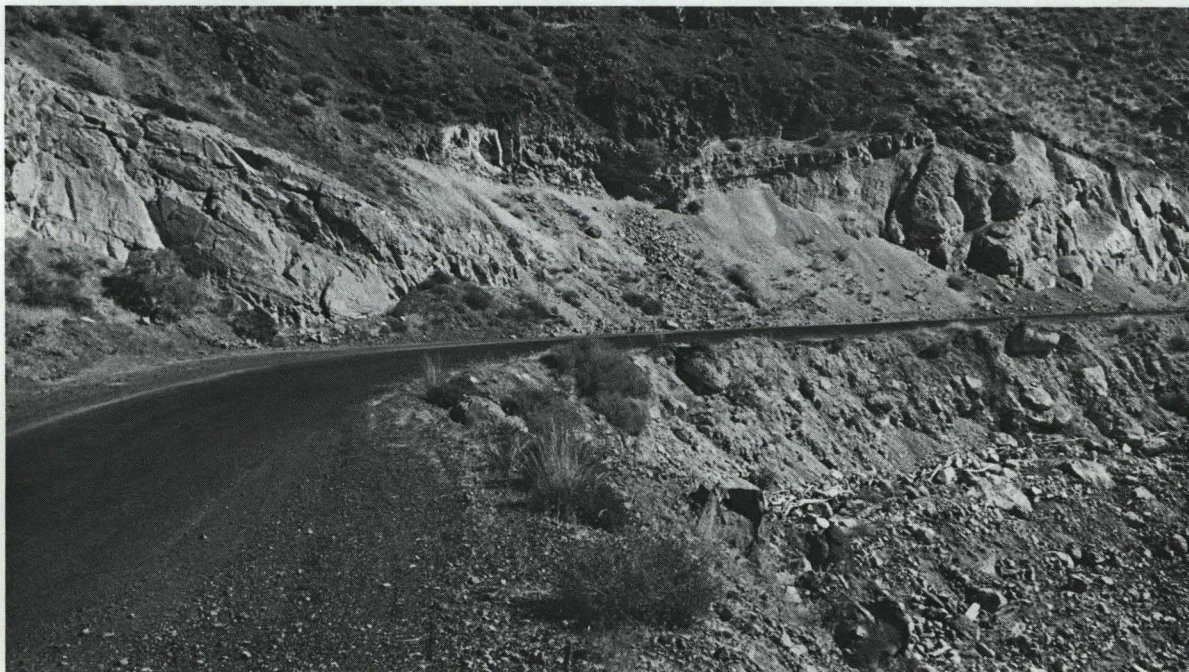
Figure 24. Owyhee Basalt overlies Sucker Creek Formation near Owyhee Dam. The distinct line of contact between the two formations is seen here just above the road.
