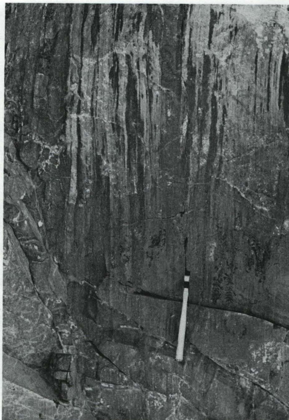
Figure 20. Vertical flow-layering in rhyolite near the right abutment of Owyhee Dam suggests that this is part of the pipe through which the molten rock rose.
