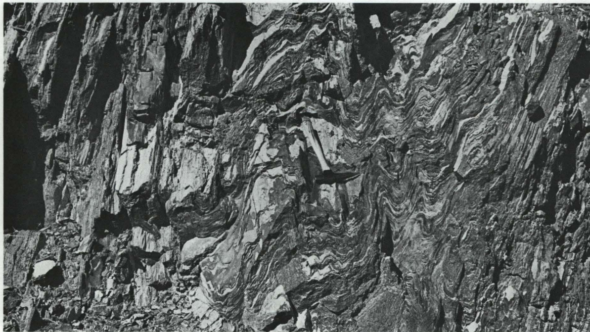
Figure 19. The Eggbeater, a structure of contorted, flow-layered rhyolite near Owyhee Dam.
