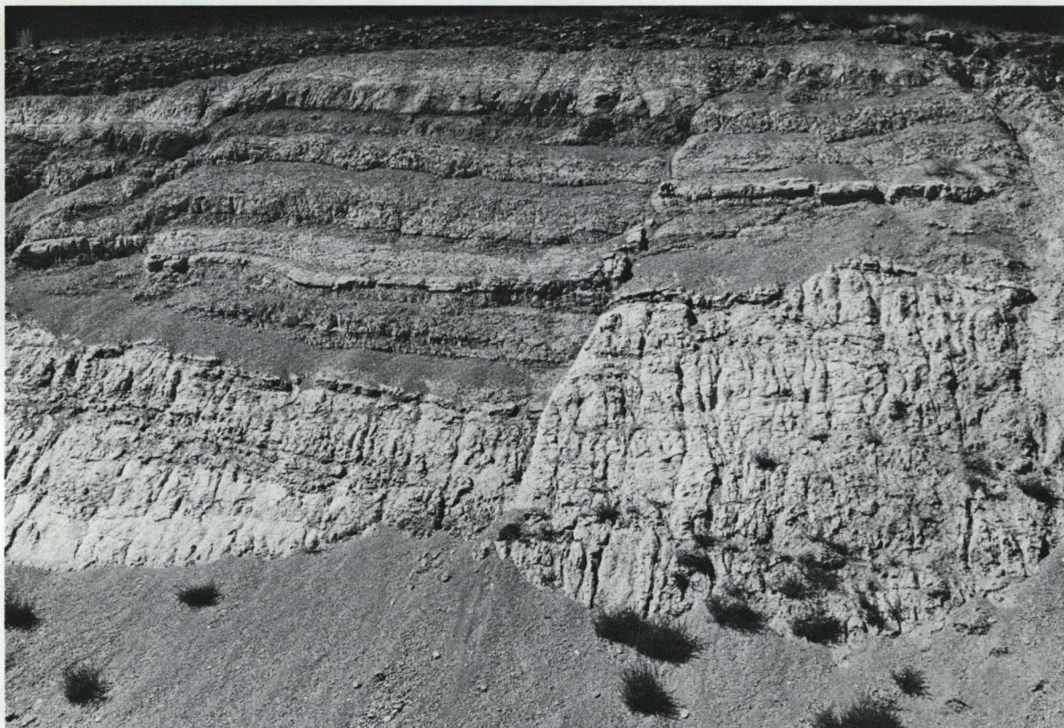
Figure 6. A minor fault in the Juntura Formation at Drinkwater Pass. The layers on the left have moved down in relation to those on the right.
