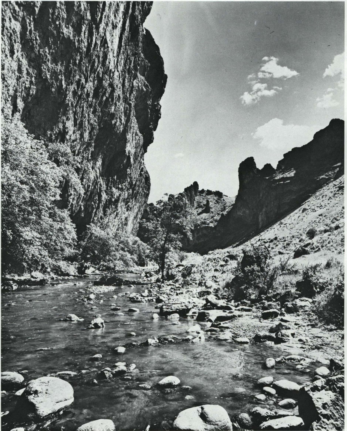
Figure 35. Overhanging cliff deep within Succor Creek Gorge. The rock is Leslie Gulch Ash-Flow Tuff. [Photograph by Oregon Highway Division]
