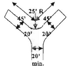
"Y" Turnaround
