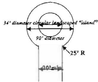
Cul-de-Sac Turnaround
