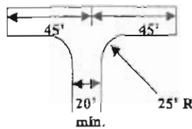
"T" Turnaround
