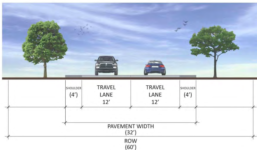
Exhibit 7-1. Rural Arterial Street Cross-Section
