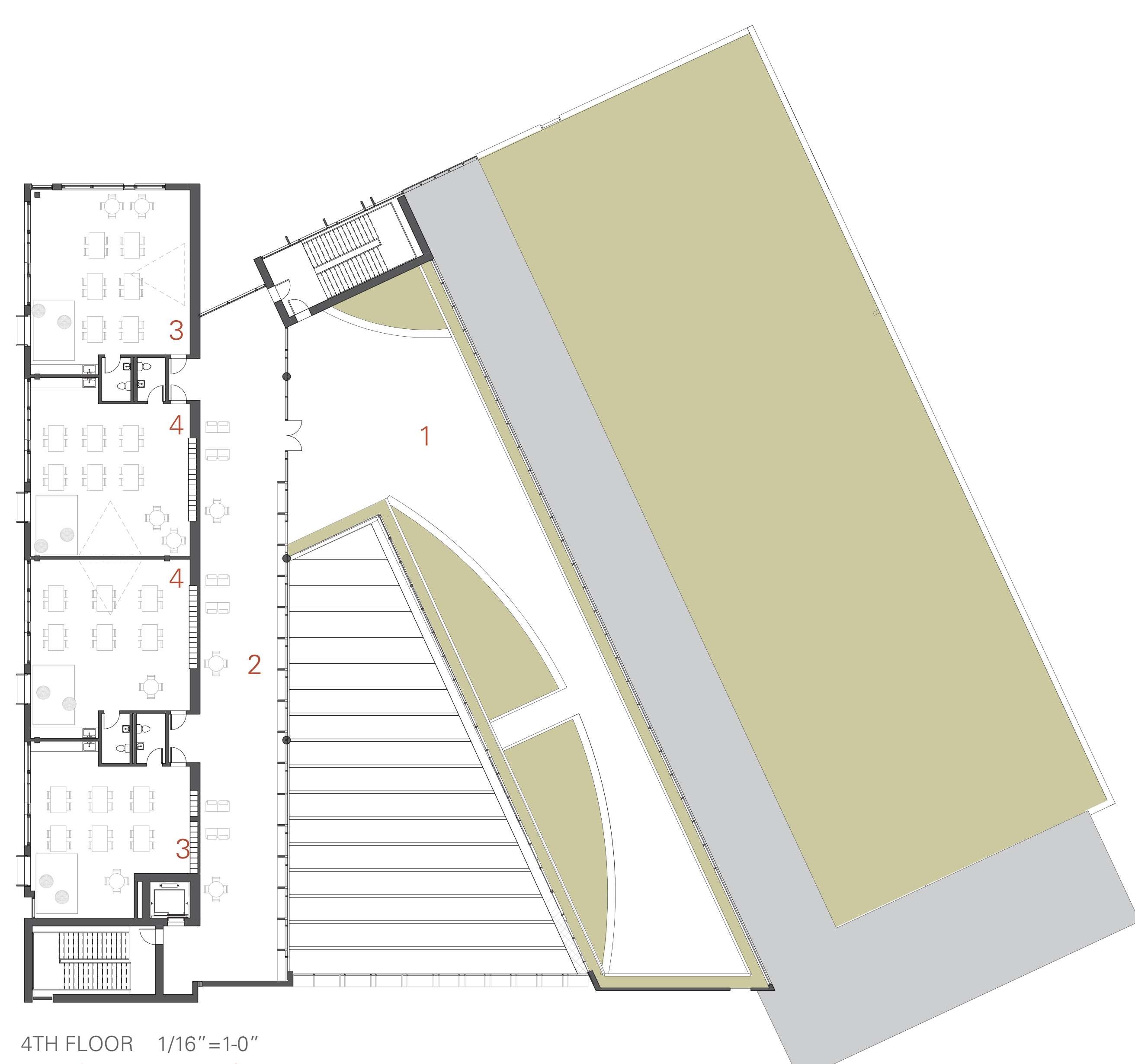
4TH FLOOR 1/16"=1'-0" 1. Roof Top Playspace/ Growing Lab 2. Collaboration Space 3. Kindergarten Classrooms 4. First Grade Classrooms
