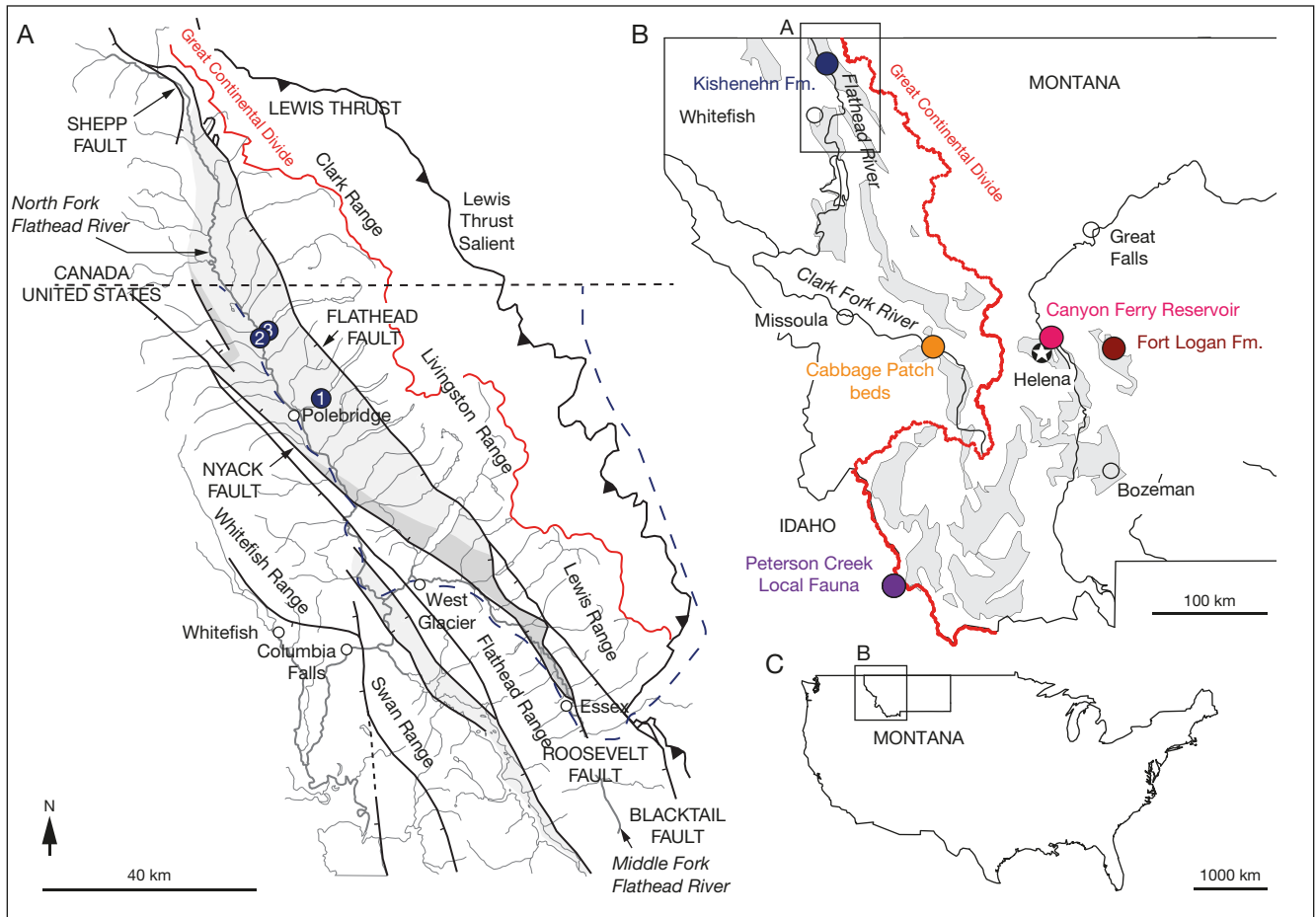
FIG. 1. — Geographic context of the Oligocene-aged fossils from Glacier National Park: A , detailed map of the Kishenehn basin showing the North Fork and Middle Fork areas, faults in the area (continuous black lines), continental divide (red), national park boundaries (dashed blue line), and water courses (gray). Localities of GLAC 26988 (1), GLAC 26987 (2), and CM 87801 (3) are also showed (modified from Dawson & Constenius 2018). Detailed geographic information is available to qualified researchers from repositories; B , map of western Montana showing the location of five coeval Arikarean-aged deposits bearing leptomerycid and/or equid fossils: the Kishenehn, Renova (Cabbage Patch beds), and Fort Logan formations as well as the Canyon Ferry Reservoir and the Peterson Creek Local Fauna (in Idaho). Select water bodies, cities, and the continental divide are also displayed. Grey areas represent basins with strata coeval with the Kishenehn Formation. Black box shows location of A; C , location of the state of Montana within the United States with black box showing location of B.
