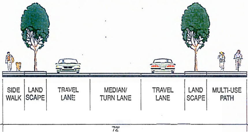
Lochner Multi-Use Trail Cross Section
