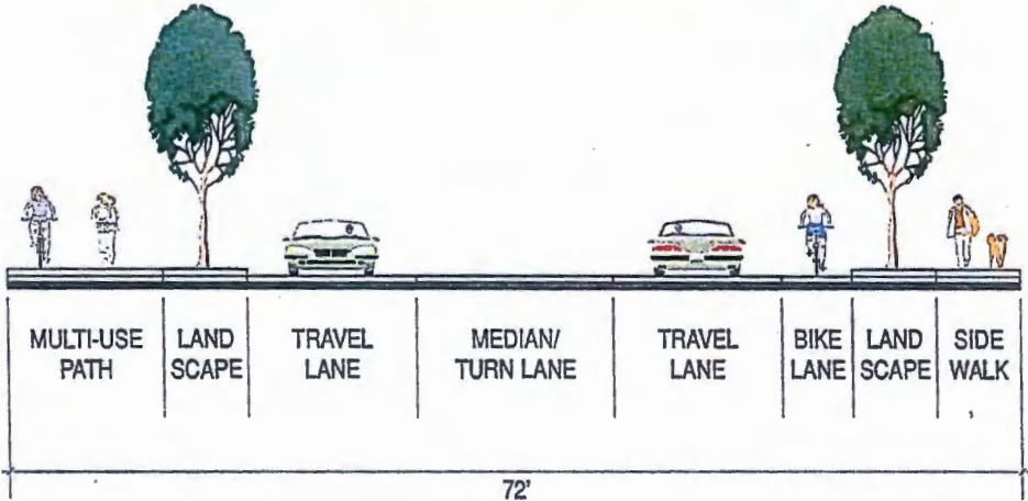
Columbus Multi-Use Trail Cross Section
