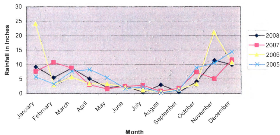
Figure 6. Precipitation Patterns for the North Coast 2005-2008
