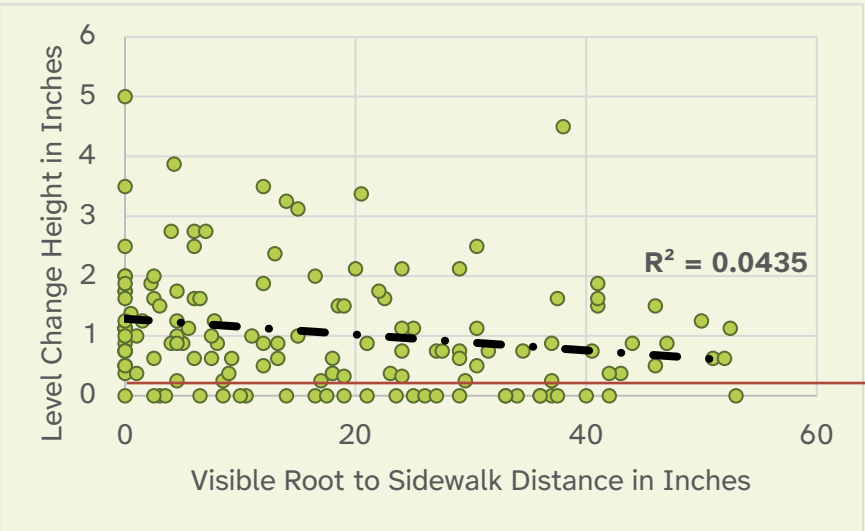
Figure 2.4.30 Relationship between Level Change Height and Root to Sidewalk Distance Scatterplot showing the relationship between the maximum level change height within tree canopy and the distance from the nearest roots to the sidewalk edge.
