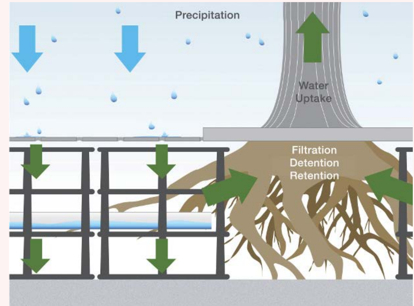
Figure 1.3.12 Root Accommodating Subgrade Construction
