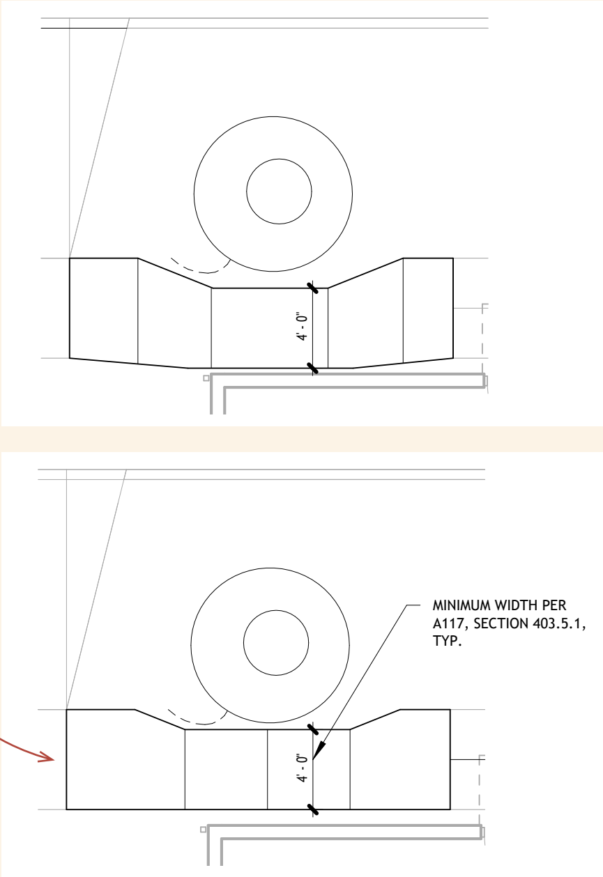
Figure 3.3.9 Possible Scalloped Walk Options for Repairing the Sidewalk within the Current System - Redlined Post Analysis Drafted plans of ways to scallop the sidewalk illustrated January 2026 while waiting to hear the determined fate of the Majestic Maple with redlines added after data analysis.
