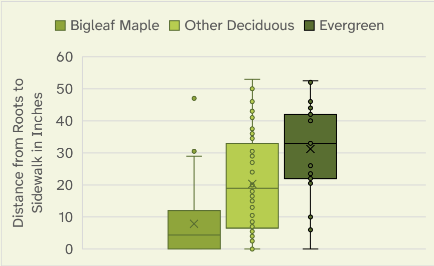
Figure 2.4.29 Distance from Roots to Sidewalk by Species Category Box and whisker charts showing the common distance ranges between the nearest visible roots/burls and the adjacent pavement by species category.
