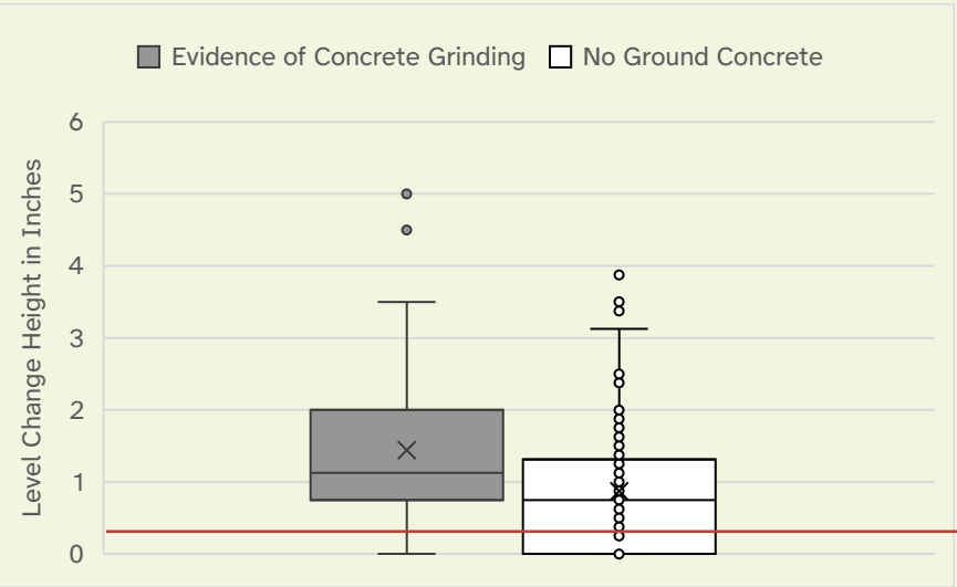
Figure 2.4.11 Accessibility of Sidewalks with and Without Evidence of Concrete Grinding Box and Whisker Chart showing the height of level changes at sites with vs. without signs of concrete grinding, showing that sites with concrete grinding had notably higher level changes.
