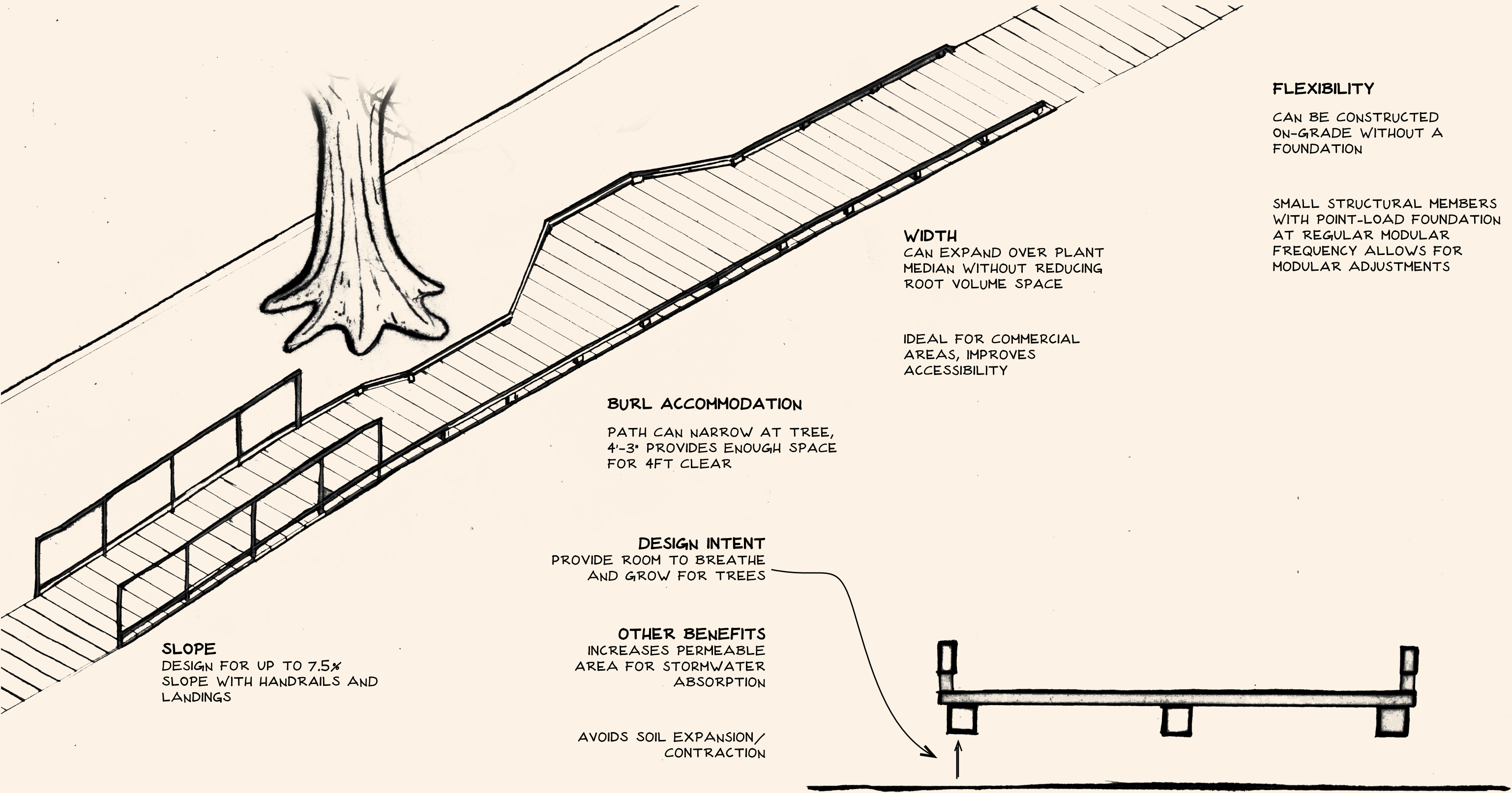
Figure 3.4.3 Potential for Expansion Illustration of ways WhitWalks could expand and be modified to elevate sidewalks at various sites.
