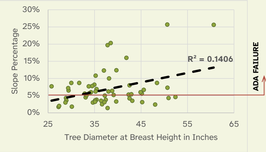
Figure 2.4.24 Relationship between Slope Within Canopy and Tree DBH for Bigleaf Maple Scatterplot showing the relationship between trunk diameter at breast height and measured maximum slope within tree canopy.
