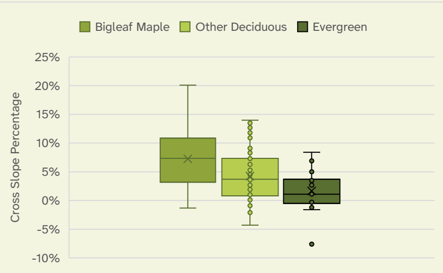
Figure 2.4.17 Difference in Max Slope In - Outside Canopy Box and whisker charts reflecting the difference in slope within vs. outside the tree canopy by species category.
