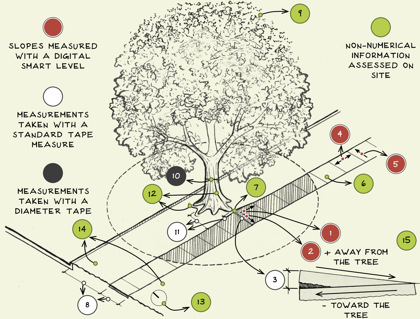
Figure 2.3.1 Methods Isometric drawing of the measurements taken at each site.
