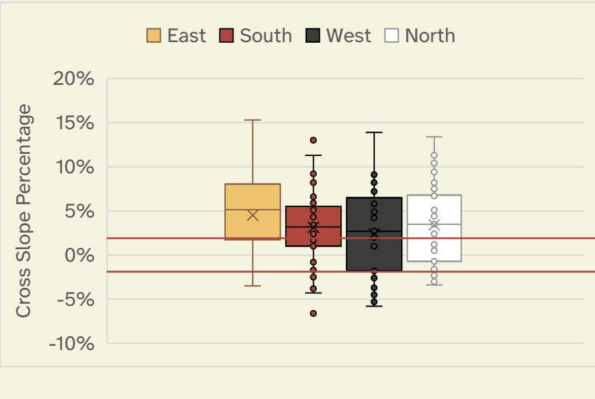
Figure 2.4.34 Maximum Cross Slope by Relative Sidewalk Direction Box and whisker chart reflecting the range of maximum cross slopes measured at all sites within the research scope divided by the direction of the sidewalk relative to the tree.
