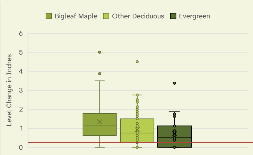
Figure 2.4.18 Level Change Height by Species Category Box and Whisker chart illustrating the common range of level height by species category.
