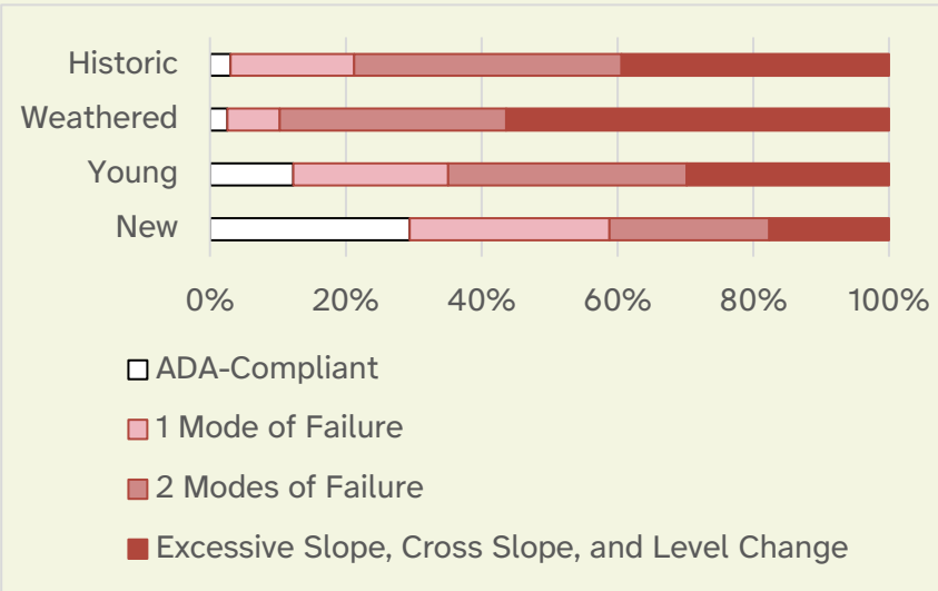
Figure 2.4.7 Number of Modes of Failure by Estimated Sidewalk Age 100% Stacked horizontal bar chart reflecting the number of modes of path failure at sites with sidewalks estimated to be new, young, weathered, or historic.
