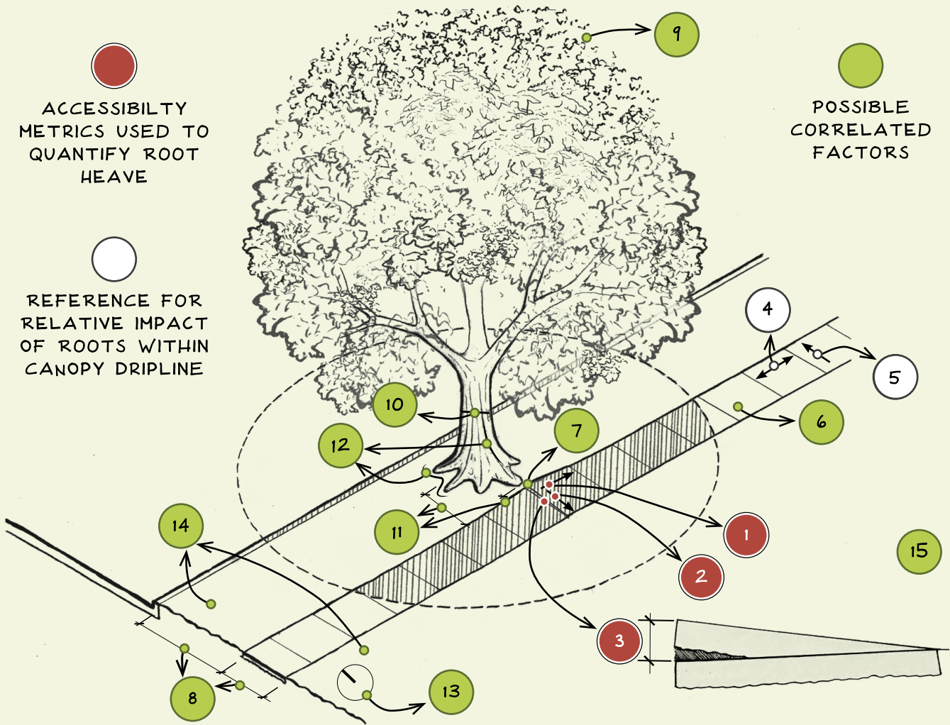
Figure 2.1.2 Hypotheses Isometric drawing of a street tree indicating a focus on the relationship between the base of the tree and the sidewalk.
