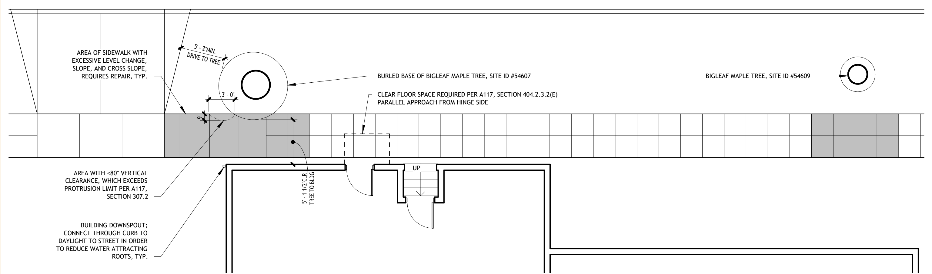
Figure 3.4.8 Conditions Measured in the Field Drafted plan illustrating existing conditions surrounding the trees at this site.
