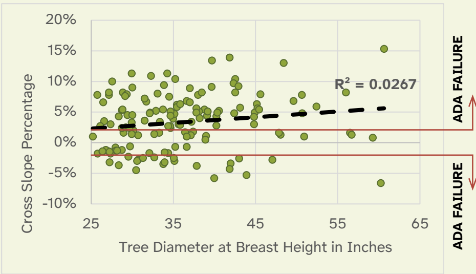
Figure 2.4.21 Relationship between Cross Slope Within Canopy and Tree DBH Across All Species
