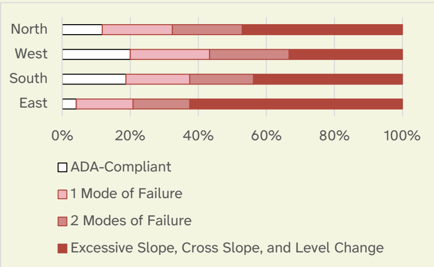
Figure 2.4.35 Modes of Failure by Relative Sidewalk Direction 100% horizontal stacked bar chart showing the number of modes of failure found at sidewalks across all sites within the research scope by the direction of the sidewalk relative to the tree.
