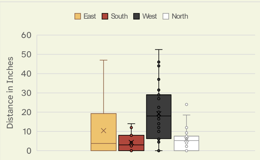
Figure 2.4.33 Distance from Roots to Sidewalk by Direction - Bigleaf Maples Box and whisker chart showing the ranges of root-sidewalk distance measured across all Bigleaf Maples within the research scope divided by the sidewalk's location relative to the tree.
