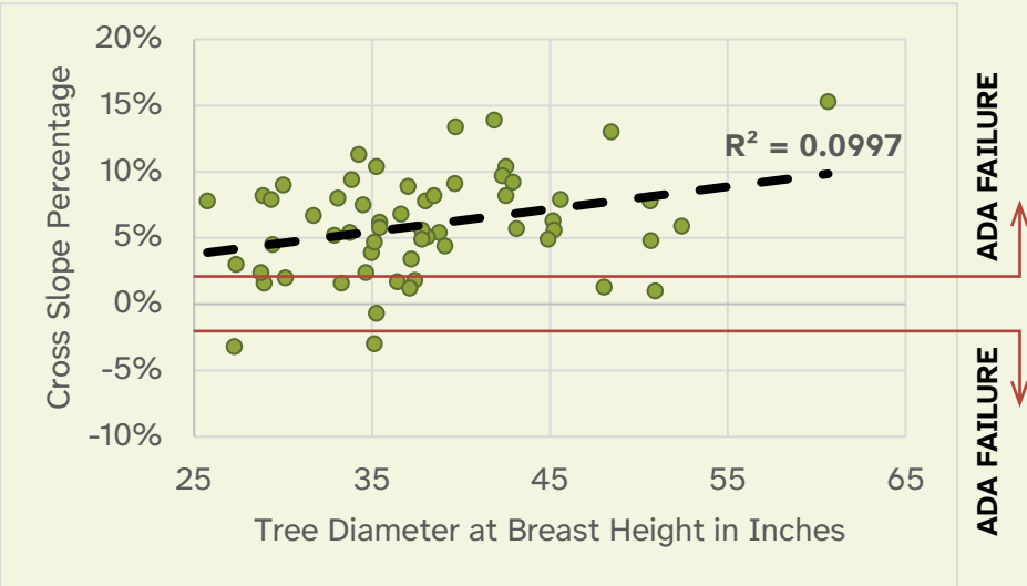
Figure 2.4.25 Relationship between Cross Slope Within Canopy and Tree DBH for Bigleaf Maple Scatterplot showing the relationship between trunk diameter at breast height and measured maximum cross slope within tree canopy.
