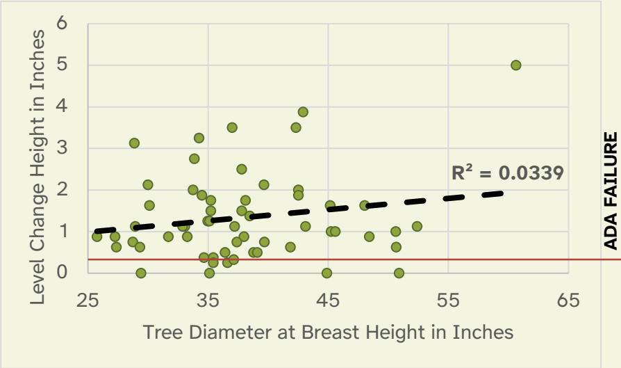
Figure 2.4.26 Relationship between Level Change Height and Tree DBH for Bigleaf Maple Scatterplot showing the relationship between trunk diameter at breast height and measured maximum level change height within tree canopy.
