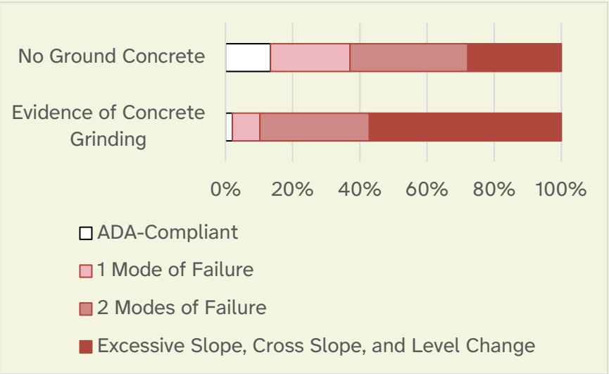
Figure 2.4.12 Accessibility of Sidewalks with and Without Evidence of Concrete Grinding 100% Stacked horizontal bar chart showing the accessibility of sidewalks with vs. out concrete grinding showing that sites with evidence of concrete grinding had substantially more accessibility failures.
