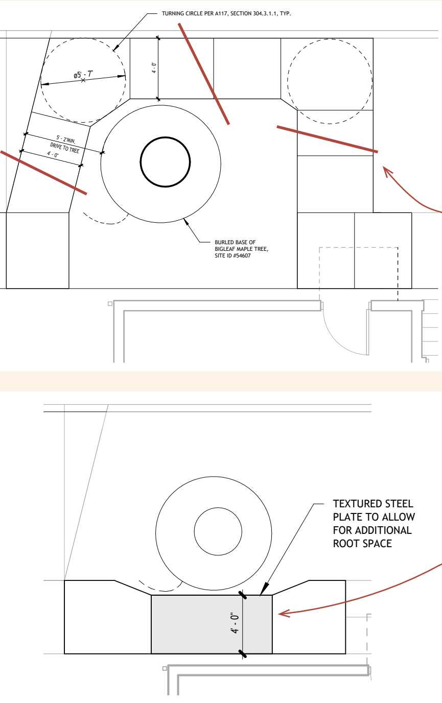
Figure 3.3.10 Theorized Radical Sidewalk Renovation Options- Redlined Post Analysis Drafted plans of potential radical sidewalk changes illustrated January 2026 while waiting to hear the determined fate of the Majestic Maple with redlines added after data analysis.
