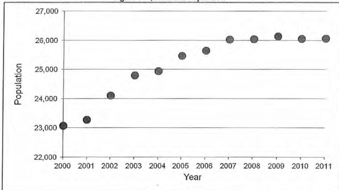
Figure 3-2 | Historical Population
