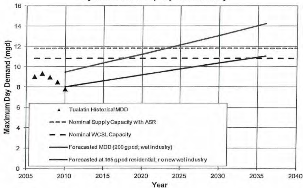
Figure 5-4 | Source Capacity Needs Summary
