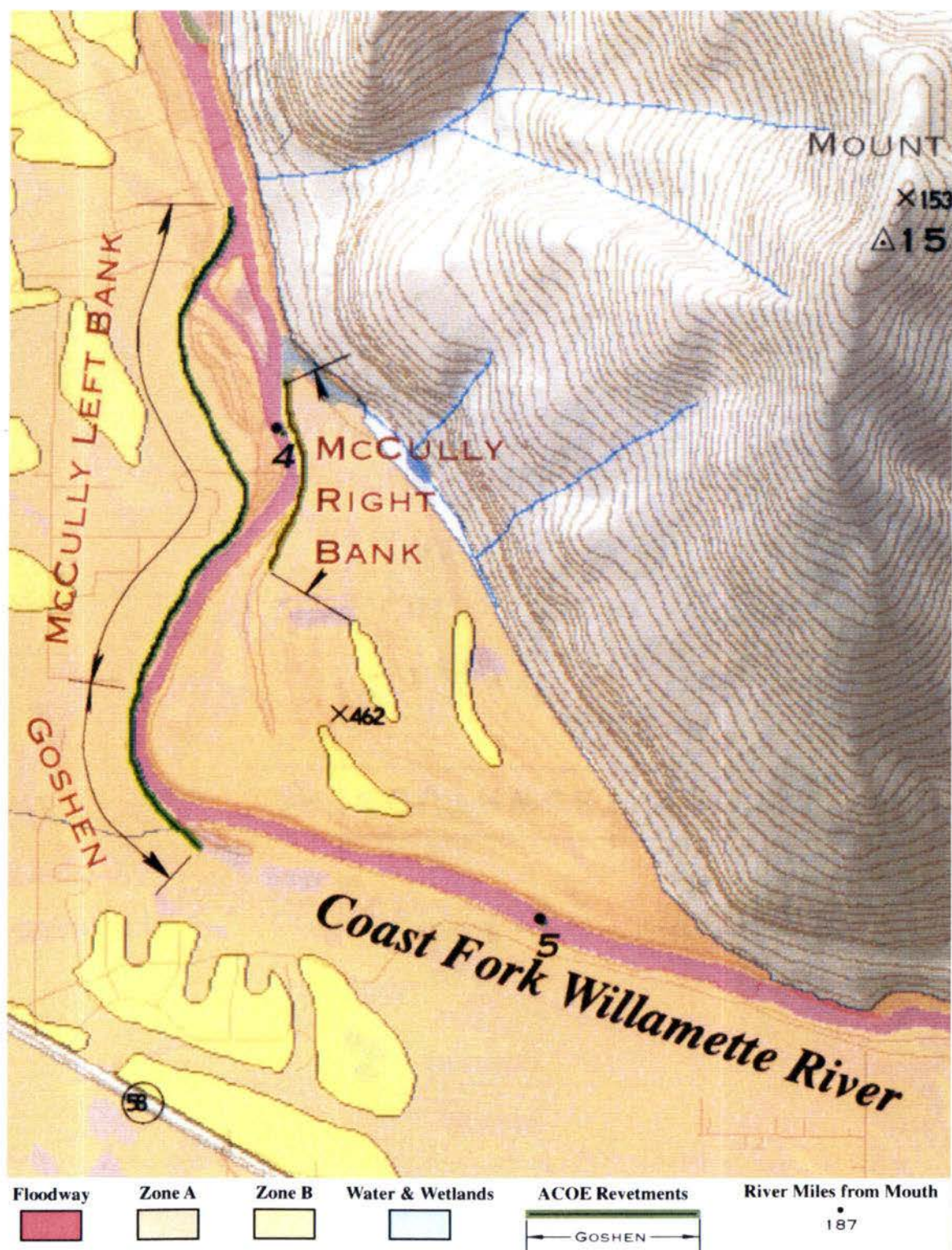
Figure 5. Federal Emergency Management Agency floodplain map of the South Meadow (the colored area east of the river). Zones A and B are the 100-year and 500-year floodplains, respectively. Note Army Corps of Engineers revetments. Approx. scale 1:12000 (adapted from LCP/FBP 2001).
