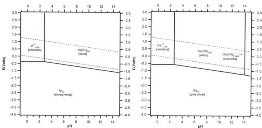
Figure 6. Pourbaix diagrams for indium (left) and gallium (right). 20
