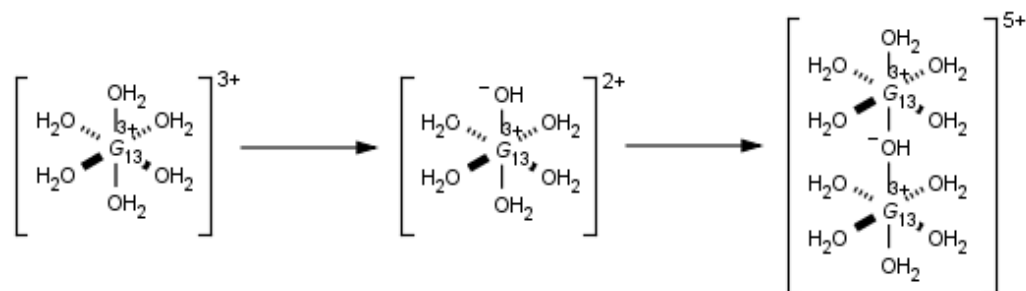
Figure 8. Proposed intermediaries for cluster formation.
