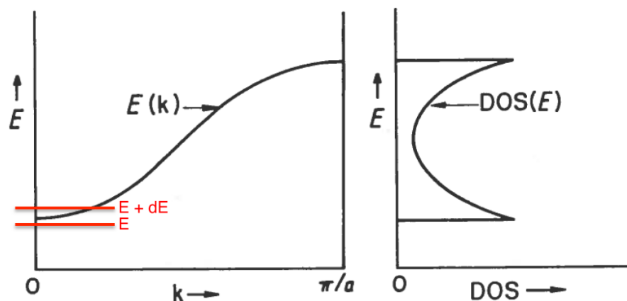
Figure 18. Band structure (left) and density of states plot (right) for the 1s orbitals of a one dimensional string of hydrogen atoms. 58
