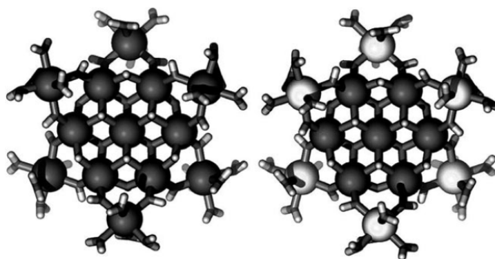
Figure 1. Structure of \text{Ga}_{13} and \text{Ga}_7\text{In}_6 nanoclusters. 19
