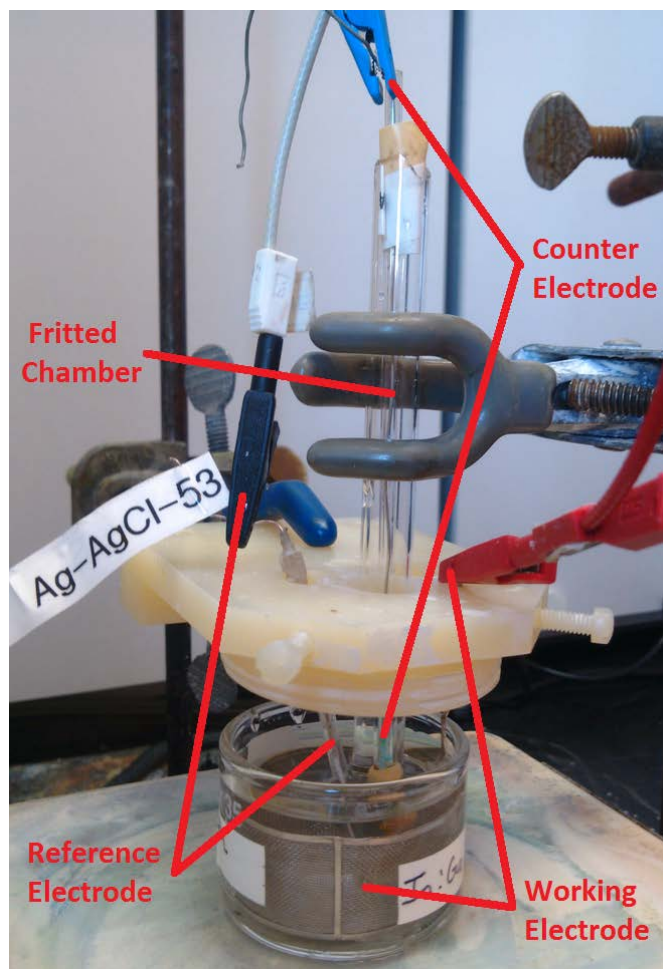
Figure 3. Picture of the electrochemical setup.
