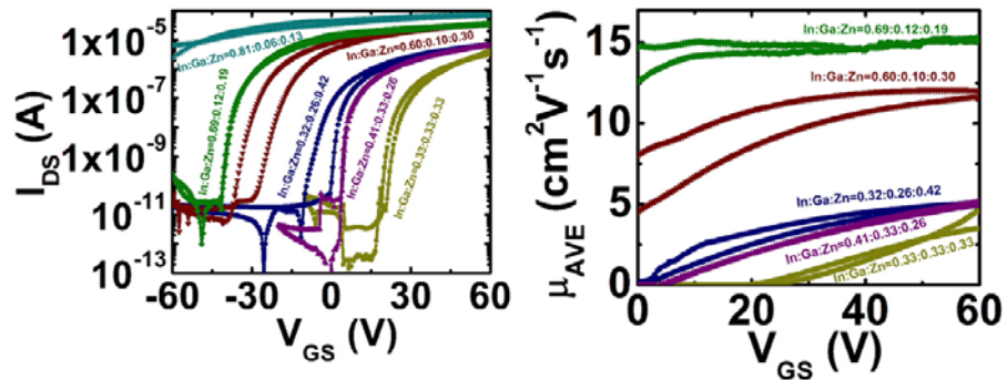
Figure 16. Transfer curve and average channel mobility plot for a range of IGZO compositions.
