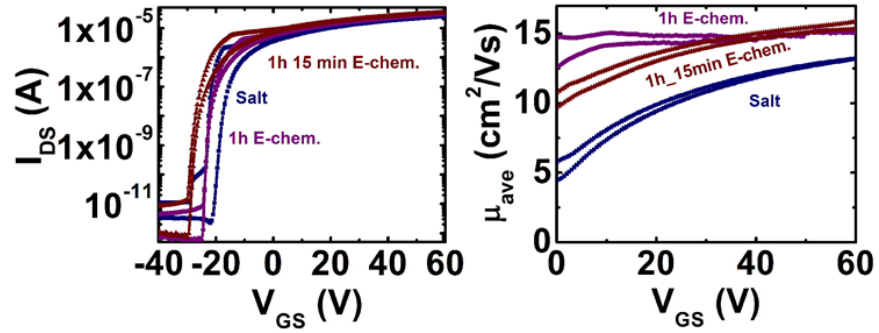
Figure 15. Comparison of electrical performance across electrolysis duration.
