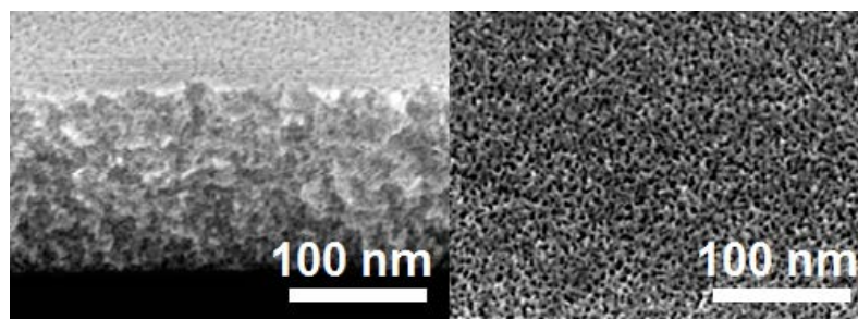
Figure 11. SEM images of IGZO films produced using the sol-gel method.
