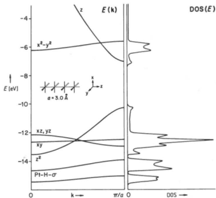
Figure 19. Band structure and DOS plots for \text{PtH}_4^{2-} atoms. 58
