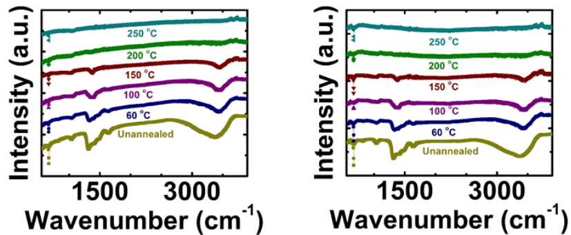
Figure 14. IR spectrums of films made using a salt solution (left) and a 1 h electrochemistry precursor (right).
