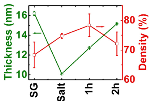
Figure 12. Results of XRR analysis.
