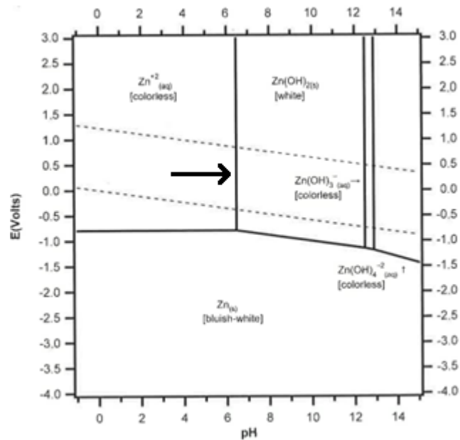
Figure 2. A Pourbeix diagram for zinc. 20
