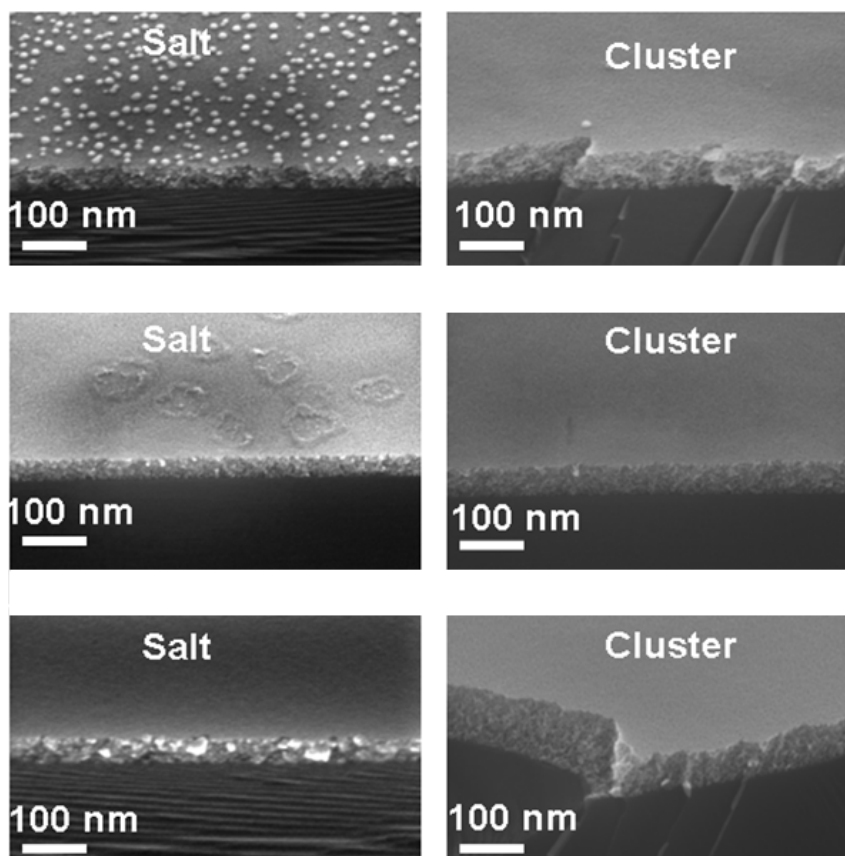
Figure 10. SEM images of IGZO films produced using electrochemical precursor.
