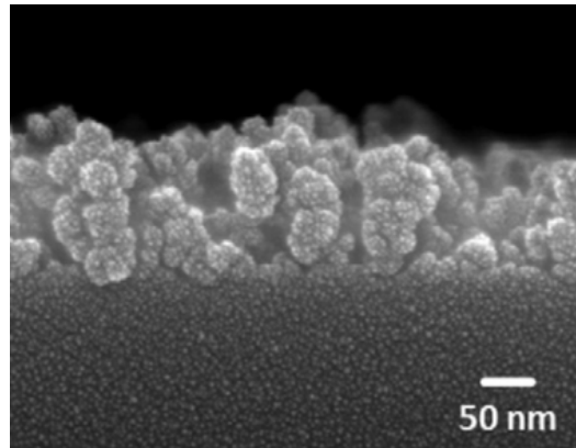
Figure 17. SEM image of IGZO produced via ELA. 36
