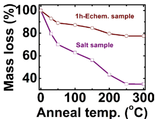
Figure 13. Results of QCM analysis.
