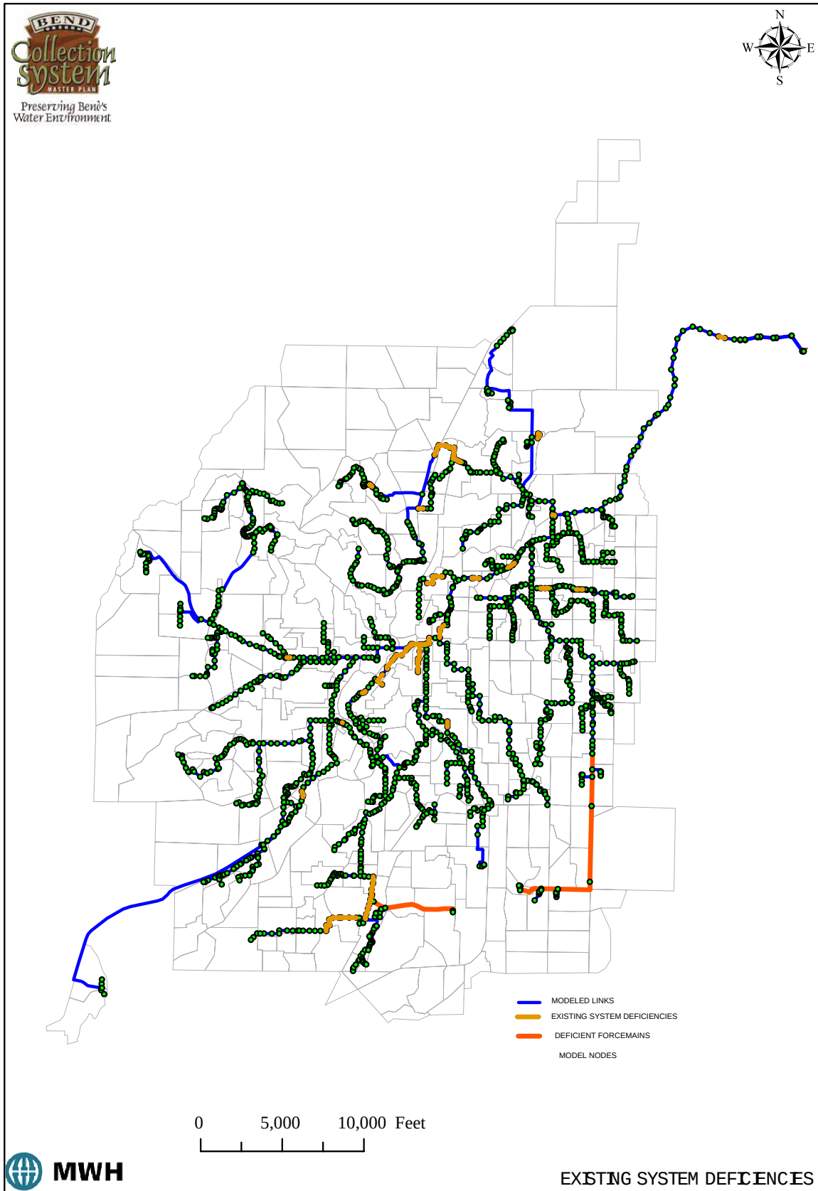
Figure 3-7 – Existing System Deficiencies
