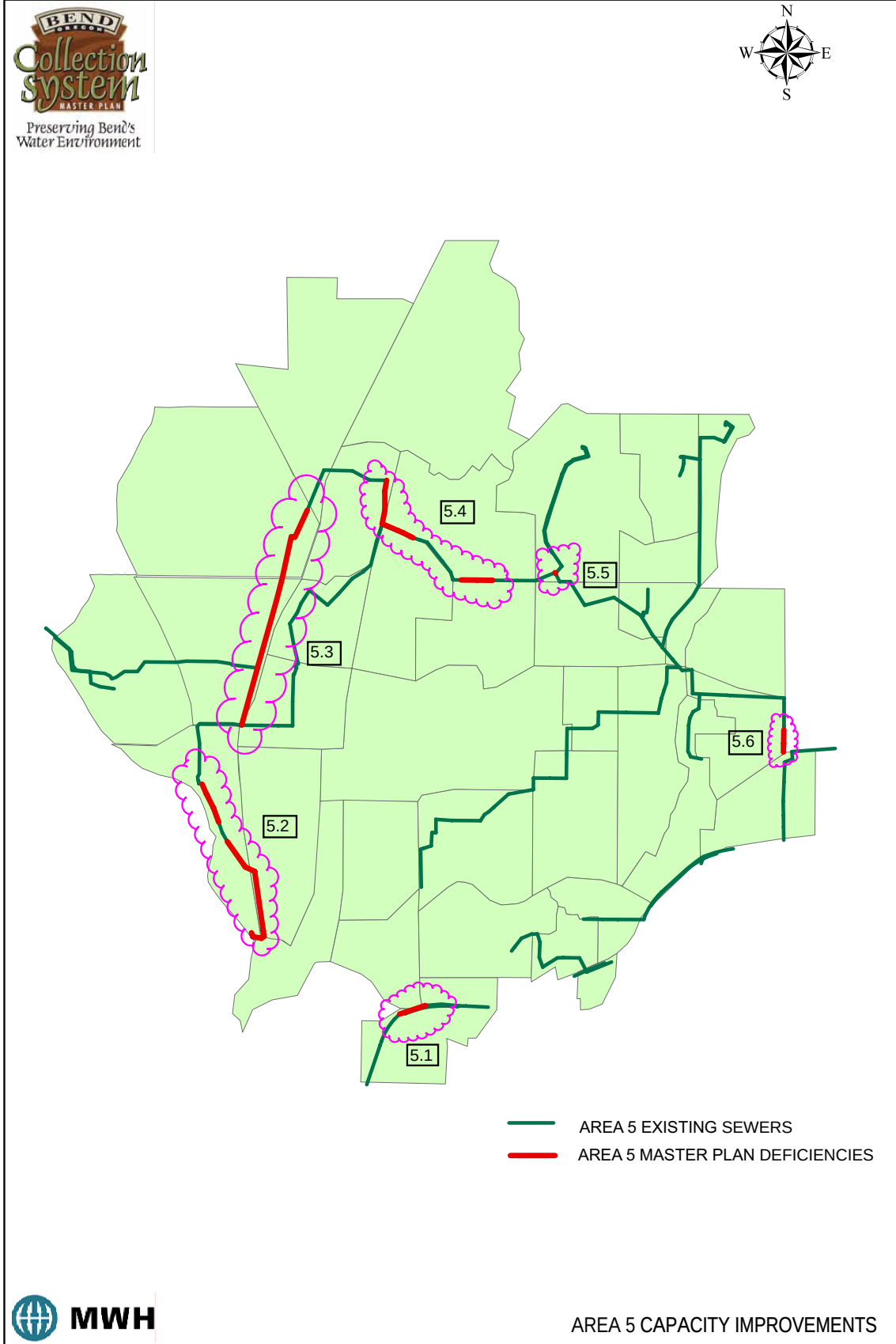
FIGURE 4-6– STUDY AREA 5 REQUIRED CAPACITY IMPROVEMENTS
