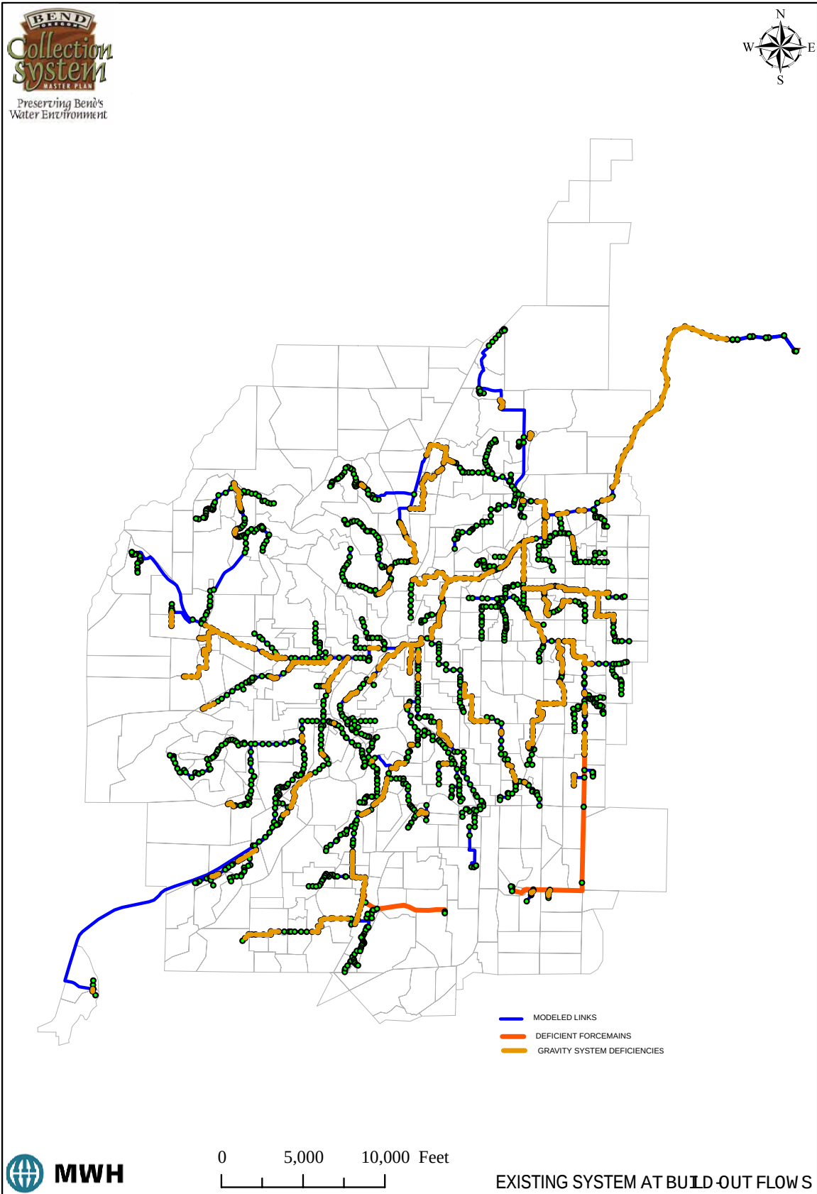
Figure 3-8 – Existing System at Build-out Flows
