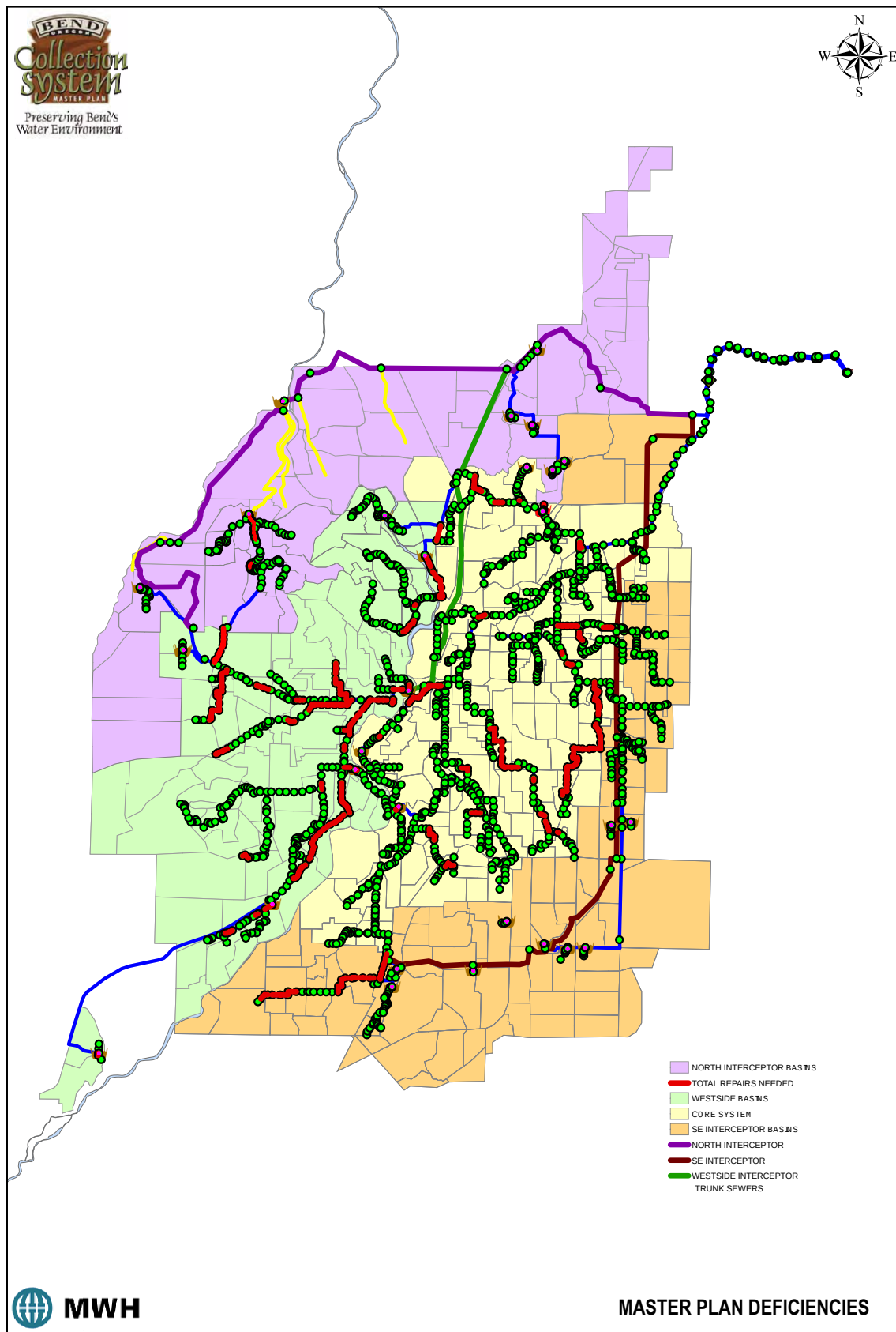
Figure 3-17 – Master Plan System Deficiencies
