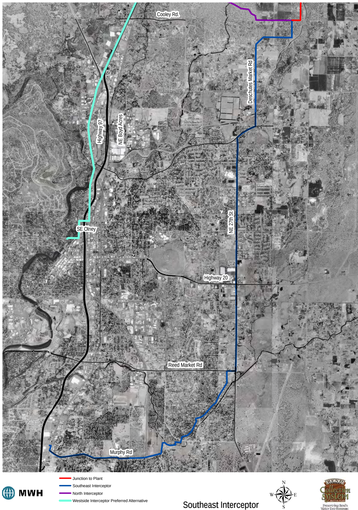
FIGURE 6-4 – SE INTERCEPTOR
