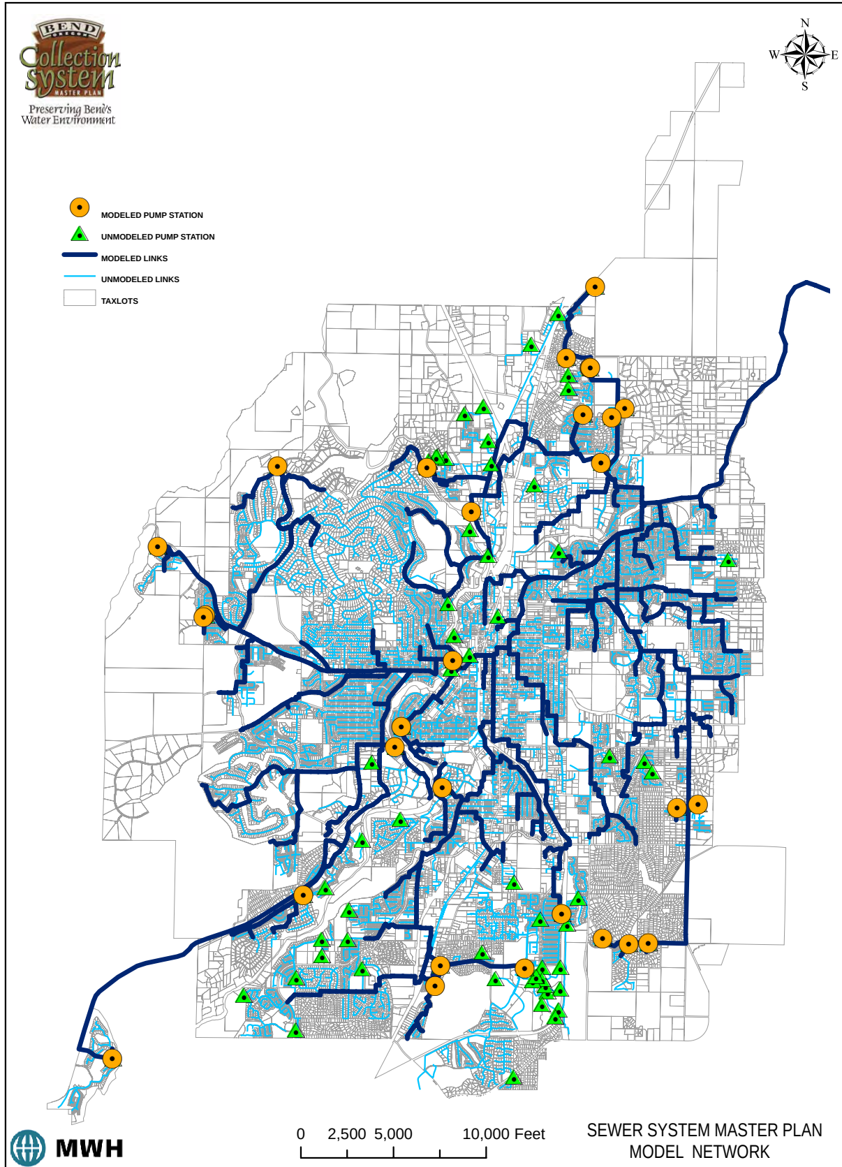
Figure 3-2 – Model Network
