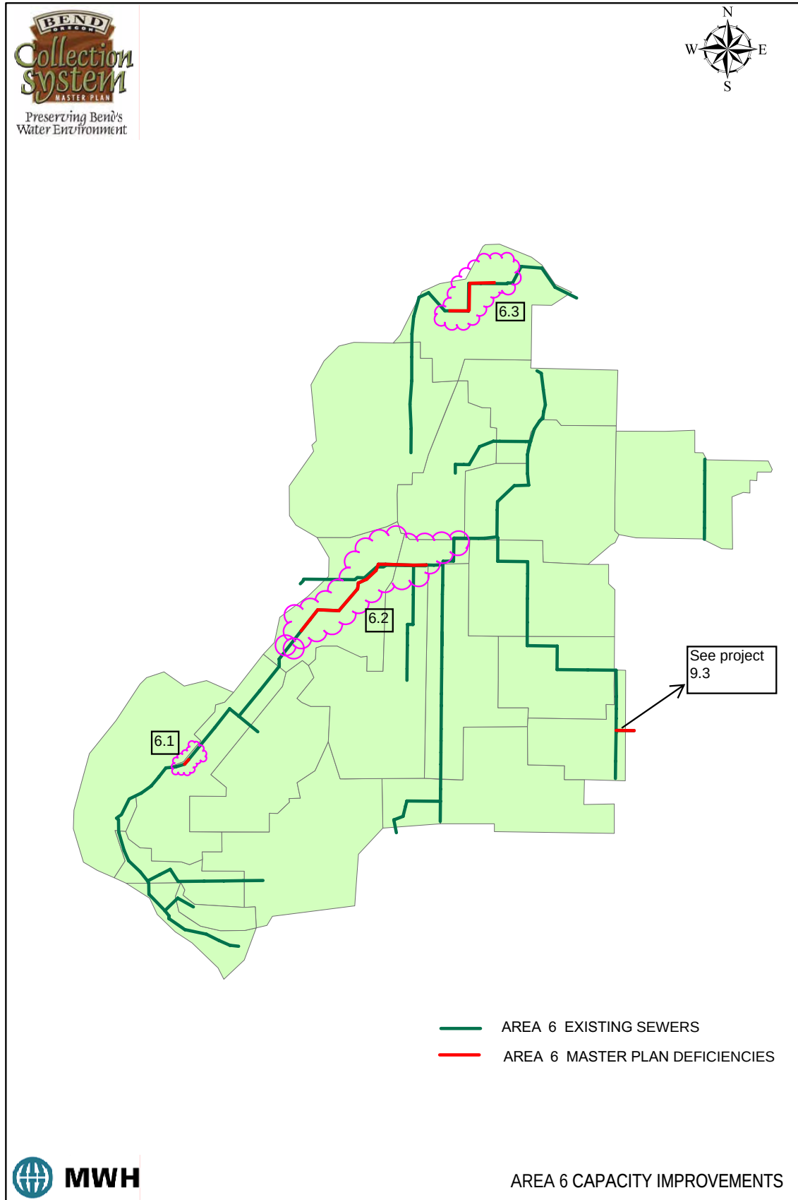
FIGURE 4-7- STUDY AREA 6 REQUIRED CAPACITY IMPROVEMENTS
