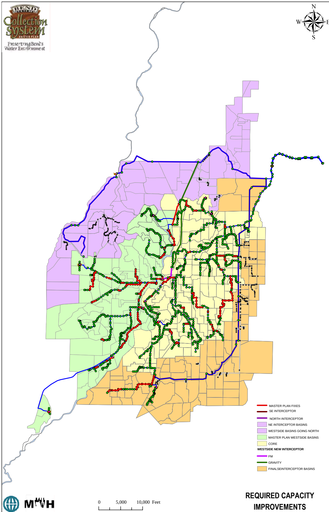
FIGURE 4-3- REQUIRED CAPACITY IMPROVEMENTS AT SYSTEM BUILD-OUT
