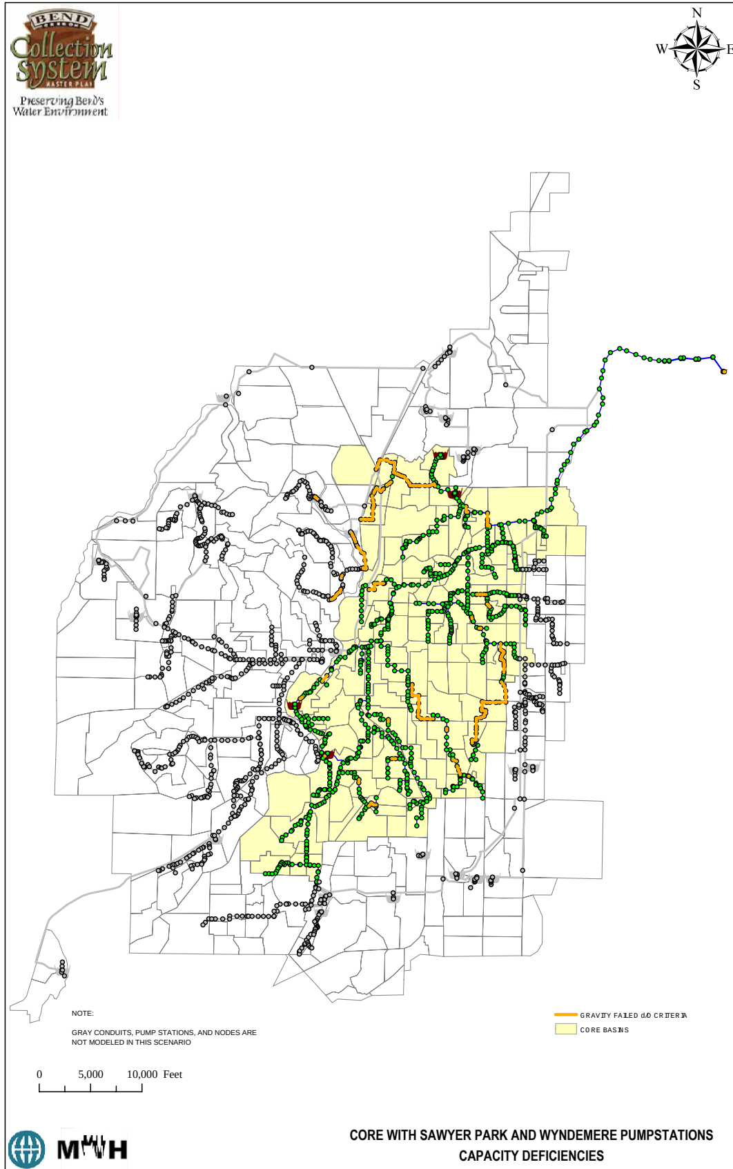
Figure 3-13 – Core System Deficiencies with Sawyer and Wyndemere Pump Stations
