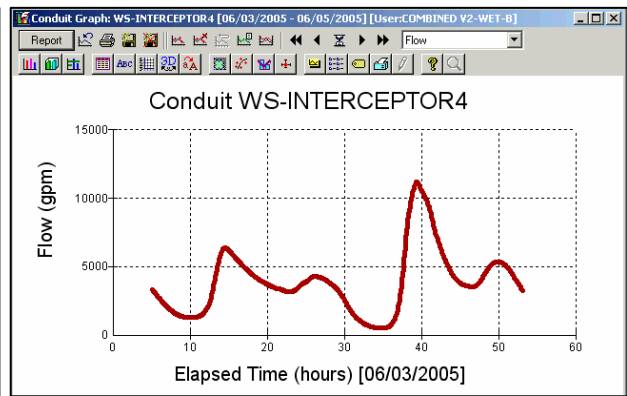
Figure 5-4: Peak wet weather flow – 10,900 - gpm
