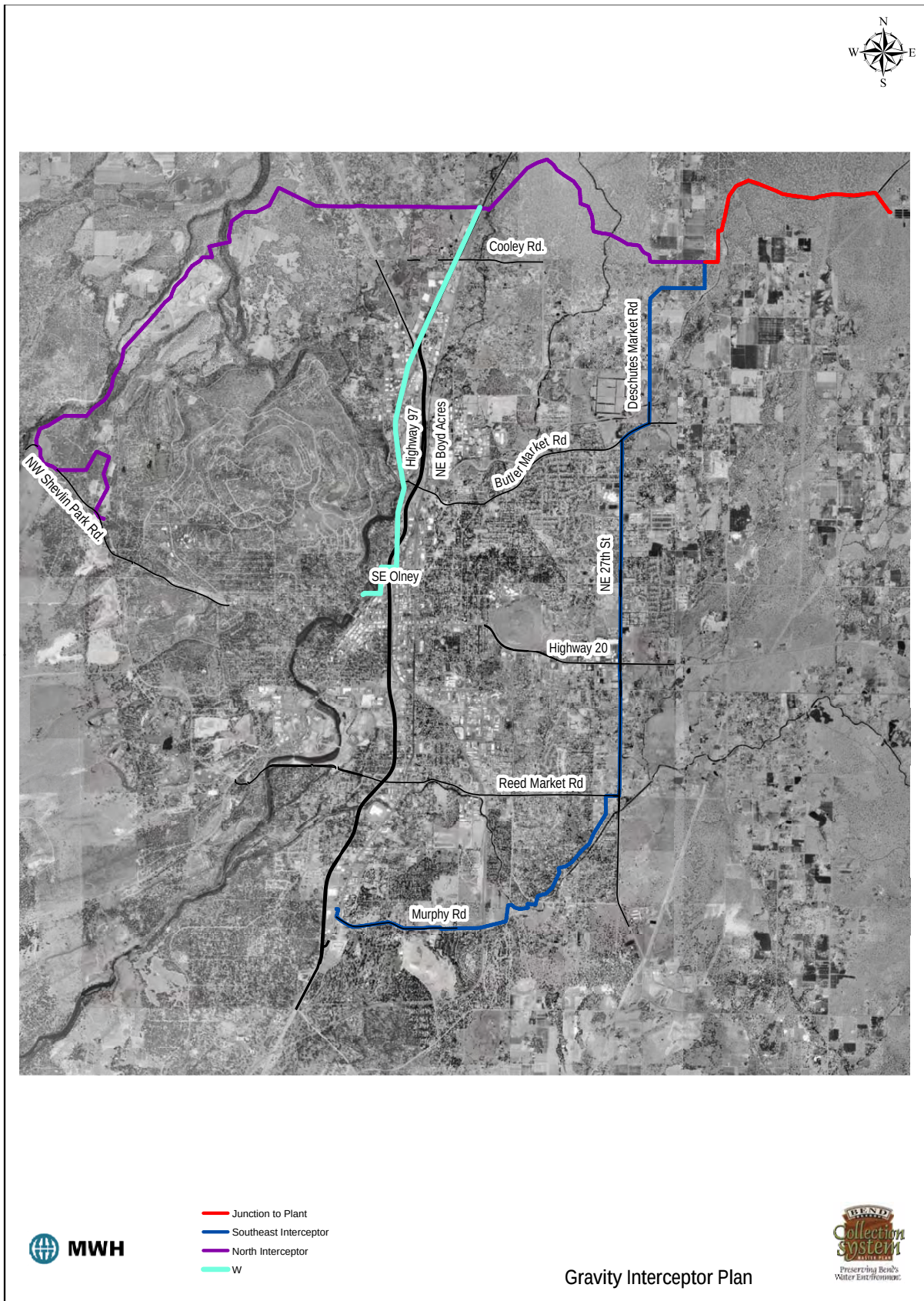
FIGURE 6-1 – INTERCEPTOR PLAN
