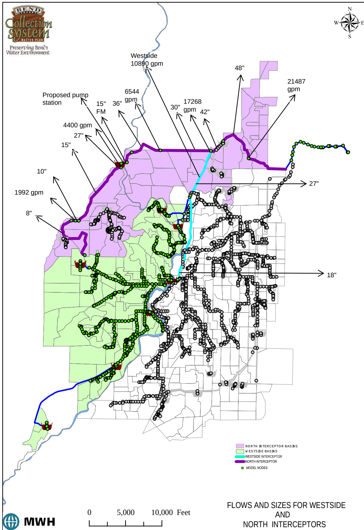
Figure 3-12 – Flows and Sizes for North and Westside Interceptors
