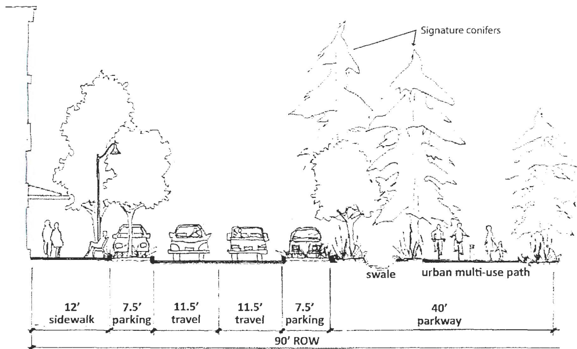
Figure 13—Typical Green Connector Street Cross-Section: Public Street
