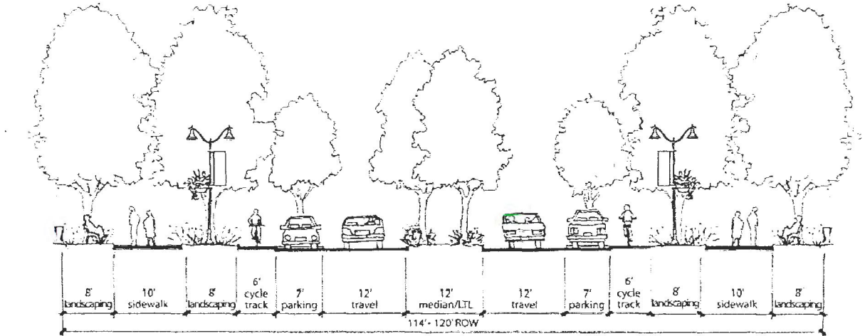
Figure 11—Typical Green Boulevard Cross-Section, NW Stucki Ave. North of NW Wilkins St to NW Cornell Road, and South of NW 194 th Ave. to LRT: Public Street
