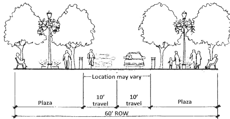
Figure 14—Typical Festival Street Cross-Section: Public Street
