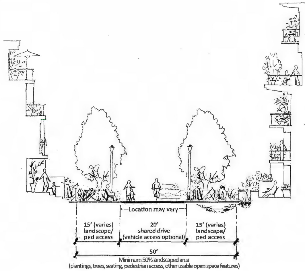
Figure 15—Typical Green Access Lane Cross-Section: Private
