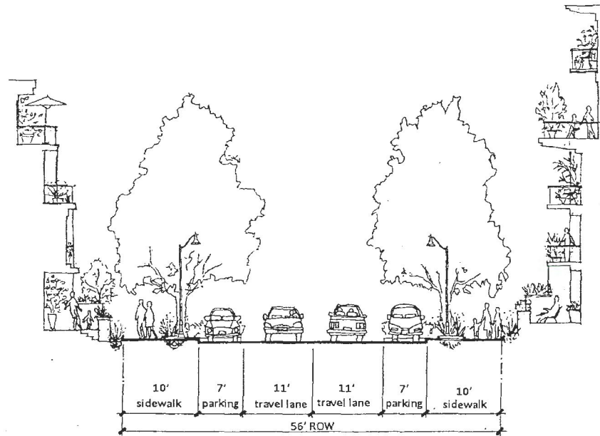
Figure 8—Typical Mixed Use Residential Street Cross-Section: Private Street
