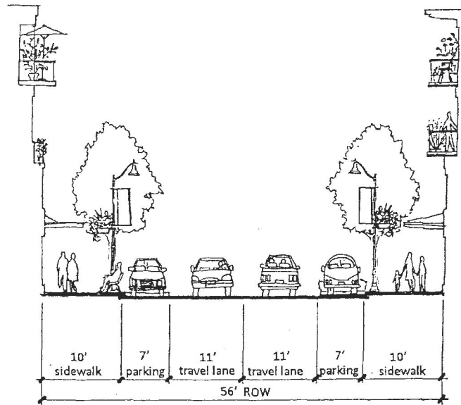
Figure 6—Typical Mixed Use Commercial Street Cross-Section: Private Street
