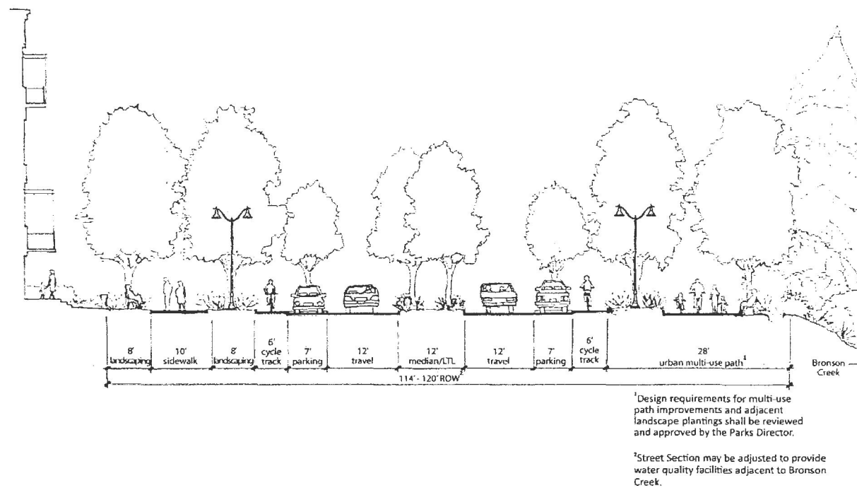
Figure 12—Typical Green Boulevard Cross-Section, NW Stucki Ave. Between NW Wilkins St. and NW 194 th Ave.: Public Street
