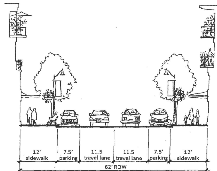
Figure 5—Typical Mixed Use Commercial Street Cross-Section: Public Street
