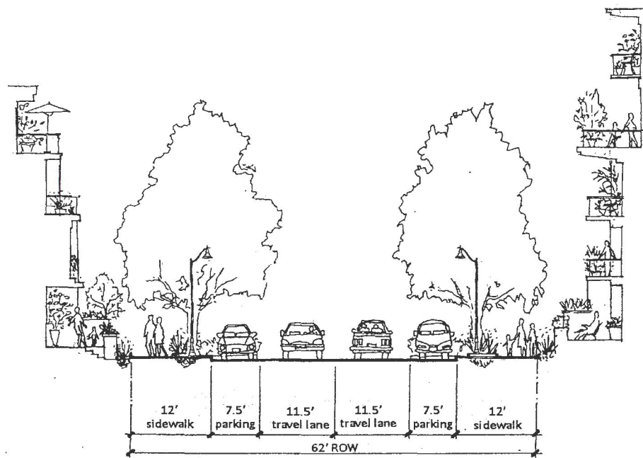
Figure 7—Typical Mixed Use Residential Street Cross-Section: Public Street
