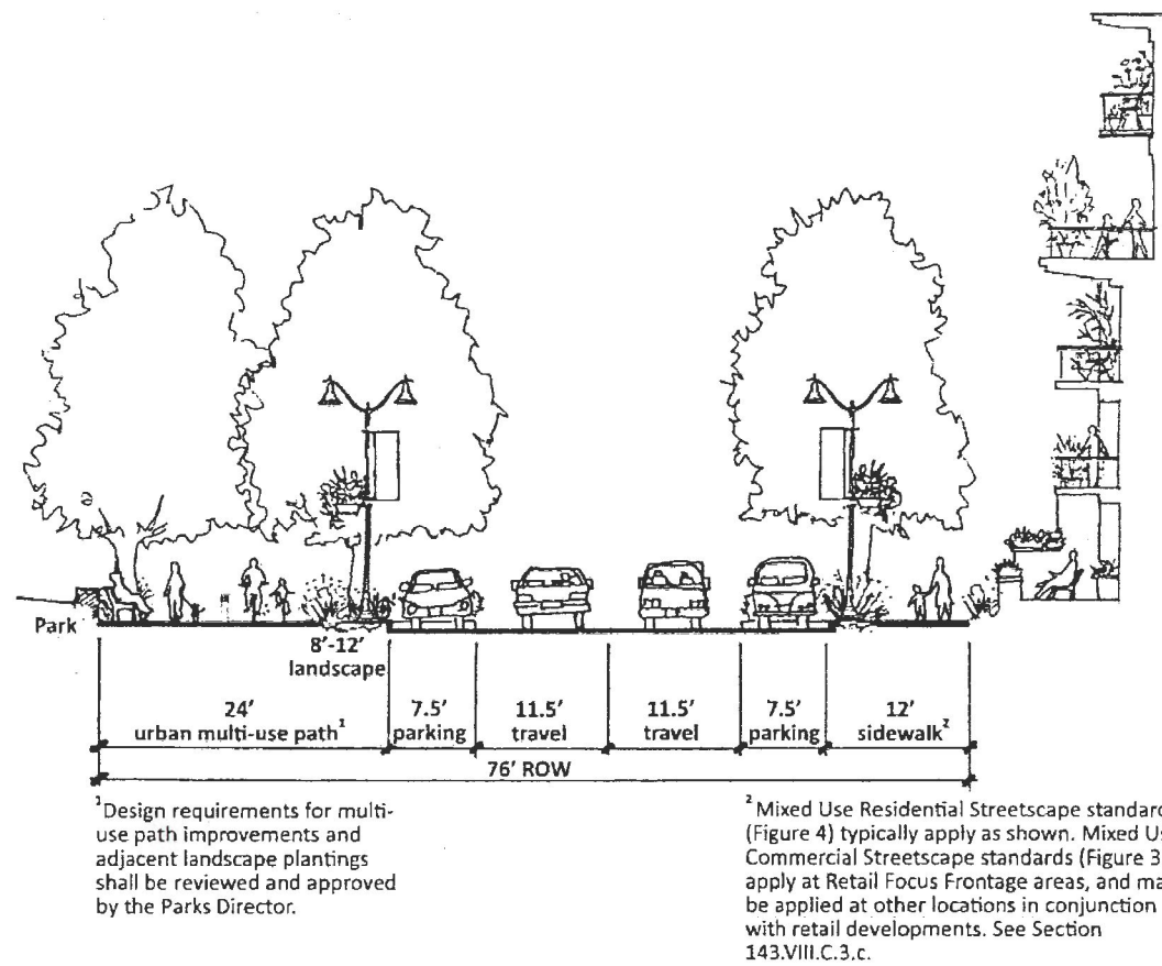
Figure 9—Typical Park Street Cross-Section: Public Street
