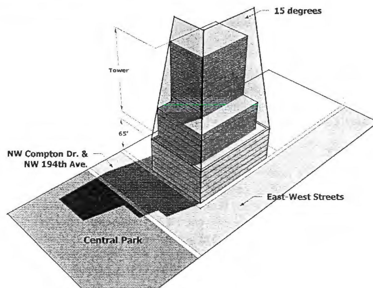
Figure 21—Example of bulk plane requirements.
