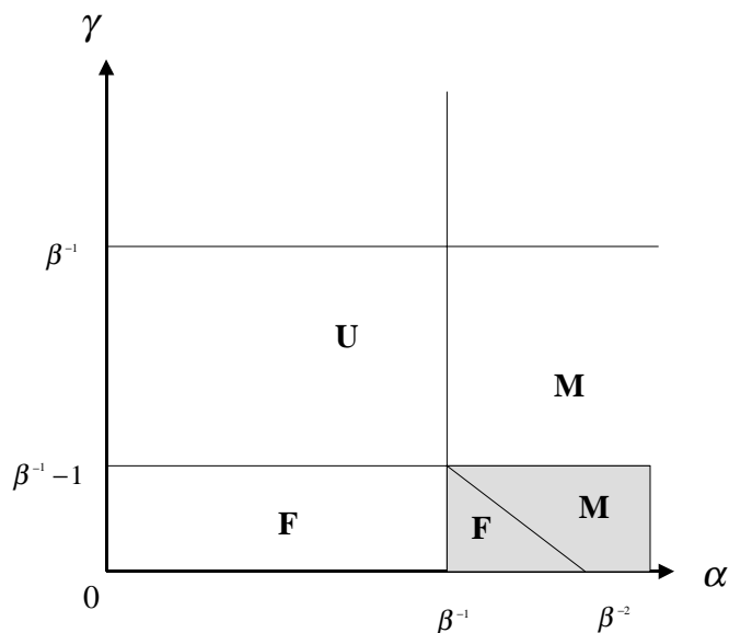
Figure 2: Regions of E-stable REE
