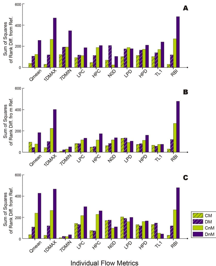
Figure 2.7. Individual flow metric impacts across scenarios as indicated by the sum of squares of rank differences (SSrd) from the reference. The SSrd of each future scenario for each flow metric indicates the relative difference of that scenario from the reference. Calculations of SSrd were based on the rank differences between each future scenario and the reference calculated for each of the 30 annual values of the flow metrics.
