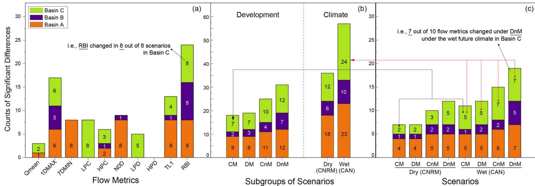
Figure 3.2. Counts of significant differences in flow metrics summarized by basin, flow metric, and scenario. This figure summarizes the results of the Combined Impacts test and reveals when and how much future climate x development combinations changed individual flow metrics. (a) shows which flow metrics were altered most often, and which basins experienced the most alterations. The maximum possible count of significant differences for each basin is 8. (b) shows which development and climate scenarios incurred the most instances of flow alterations. The maximum possible count of significant differences for each basin is 20 for the development scenarios (left) and 40 for the climate scenarios (right). (c) breaks down the results of (b) into individual climate x development combinations. The maximum possible count of significant differences for each basin is 10.
