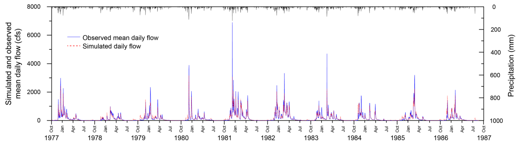
Figure 2.4. Mean daily flows from observed vs. simulated data for WY 1978-1987 (USGS 14167000 Coyote Creek near Crow, Oregon).
