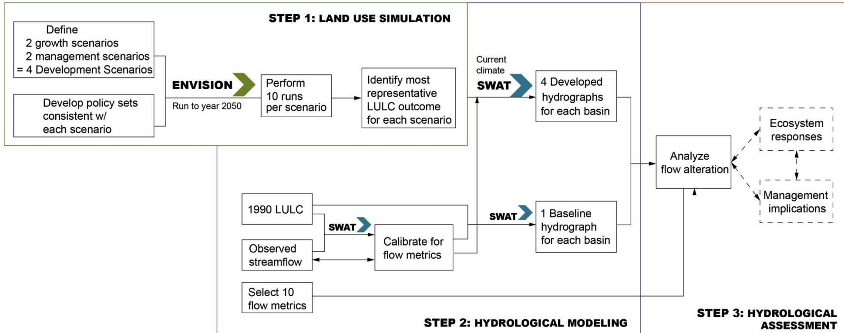
Figure 2.1. The overall modeling process under urbanization impacts alone.
