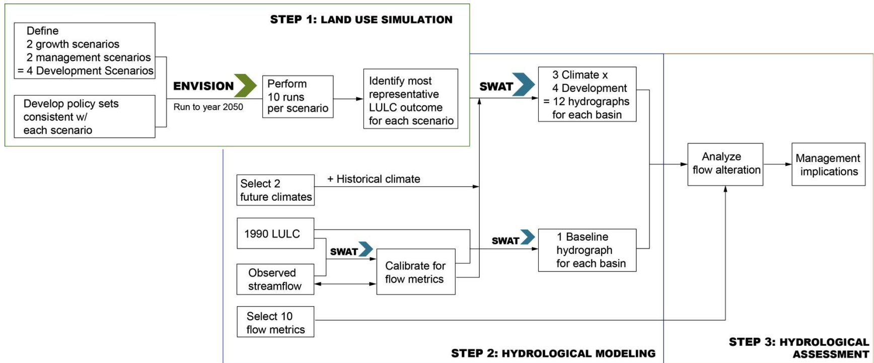
Figure 3.1. The modeling process under the combined impacts of urbanization and climate change.
