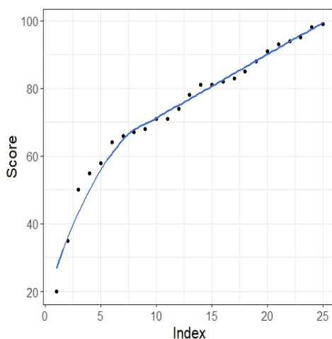
Figure 9: Locally-Weighted Regression Curve for Positively Correlated Data
