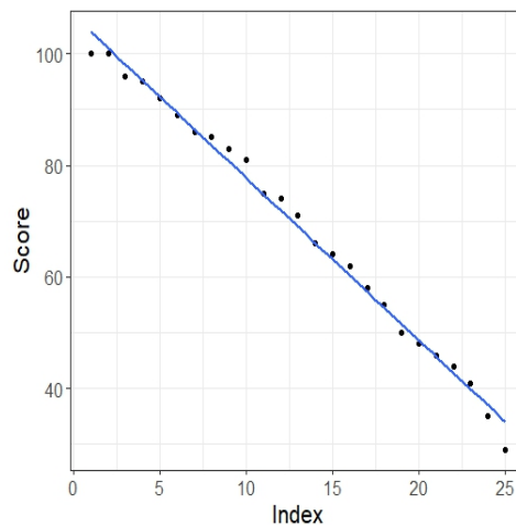
Figure 8: Best Fit Line for Negatively Correlated Data
