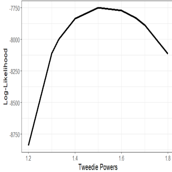
Figure 18: Profile Log-likelihood Plot for LM Home Fire LC Data
