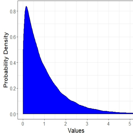
Figure 3: 100,000 Simulated Gamma( \alpha = 1, \beta = 1 ) Random Variables
