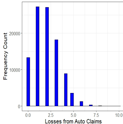
Figure 4: 100,000 Simulated Poisson( \lambda = 2 ) Random Variables
