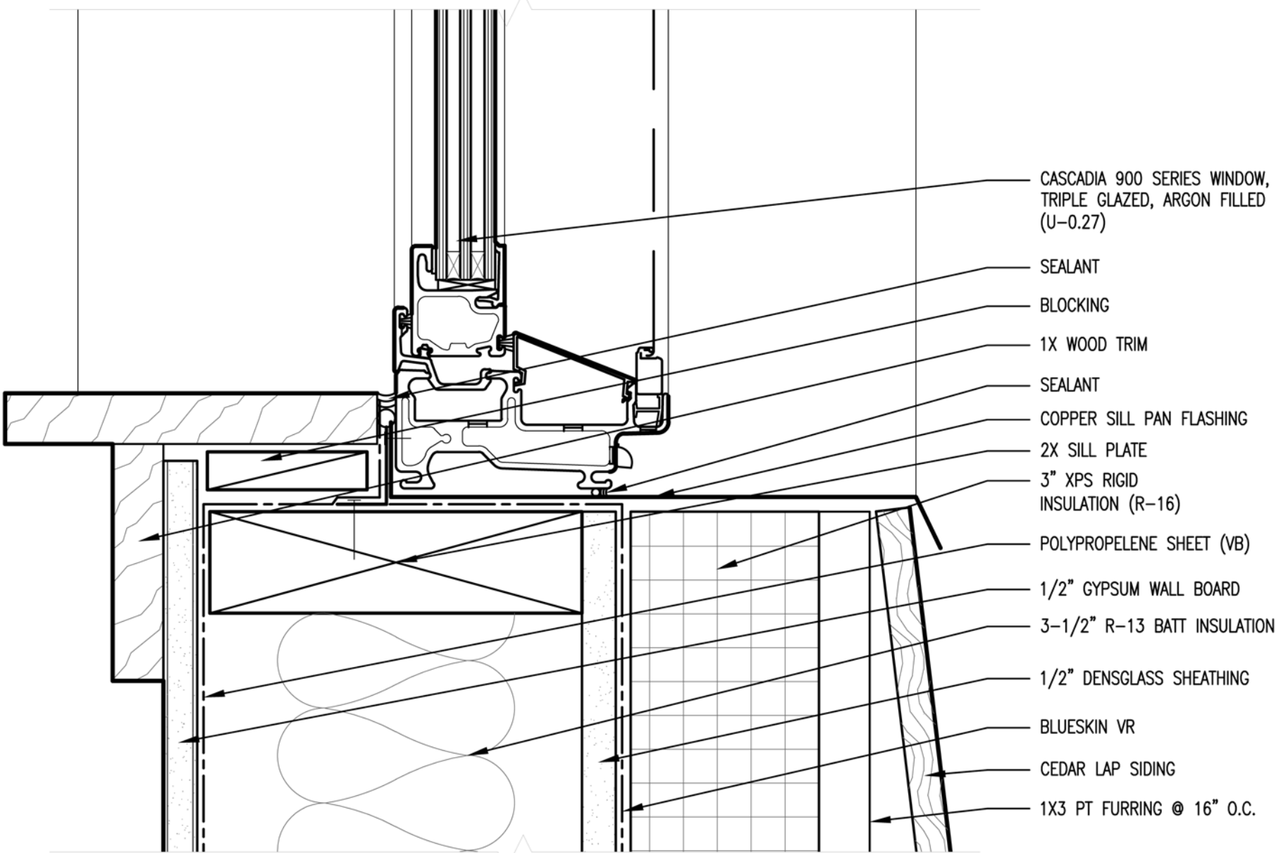
1 WINDOW SILL 6" = 1'-0"
