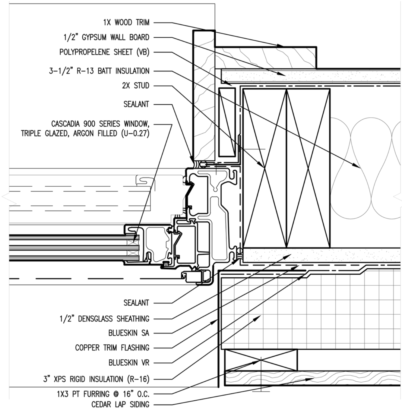
2 WINDOW JAMB 6" = 1'-0"
