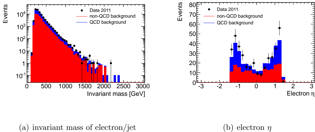
Figure 7.5. Signal region distributions without \Delta\eta selection. Distribution of electron \eta and invariant mass of electron and jet in the signal region without selection requirement for \Delta\eta are given. For the plot showing the invariant mass, no invariant mass selection has been made. The electron \eta distribution only shows events with invariant mass above 900 GeV. The background is estimated using the technique described in the following chapters.
