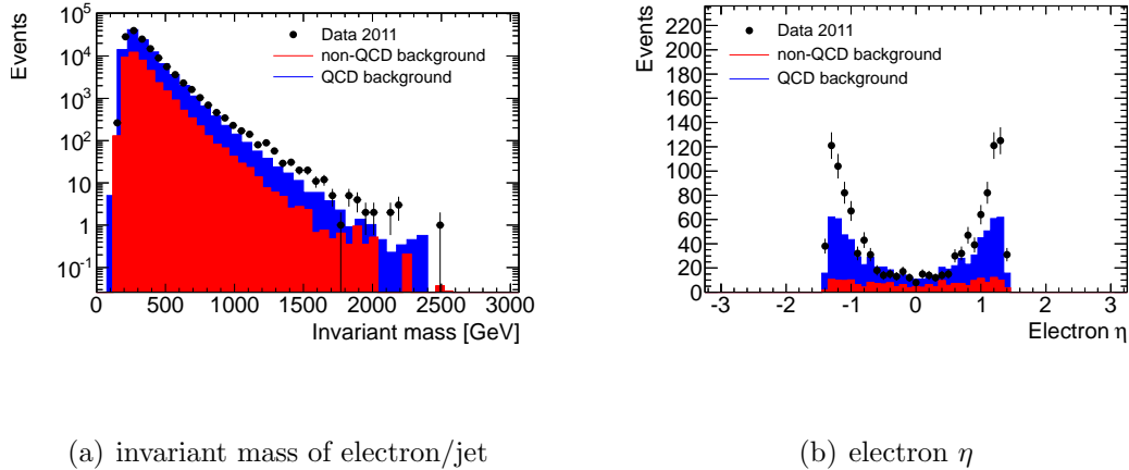
Figure 7.6. Signal region without \Delta\eta and isolation selection. Distribution of electron \eta and invariant mass of electron and jet in the signal region are given without any selection requirement for \Delta\eta and electron isolation. For the plot showing the invariant mass, no invariant mass selection has been made. The electron \eta distribution only shows events with invariant mass above 900 GeV. The background is estimated using the technique described in the following chapters.
