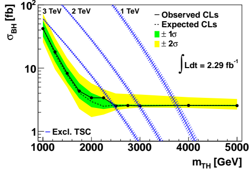
(a) 6 ADD-type extra dimensions
