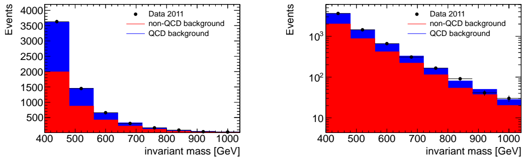
(a) invariant mass of electron/jet
