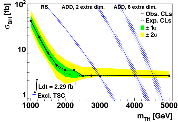
Figure 12.2. Upper limits on cross section (2). Expected and observed upper limit of the cross section of lepton plus jet events are displayed without consideration of signal PDF uncertainty. As comparison, different predicted cross sections are shown for models with a Planck mass of 2 TeV. The cross sections are given as a function of the minimum BH mass M_{TH} for different type and number of extra dimensions. The hatched area shows the theoretical cross section uncertainty due to the PDF uncertainties. CTEQ6.6 is used as PDF and the uncertainties are derived by considering its 44 PDF eigenvectors. All cross sections are shown for models without considering trapped surface calculations. For the calculation of the theoretical signal cross section, only BHs of charge 1/3 and 4/3 produced in interactions between two quarks (q-q) have been included. Some of the points may be unphysical, since M_{TH} is smaller than x_{min} \times M_{Pl} with x_{min} \geq 1 .
