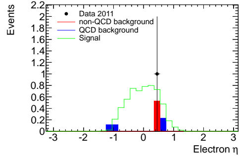
(b) Leading electron \eta
