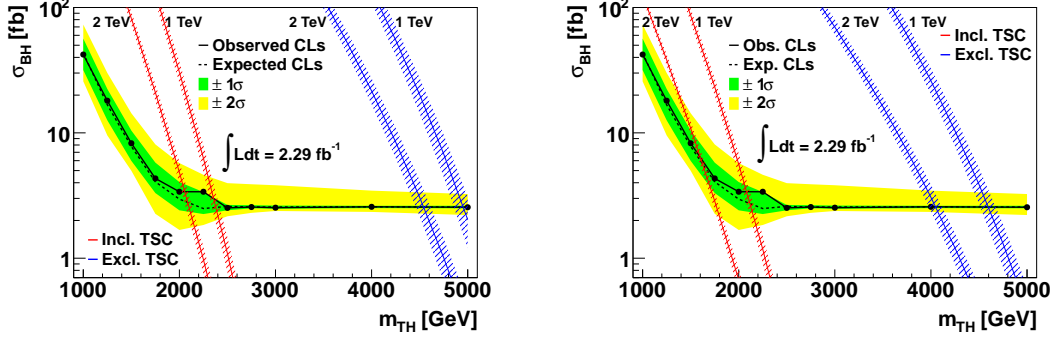
(a) 6 ADD-type extra dimensions
