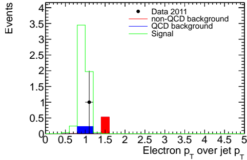
(c) Ratio of electron p_T and jet p_T
