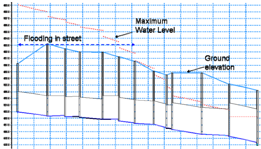
Figure 3-4 Hydraulic Profile for Piped System during Flooding Conditions
