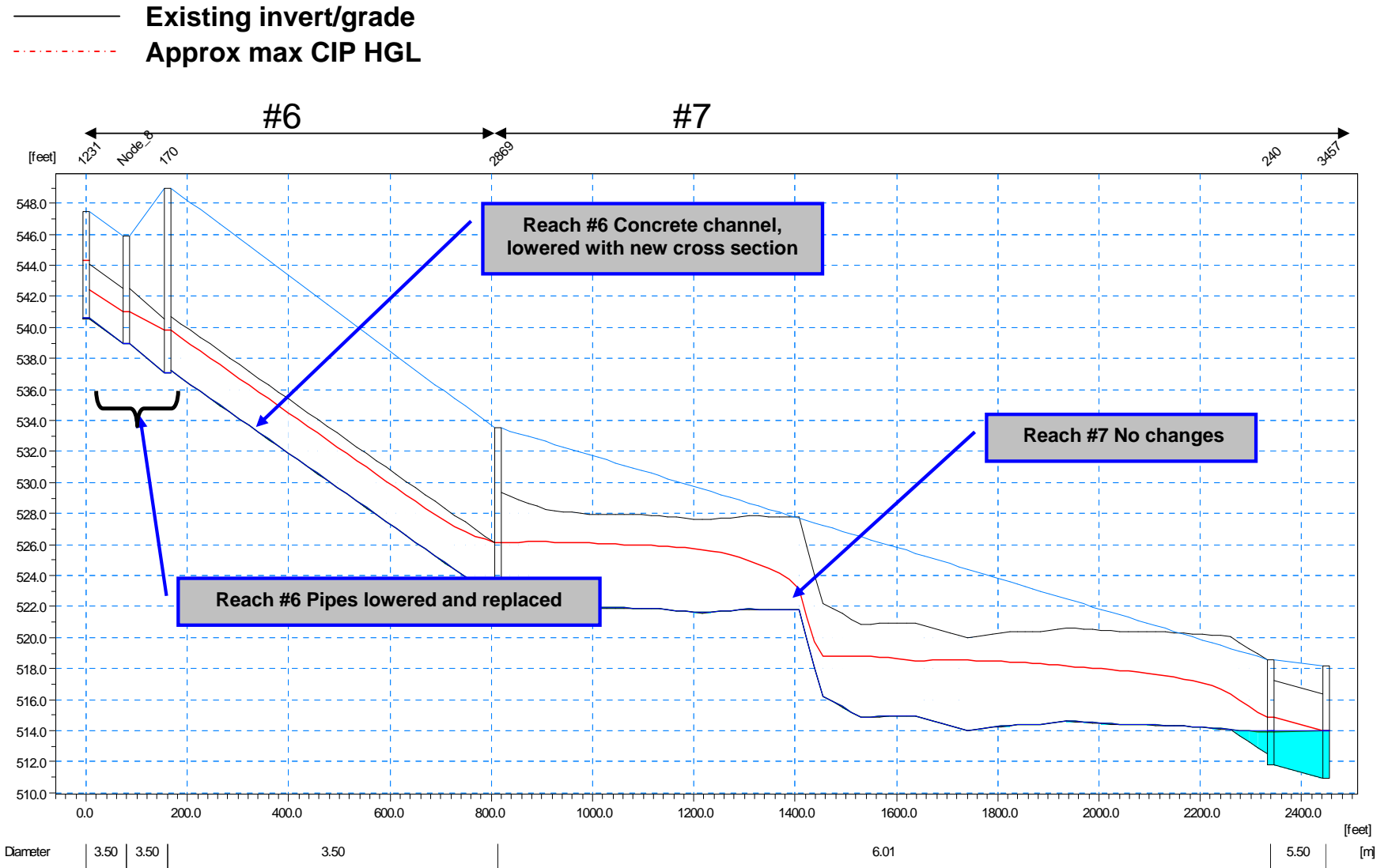
Figure E-12 Springfield2 – Reaches #6 and #7 – Future Condition
