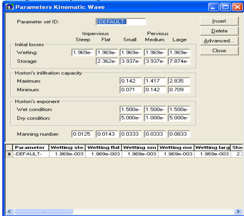
Figure 3-3 Hydrological Parameters used in Mike Urban
