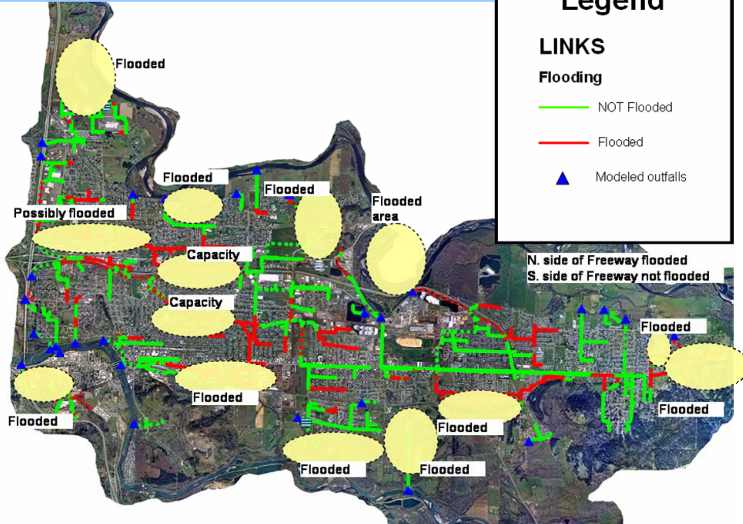
Figure 13 Flood Map Springfield - 1996 Storm Event; observed flooding circled and mapped in the picture along with model estimated results.
