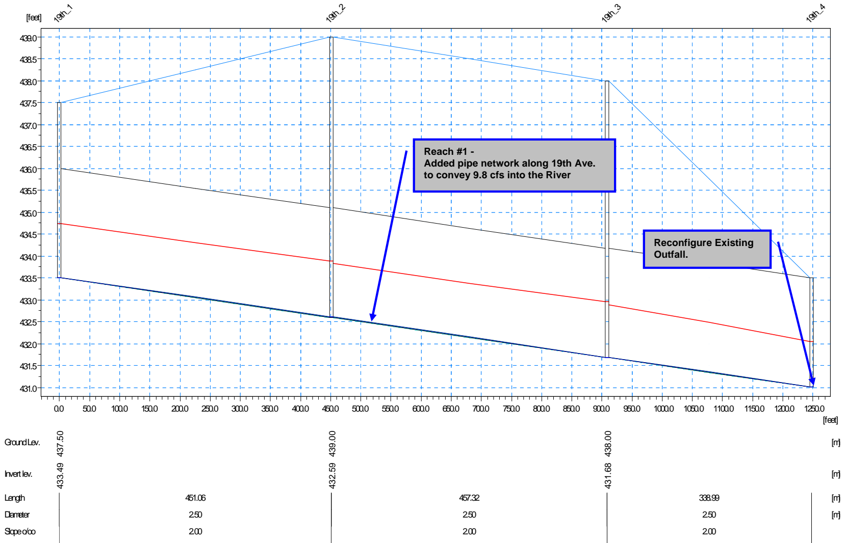
Figure E-2 Springfield1 – Reach #1 – New Reach (Future Condition)
