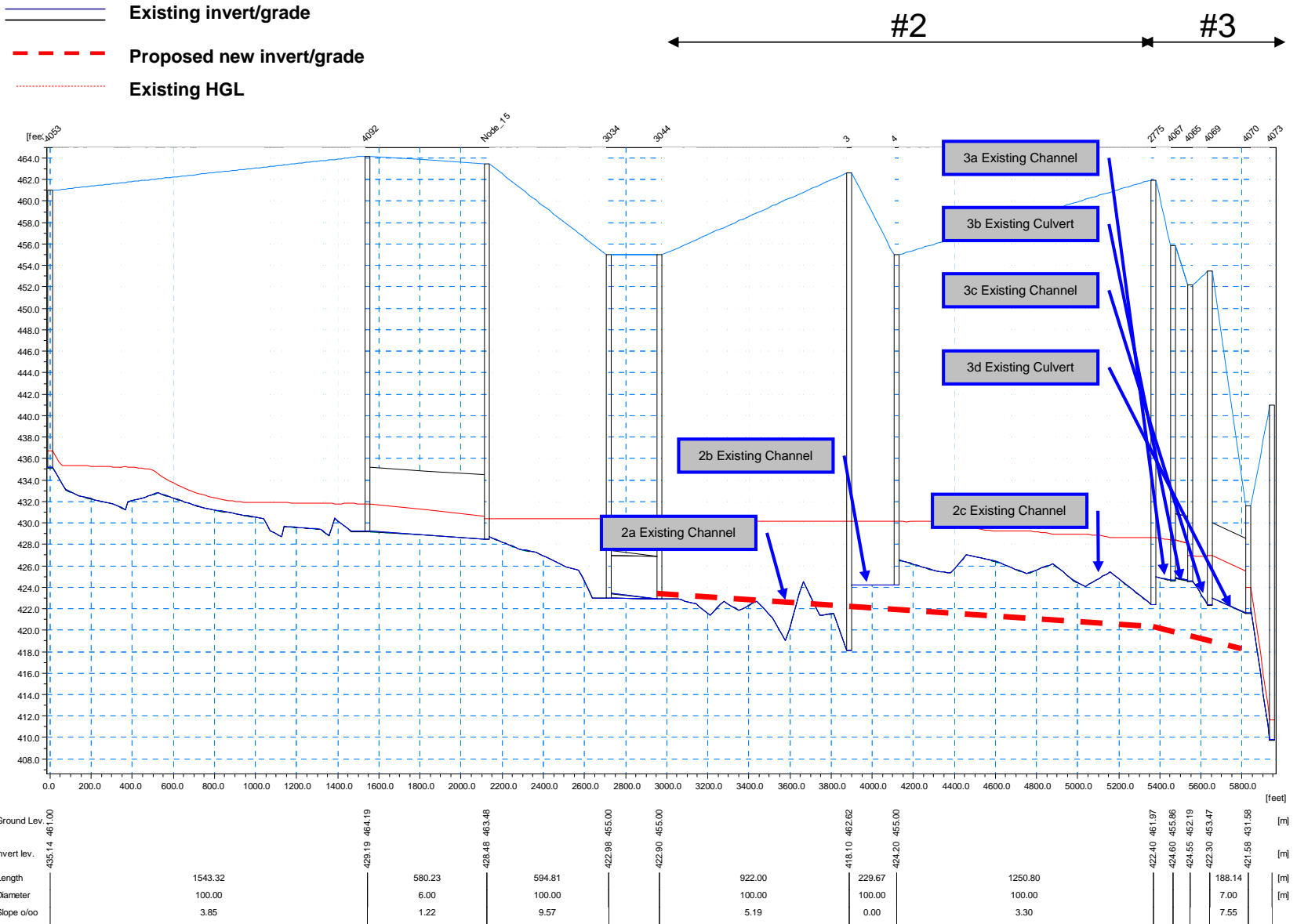
Figure E-3 Springfield1 – Reaches #2 and #3 – Existing Conditions
