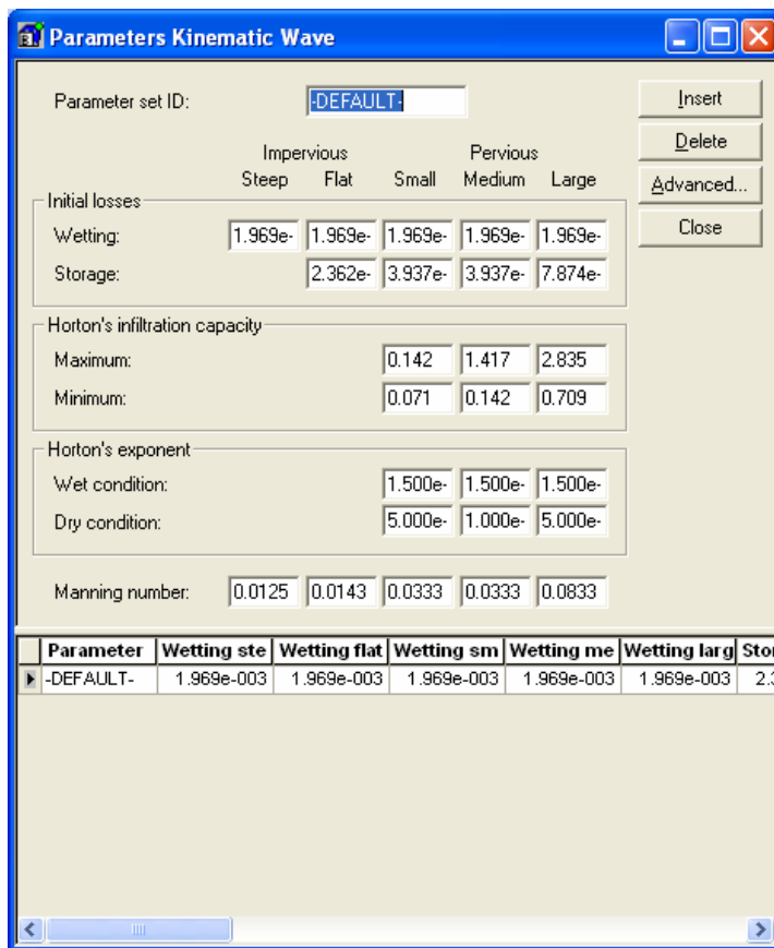
Figure 5: Hydrological Parameters used in Mike Urban
