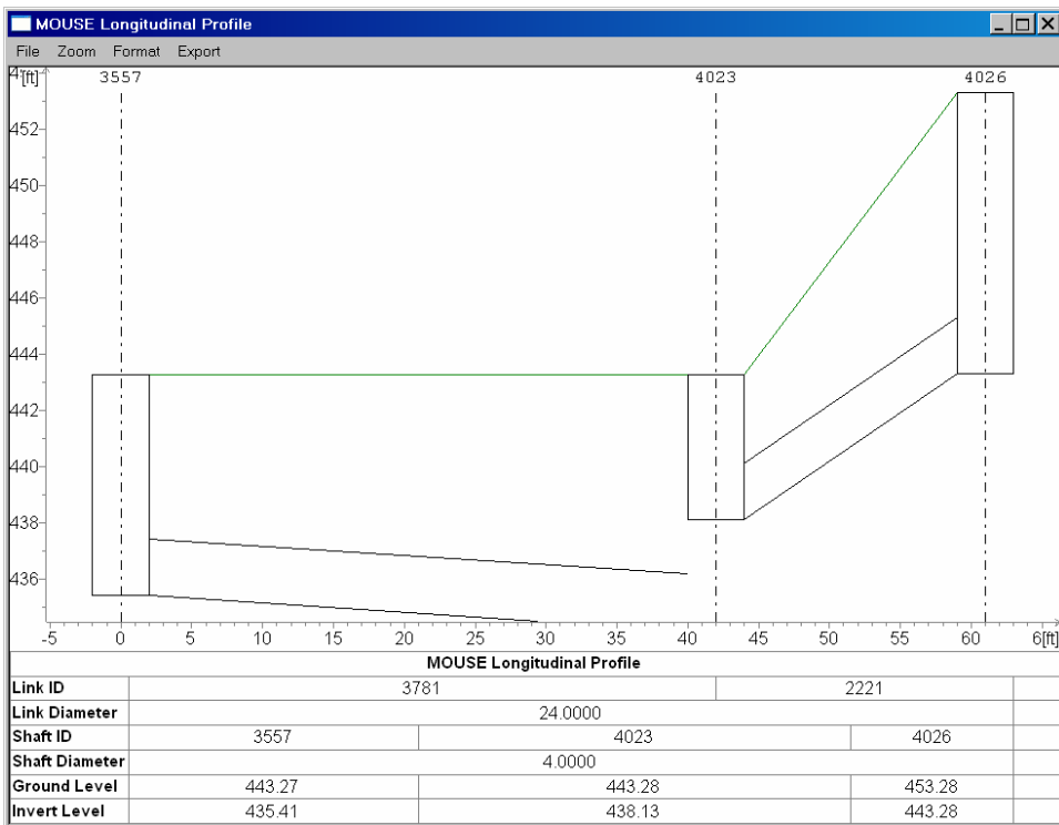
Figure 3: Longitudinal Profile of Network – Example of missing invert.
