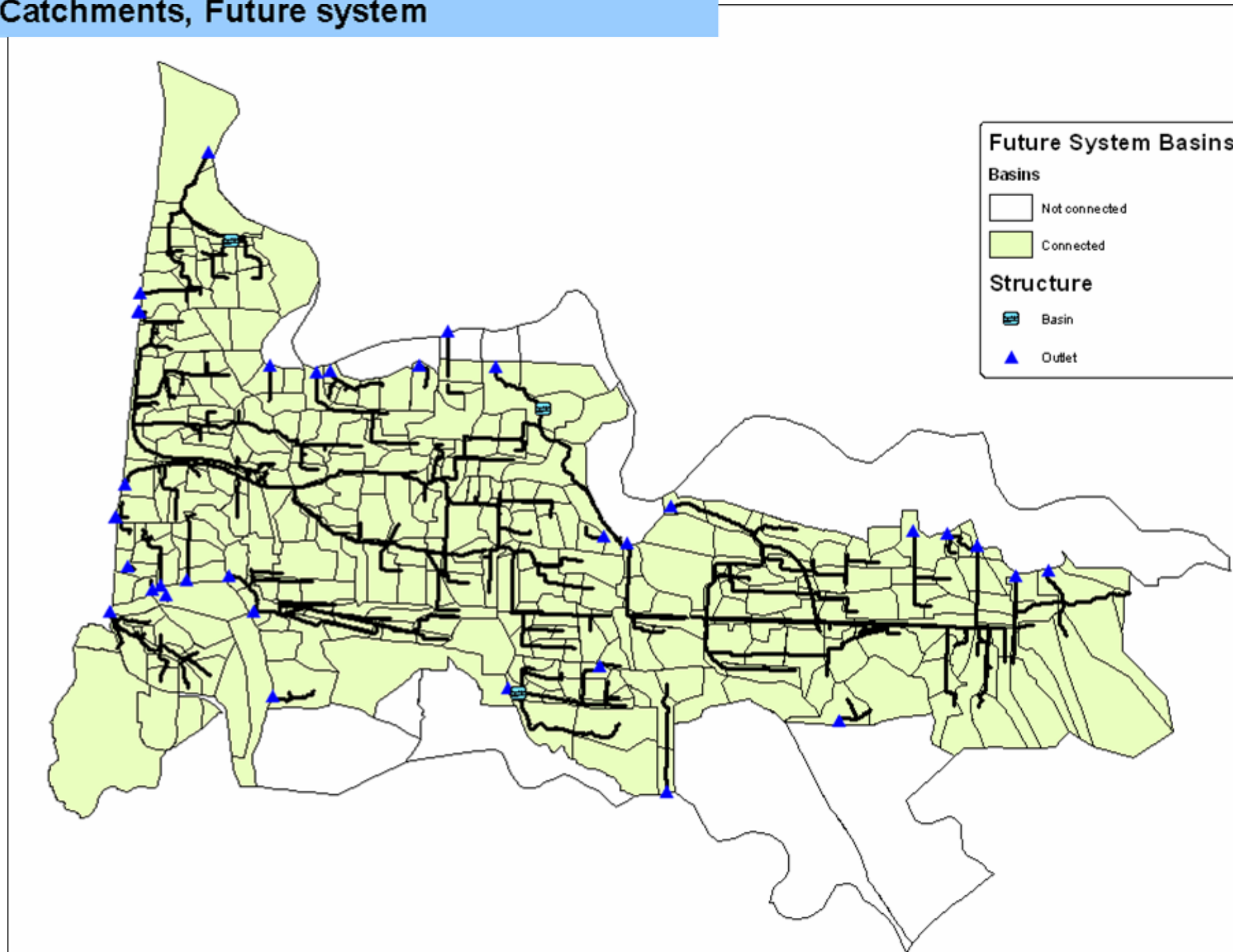
Figure 15 Catchments connected (in green) to the modeled future system file as a result of the calibration steps performed to the model
