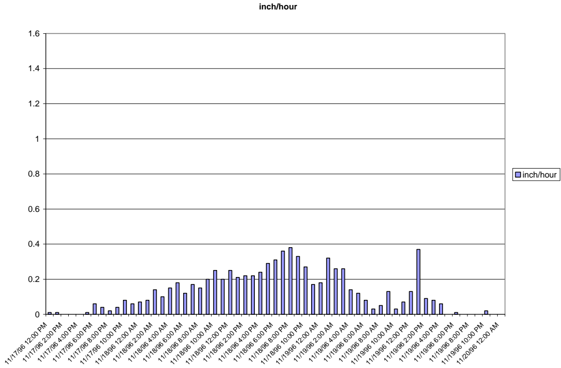
Figure 3-1 November 1996 Storm Event, Rain Intensity (inch/hour)
