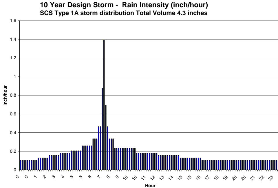
Figure 3-2 10 year Design Storm Event, Rain Intensity (inch/ hour)
