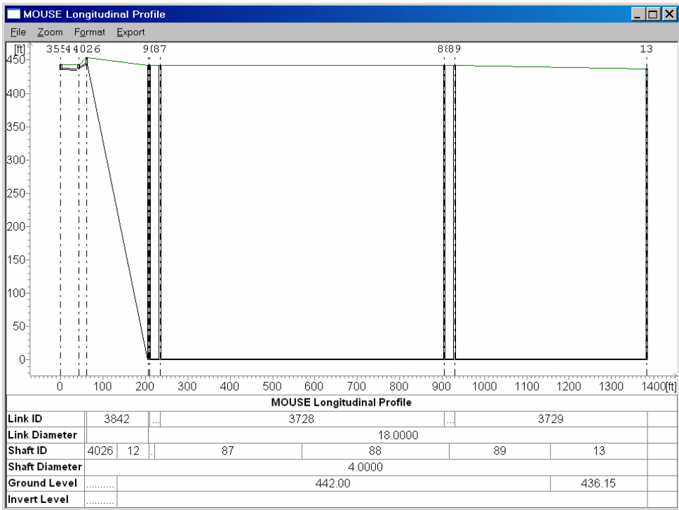
Figure 2: Longitudinal Profile of Network – Example of missing invert.
