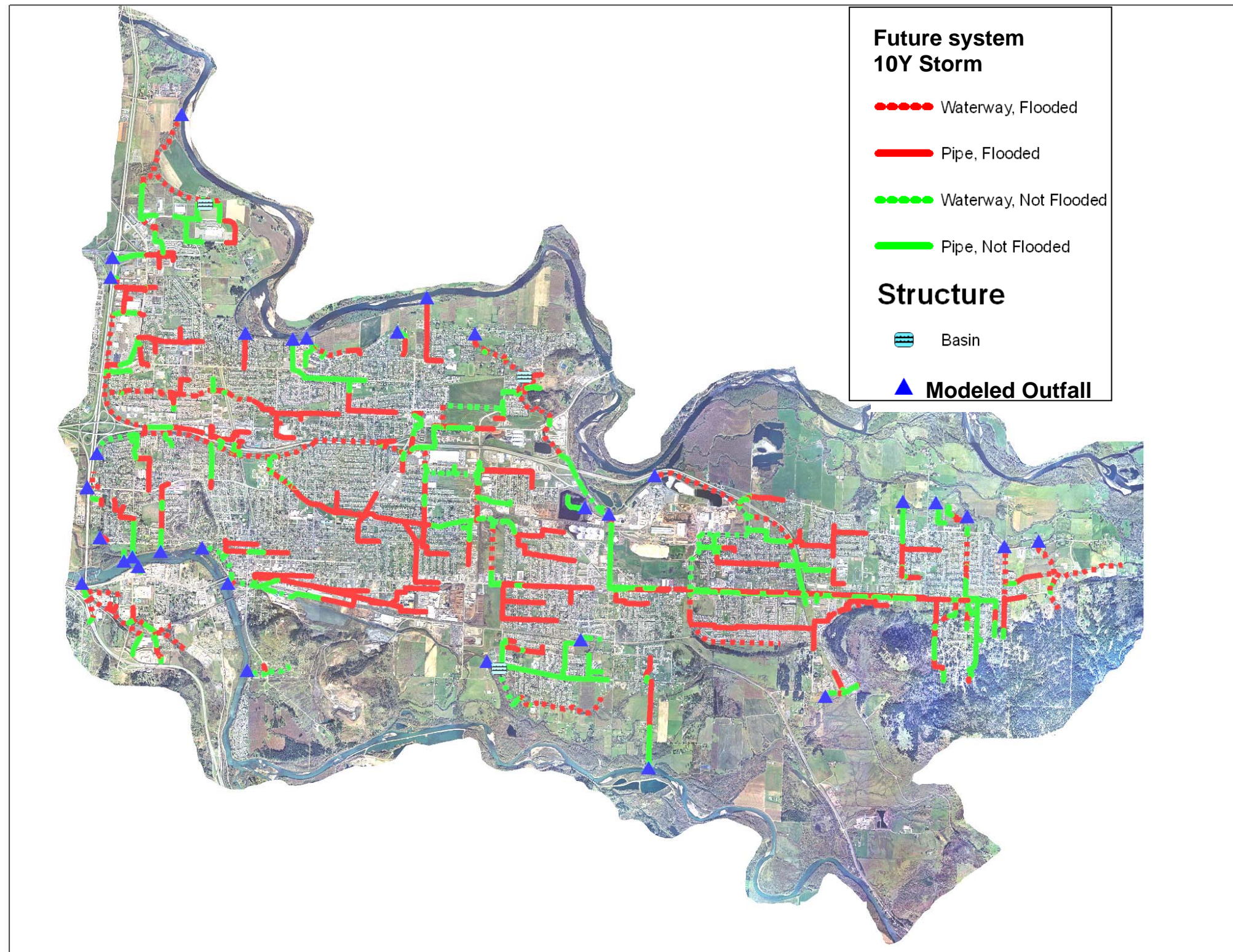
Figure 16 Future System Flood Map 10y Design Storm
