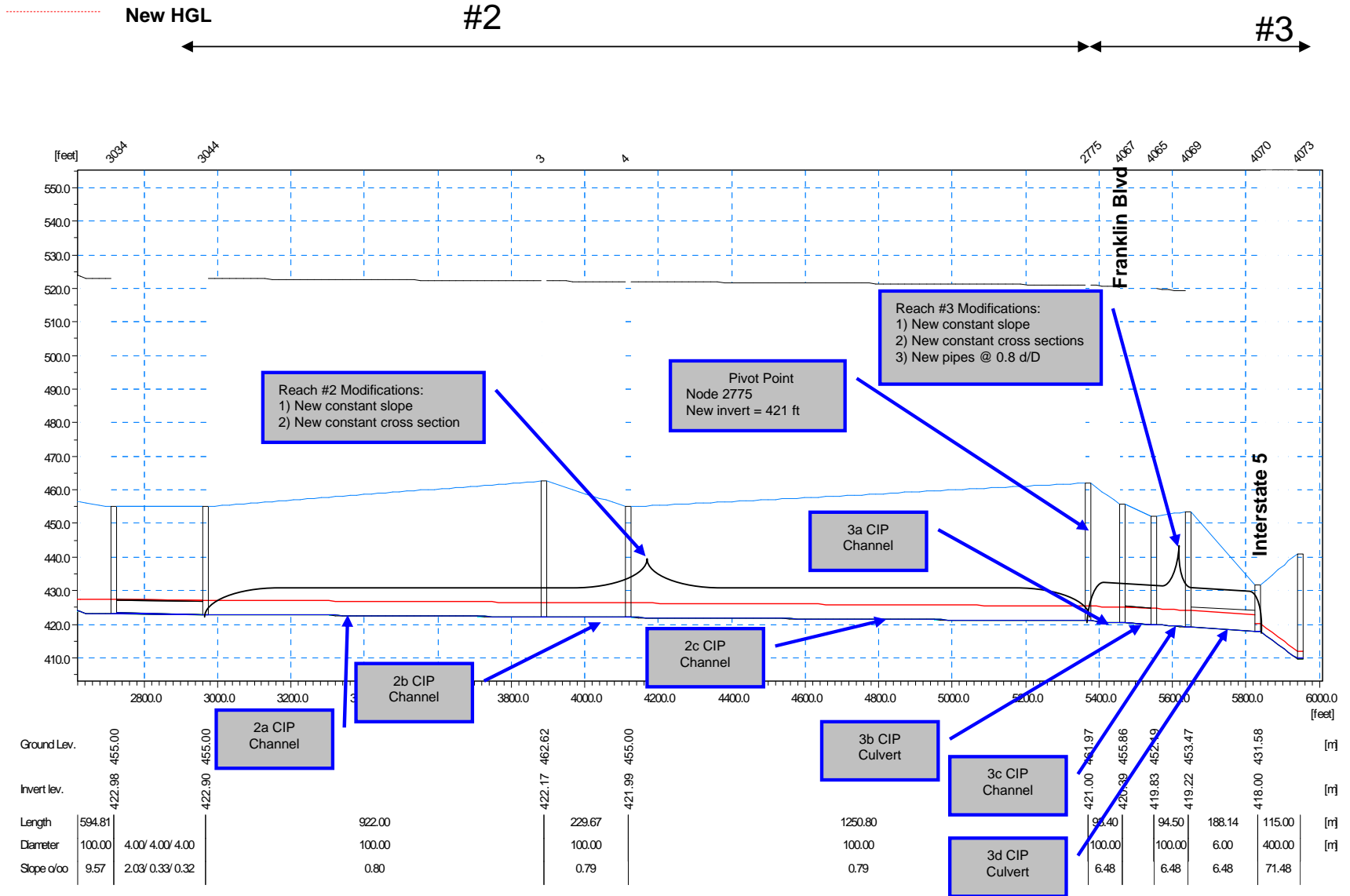
Figure E-4 Springfield1 – Reaches #2 and #3 – Future Conditions
