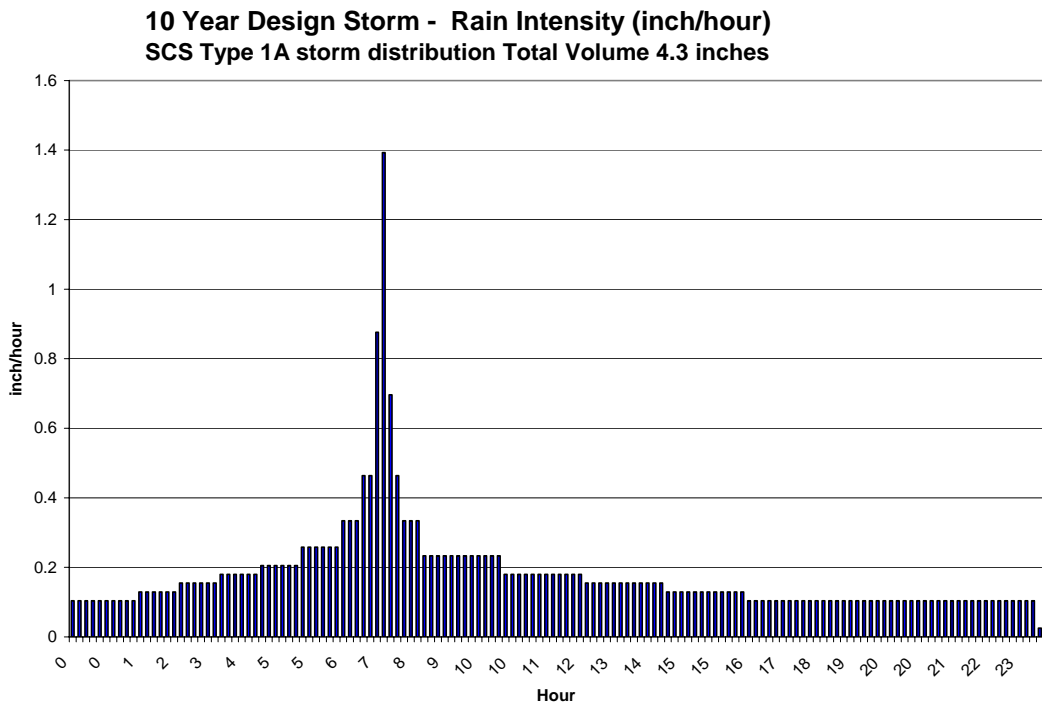
Figure 7 10y Design Storm Event; rain intensity (inch/hour)
