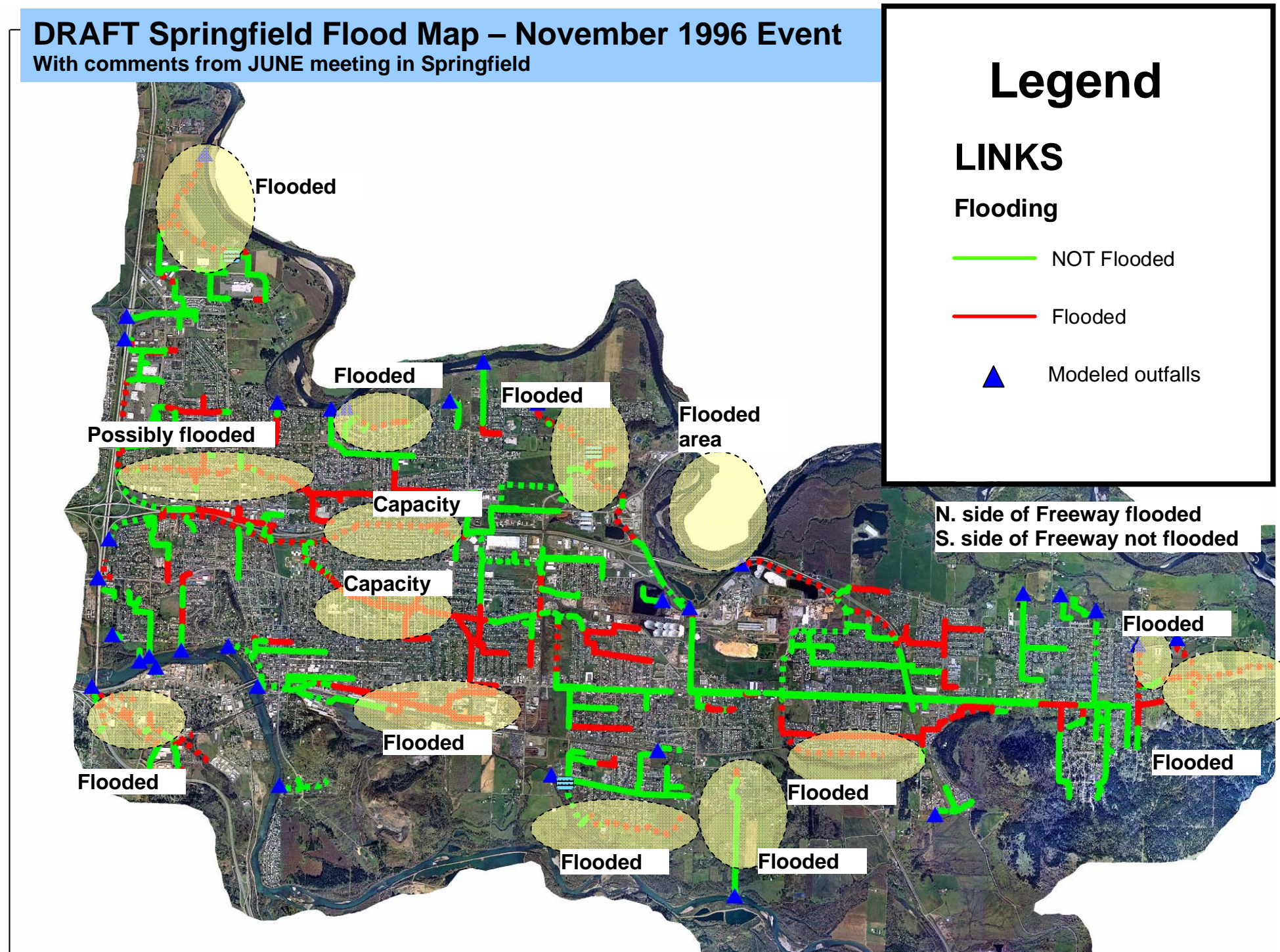
Figure 3-8 Flood Map – November 1996 Storm Event, Observed Flooding Circled and Mapped with Model Estimated Flooding Results
