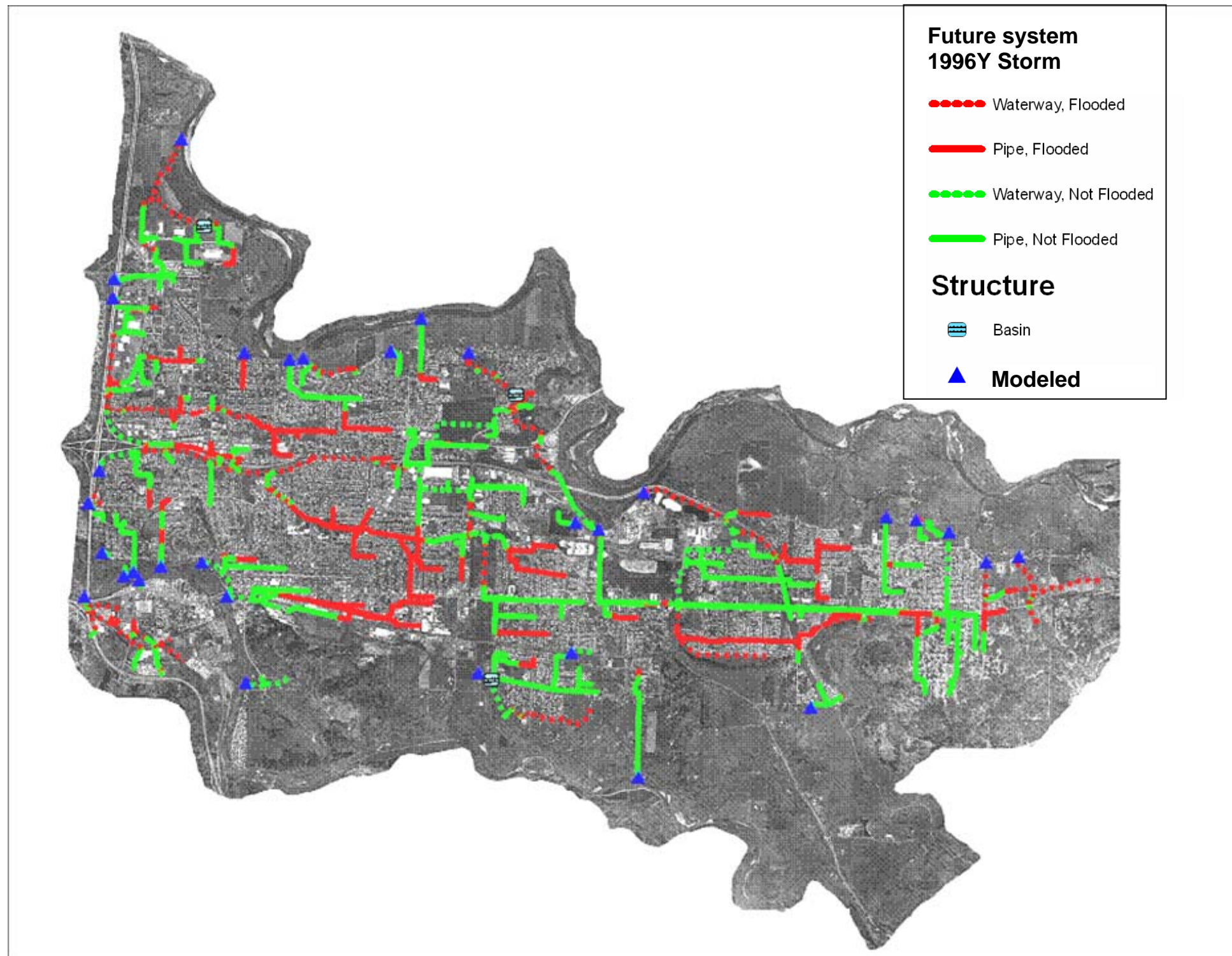
Figure 3-11 Future Condition System Flood Map 1996 Storm Event
