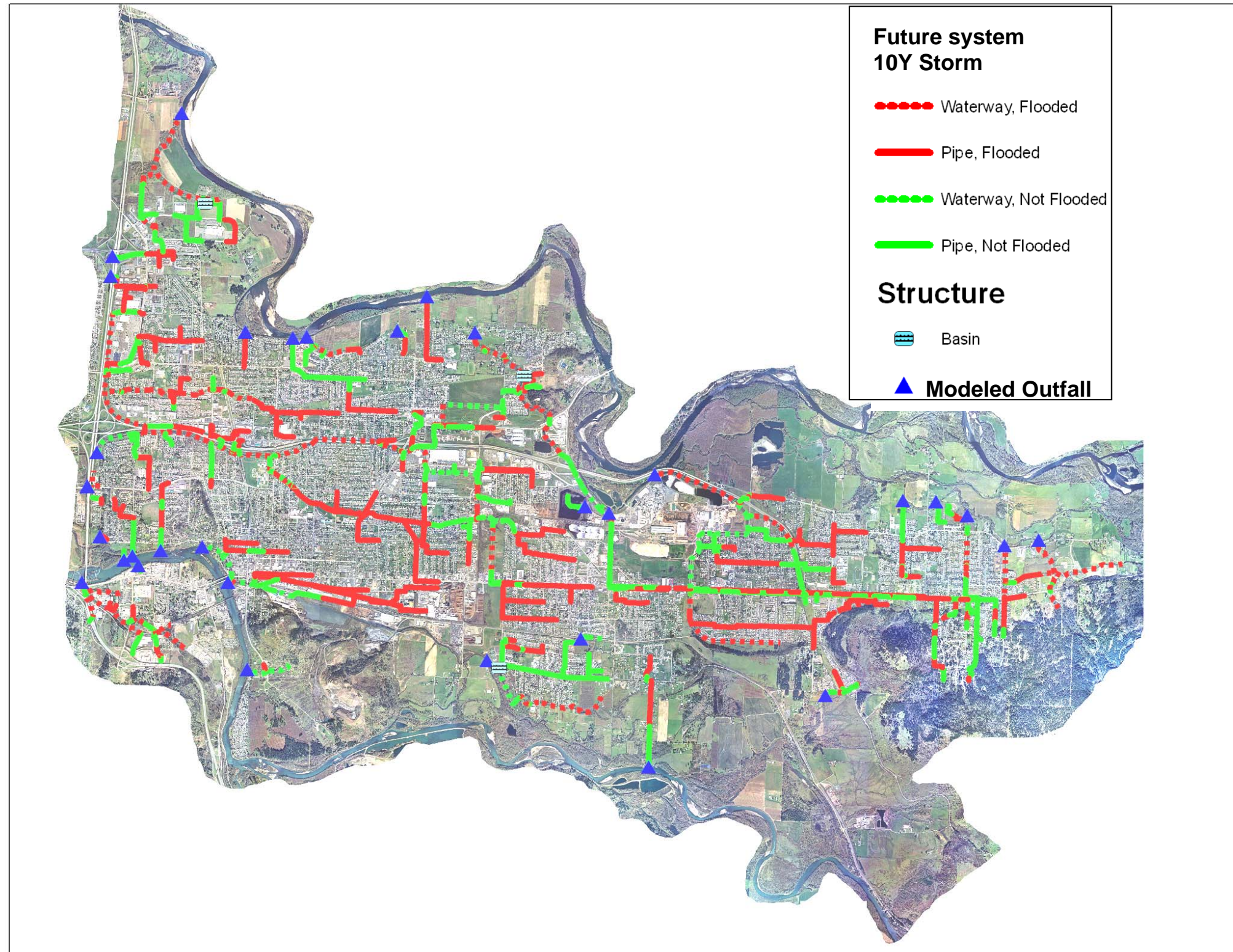
Figure 3-10 Future Condition System Flood Map 10y Design Storm
