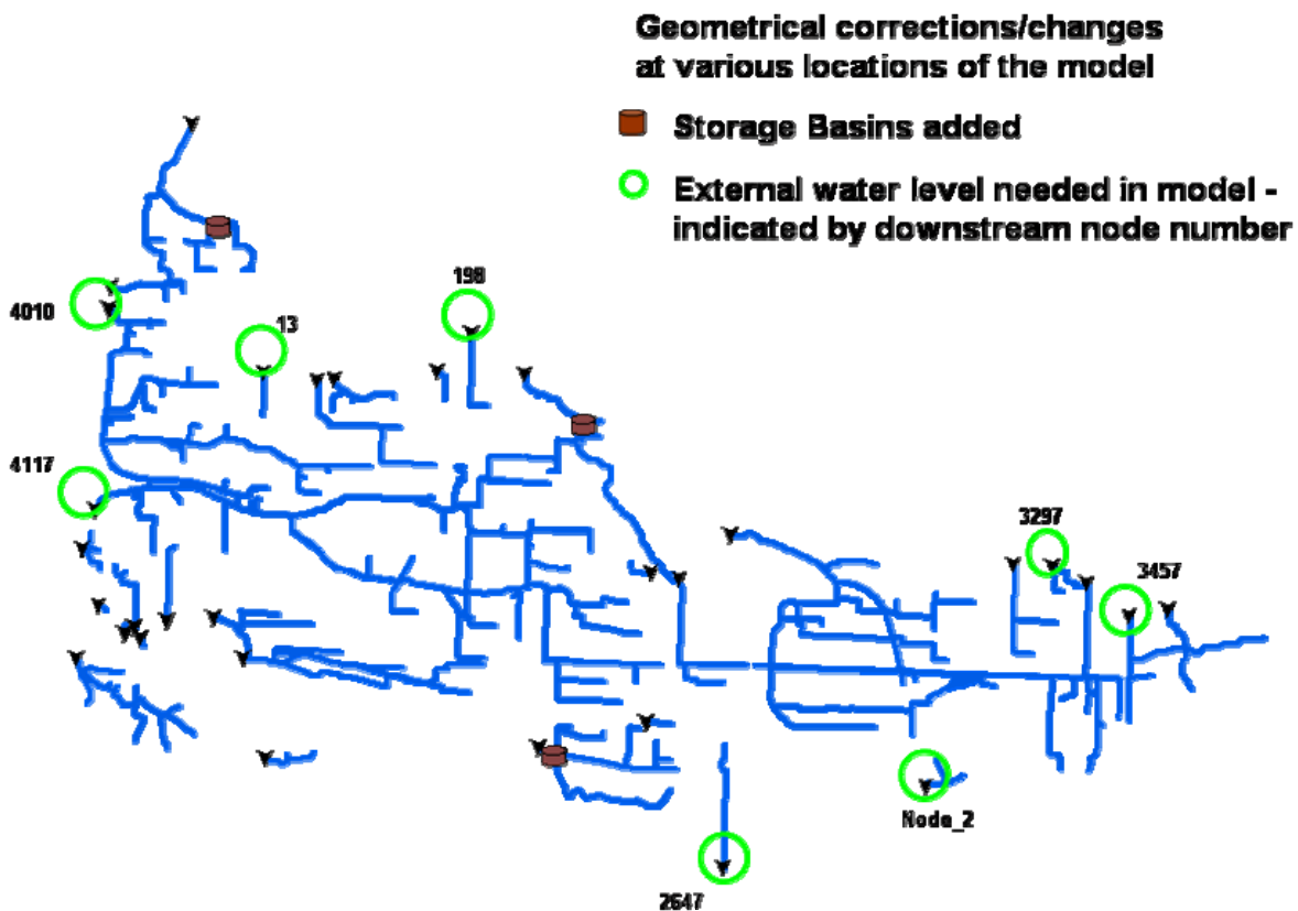
Figure 9 Model adjustments conducted as part of the calibration process
