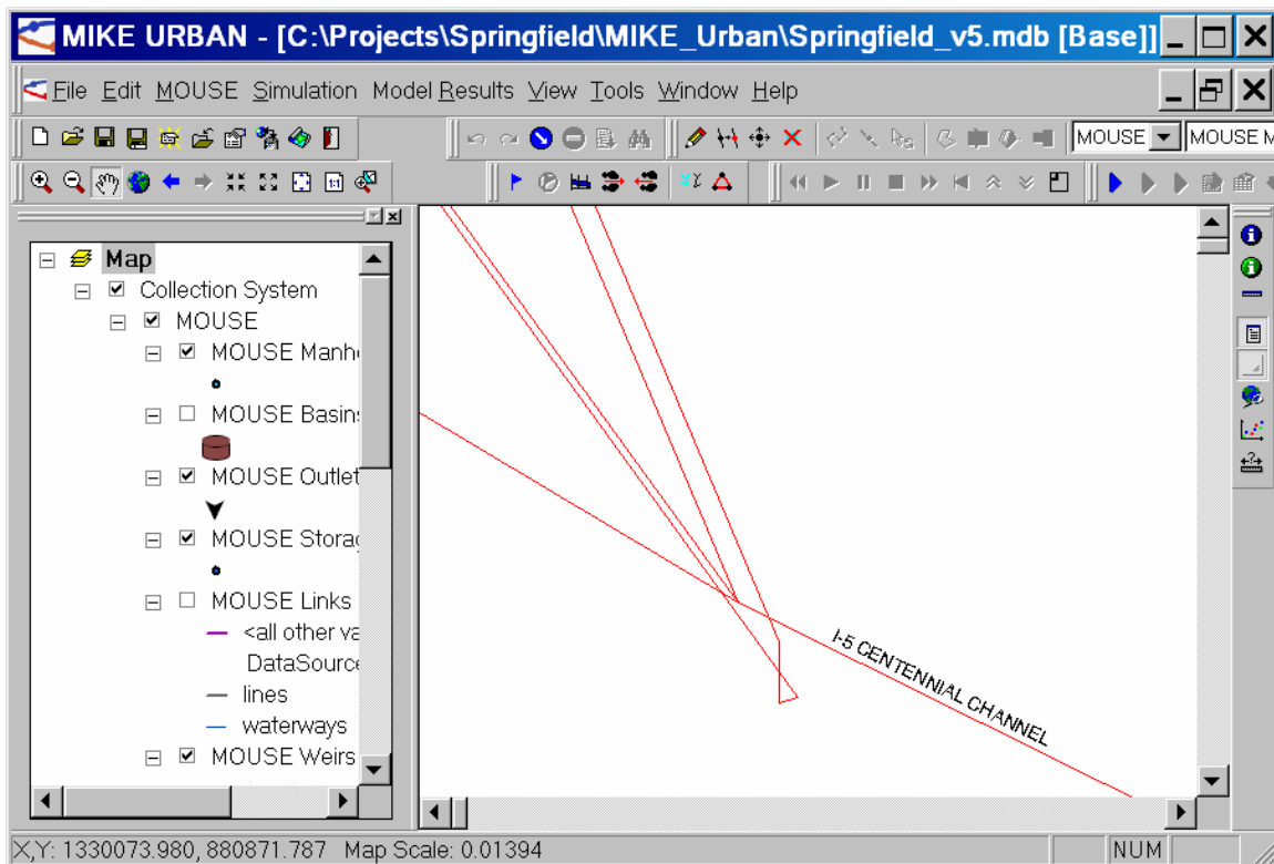
Figure 1: Example of Improper Network Geometry at Flow Bifurcation.
