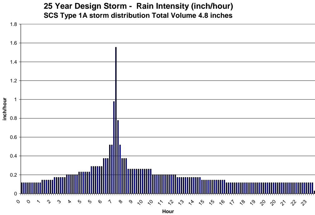
Figure 8 25y Design Storm Event; rain intensity (inch/ hour)
