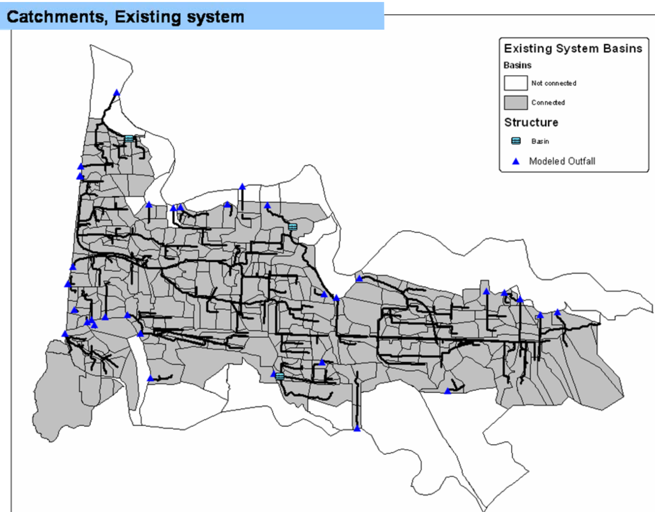
Figure 3-7 Catchments (in gray) Reflecting Model Adjustments Made as a Result of the Model Validation Process
