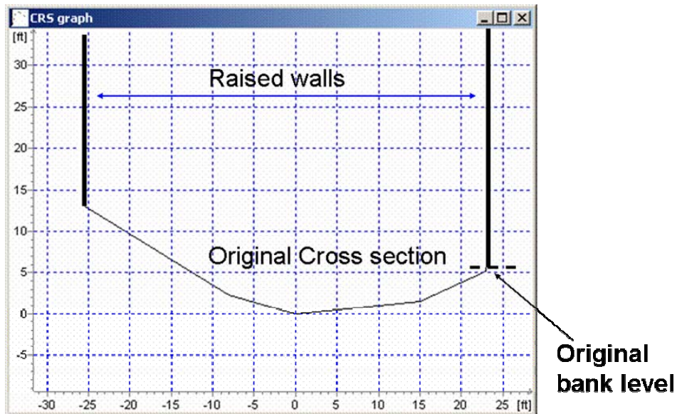
Figure 12 Typical cross section along a waterway used in the model
