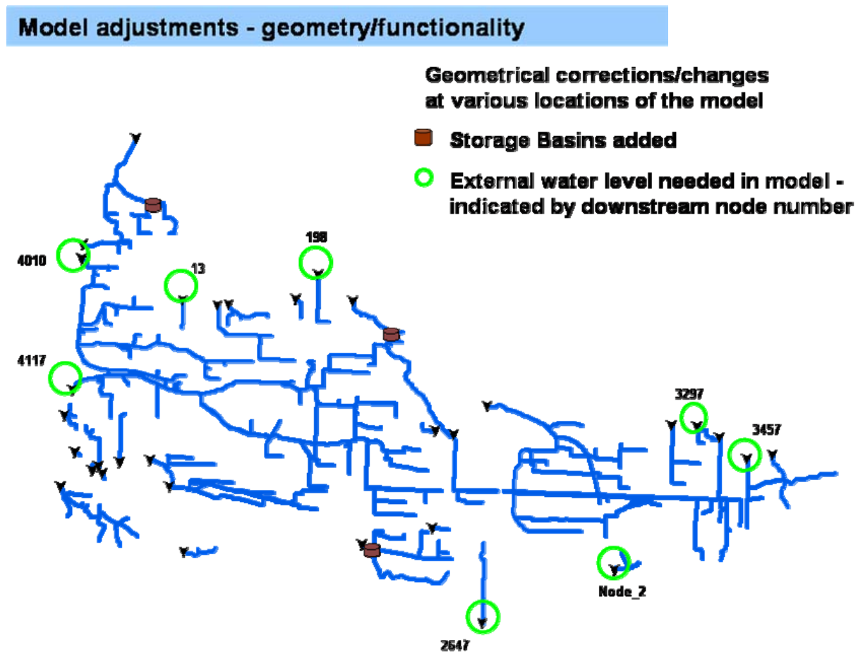
Figure 3-6 Model Adjustments Conducted as a Result of the Model Validation Process
