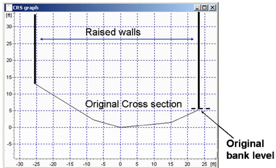
Figure 3-5 Typical Cross Section Along a Waterway Used in the Model
