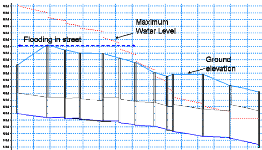
Figure 11 Hydraulic profile showing the inverts of several pipe sections along with the calculated HGL (in red)
