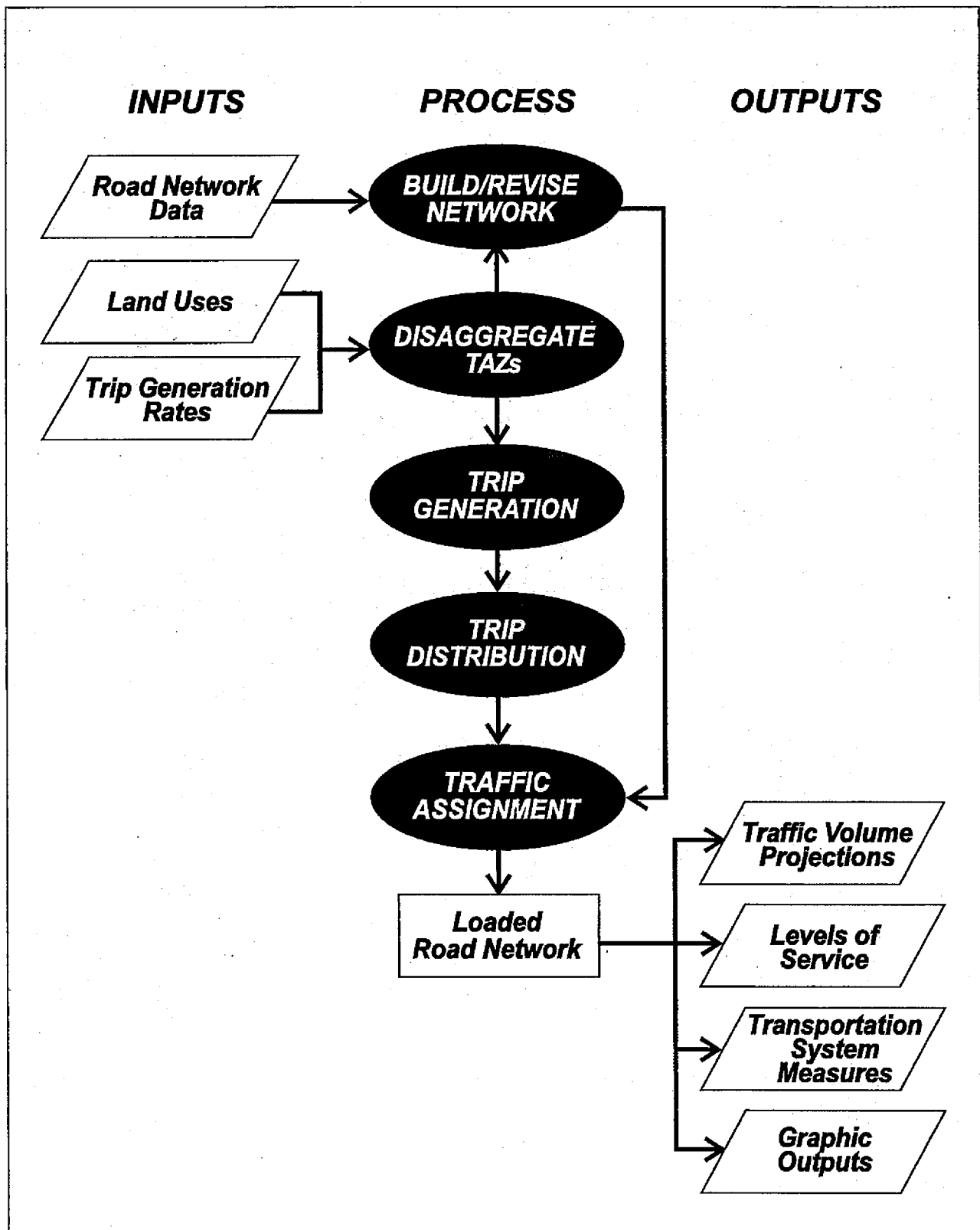
Figure 4-2 MODEL PROCESS
