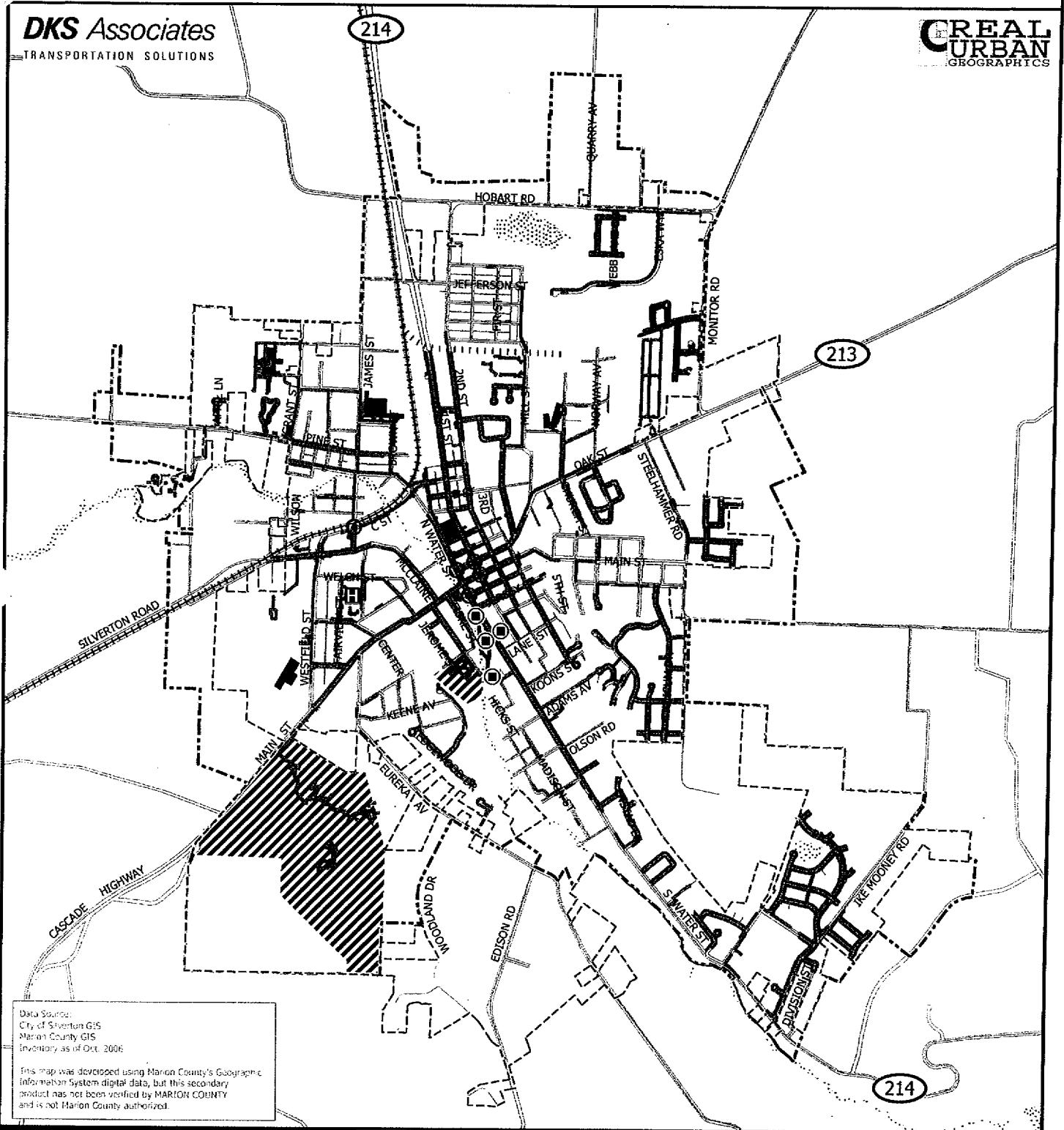
FIGURE 3-2 Existing Pedestrian Facilities
