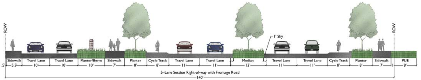
5-Lane Section with Median and Frontage Road
