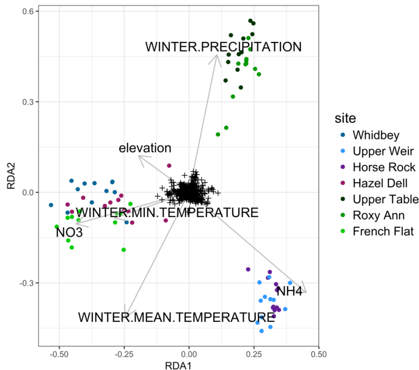
Figure 19: Tri-plot showing the effect of environmental variables on community composition of F. roemerii fungal endophytes.
