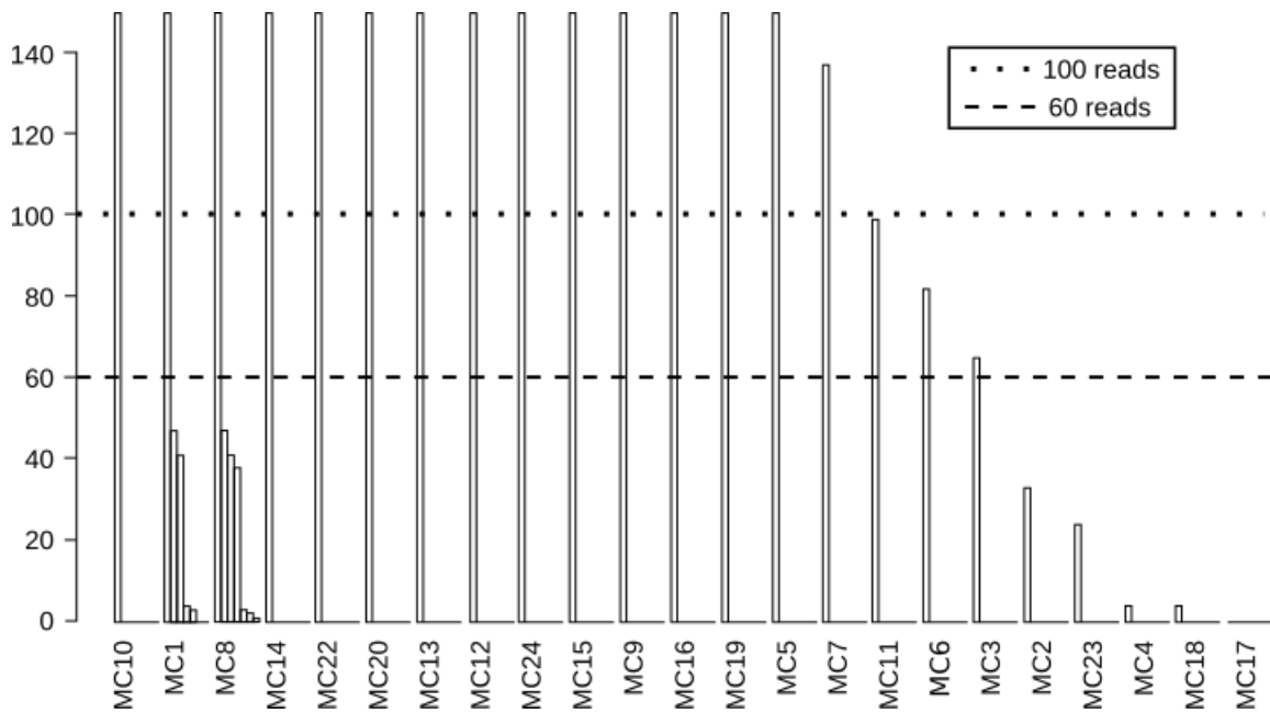
Figure 5.3. Truncated ranked read distribution of abundances of genomic positive control, including OTU splitting of mock-community members. The 100-read line represents the level around which tag-switching errors were observed to occur in the study (see Fig. 5.7 ), the 60-read line represents the abundance which authors of the subsequent ecological study chose as a minimum abundance cut-off for observations. Click here for a higher resolution image.
