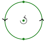
FIGURE 6.1 \mathbb{R}P_{tw}^2
