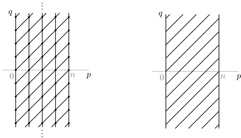
FIGURE 2.3 \mathbb{A}_n = H^{*,*}(S_a^n)
