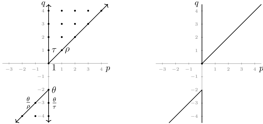
FIGURE 2.2 \mathbb{M}_2 = H^{*,*}(pt)
