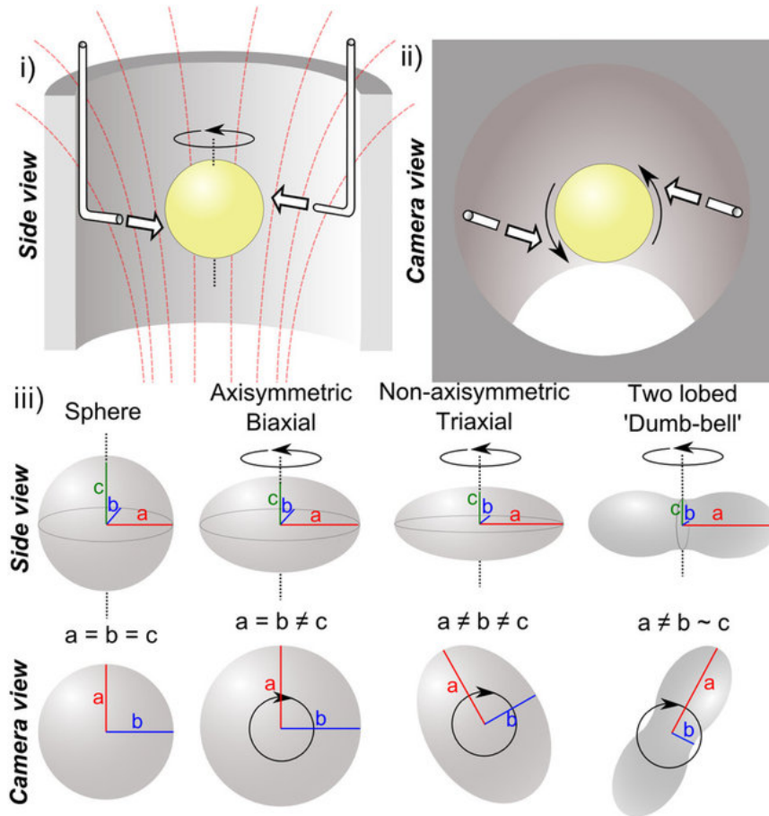
Figure 2: Simple Bifurcation of a Rotating Sphere
