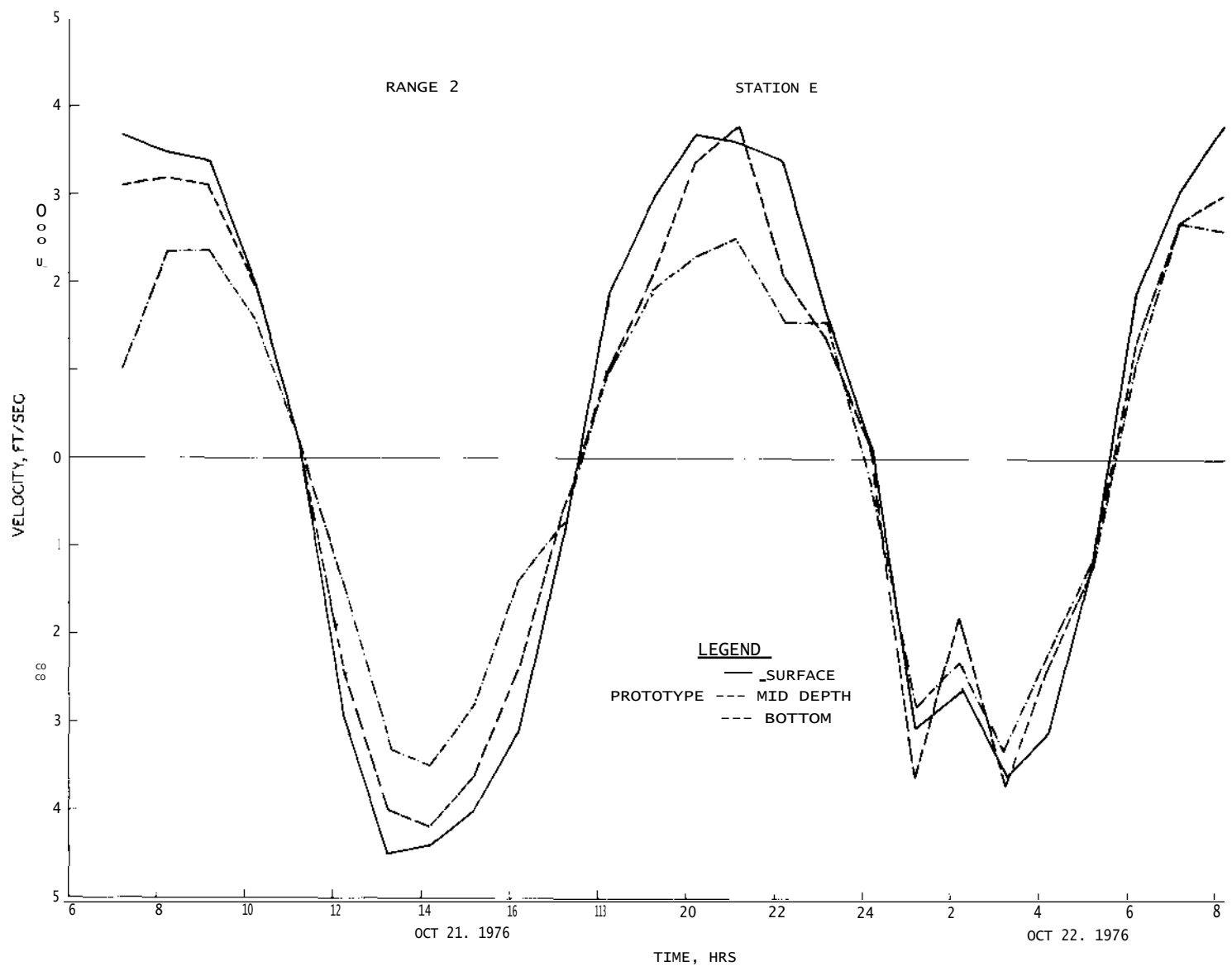
Figure 9. Example of the vertical variation in prototype current measurements
