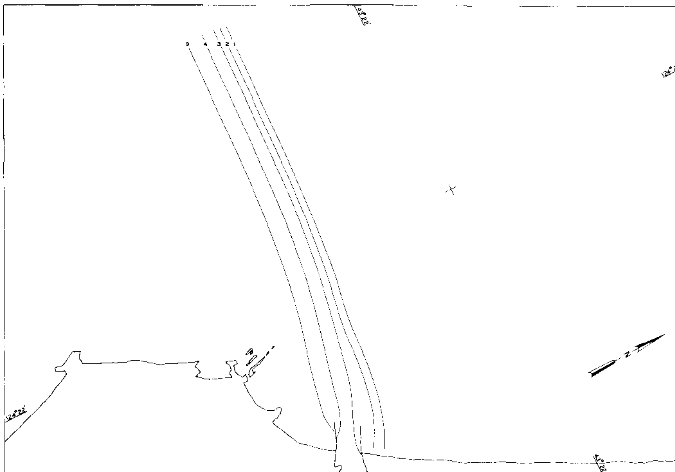
COOS BAY HARBOR WAVE REFRACTION DEEPWATER GRID WAVE PERIOD 120 SECONDS DEEPWATER AZIMUTH 2700 DEGREES
