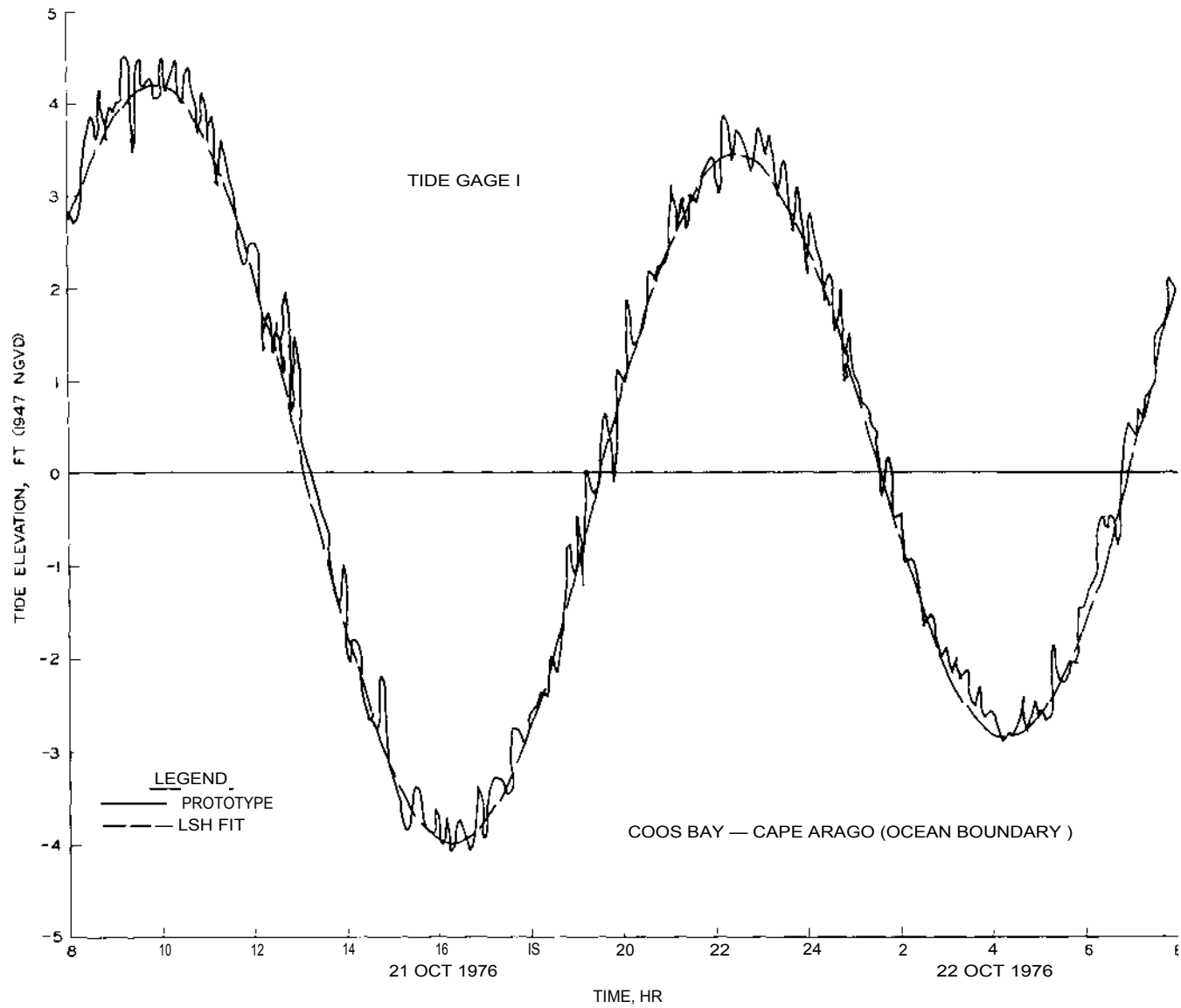
Figure 7. Least-squares harmonic fit to Cape Arago tide data
