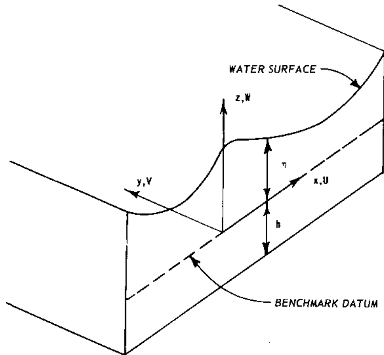
Figure 2. Coordinate system for problem formulation
