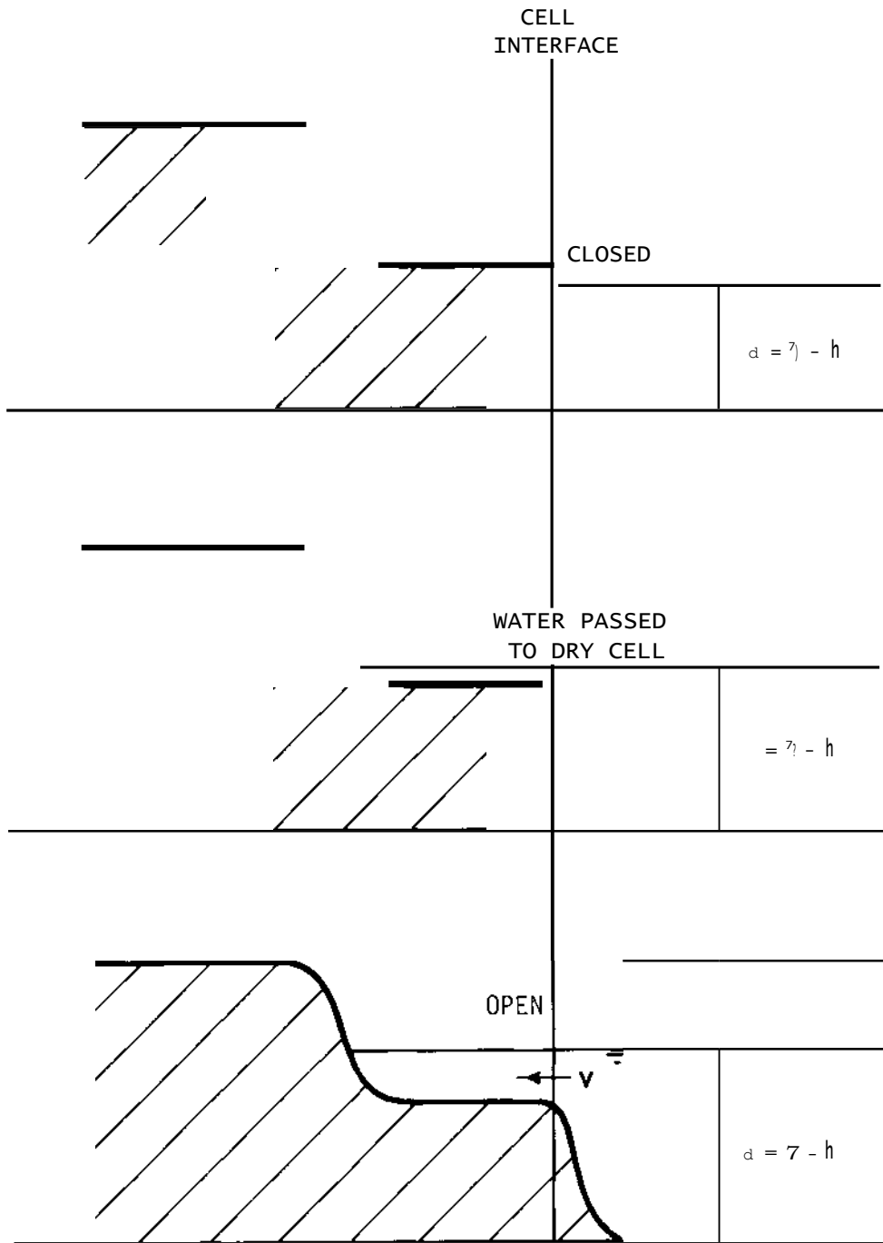
Figure 4. Flood cell treatment
