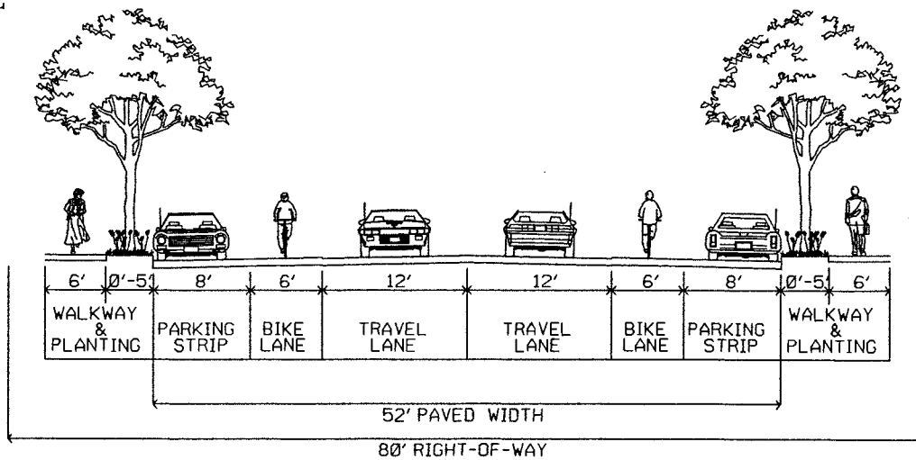
FIGURE 7-1 STREET STANDARDS
