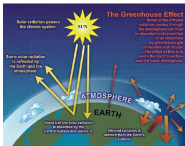
Figure 1-1. Greenhouse Effect
