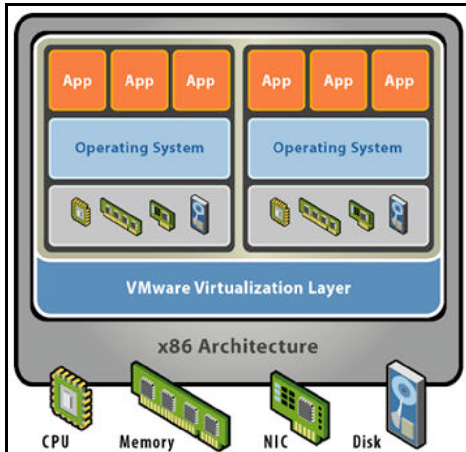
Figure 1: Virtualization Layers
