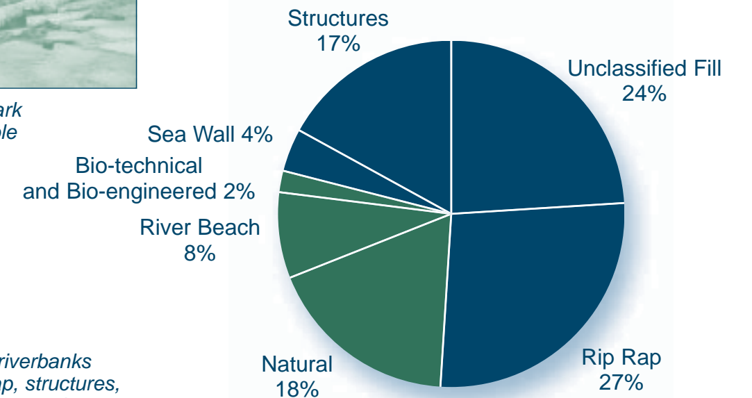
FIGURE 3: Existing Willamette Riverbank Composition
